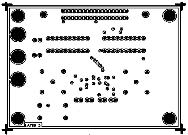
b. FSPCB Power Plane
