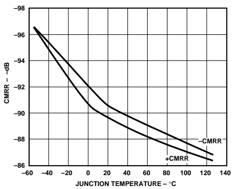
Figure 50. AD9631/AD9632 CMRR vs. Temperature
