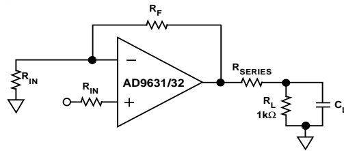
Figure 60. Driving Capacitive Loads
