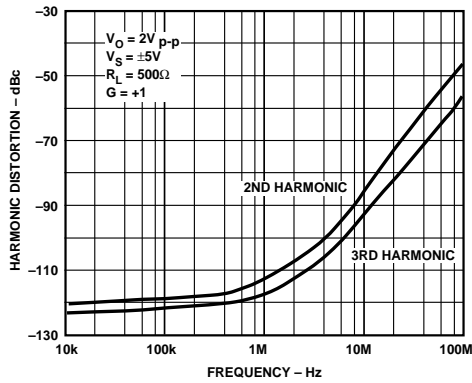
Figure 21. AD9631 Harmonic Distortion vs. Frequency, R_L = 500 \Omega
