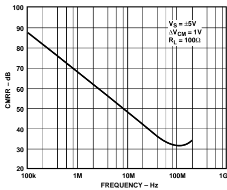
Figure 41. AD9631 CMRR vs. Frequency
