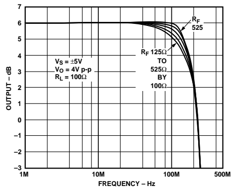
Figure 31. AD9632 Large Signal Frequency Response, G = +2
