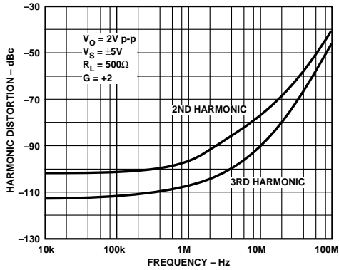
Figure 33. AD9632 Harmonic Distortion vs. Frequency, R_L = 500 \Omega
