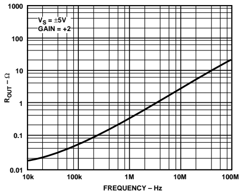
Figure 46. AD9632 Output Resistance vs. Frequency
