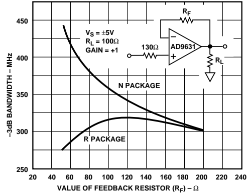
Figure 18. AD9631 Small Signal -3 dB Bandwidth vs. R_F
