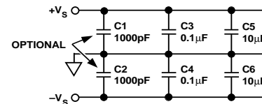
Supply Bypassing
