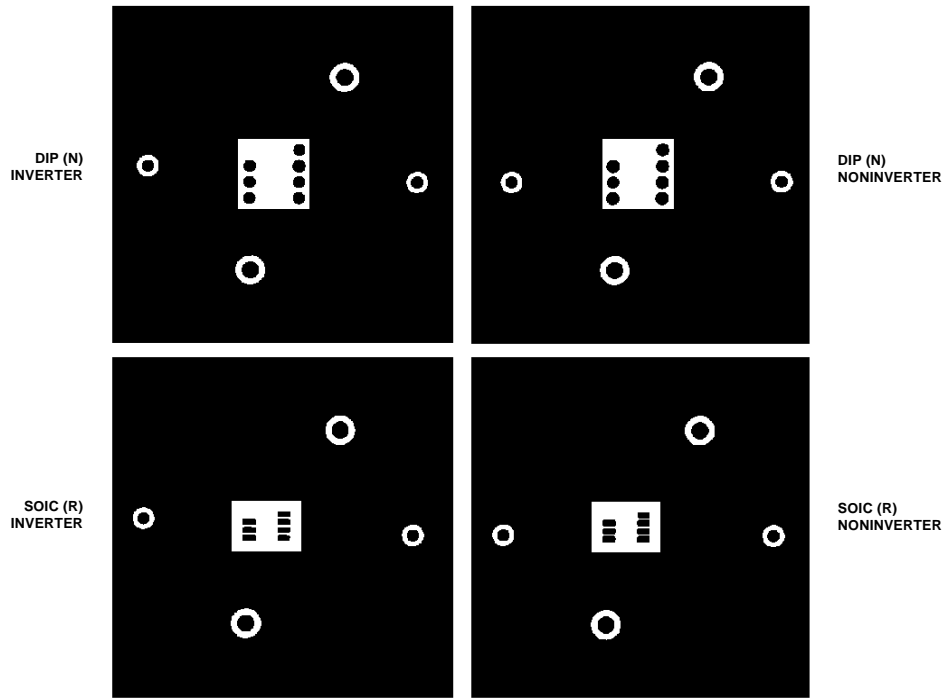
Figure 68. Board Layout (Component Side)
