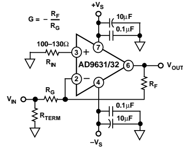
Figure 58. Inverting Operation
