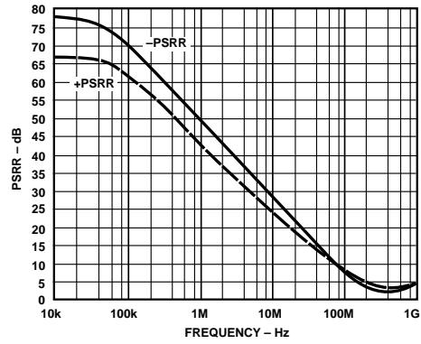
Figure 43. AD9632 PSRR vs. Frequency
