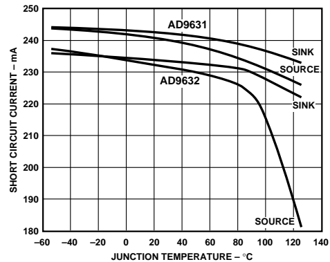
Figure 54. Short Circuit Current vs. Temperature
