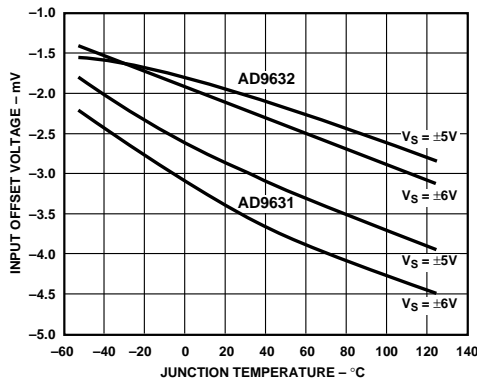
Figure 52. Input Offset Voltage vs. Temperature
