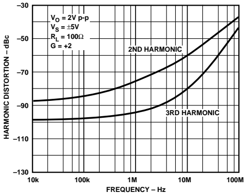
Figure 34. AD9632 Harmonic Distortion vs. Frequency, R_L = 100 \Omega
