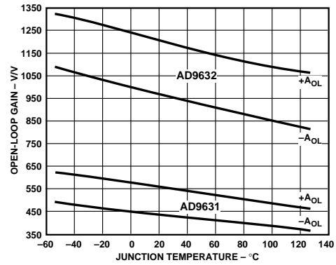
Figure 48. Open-Loop Gain vs. Temperature
