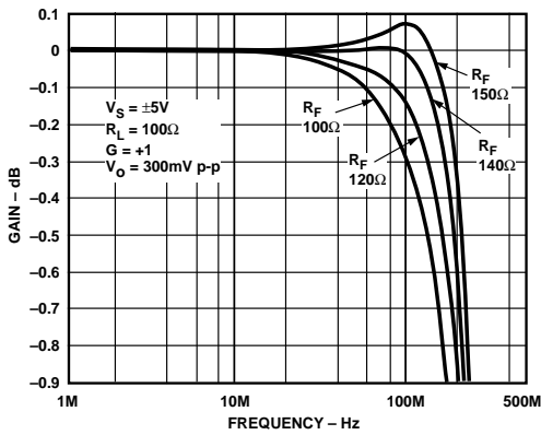
Figure 16. AD9631 0.1 dB Flatness, N Package (for R Package Add 20 Ω to R_F )
