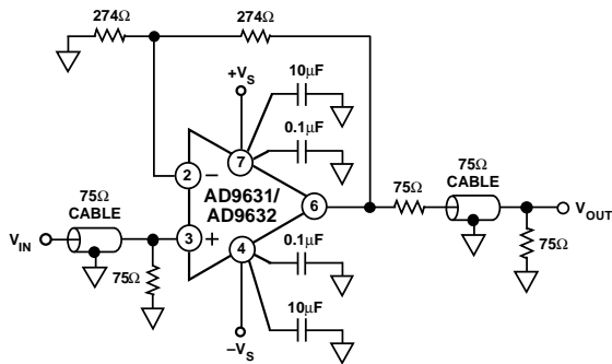
Figure 62. Video Line Driver
