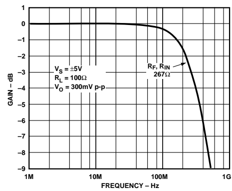
Figure 32. AD9632 Small Signal Frequency Response, G = -1
