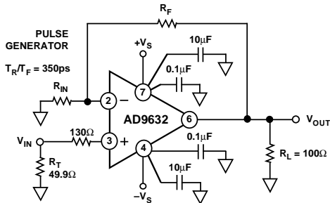
Figure 9. Noninverting Configuration, G = +2
