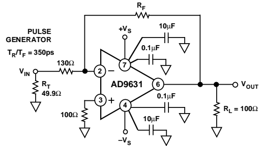
Figure 6. Inverting Configuration, G = -1
