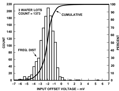
Figure 53. AD9631 Input Offset Voltage Distribution
