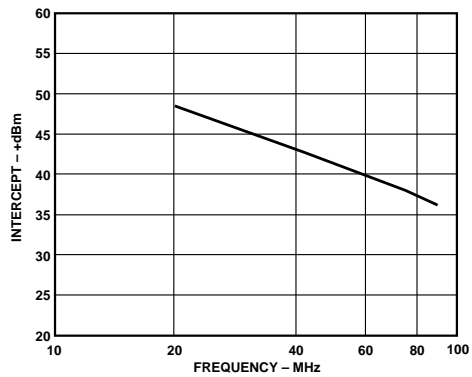
Figure 23. AD9631 Third Order Intercept vs. Frequency
