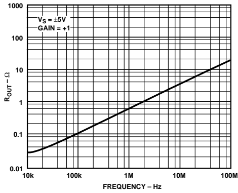
Figure 45. AD9631 Output Resistance vs. Frequency
