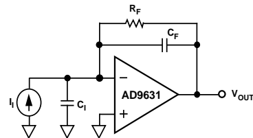
Figure 59. Transimpedance Configuration
