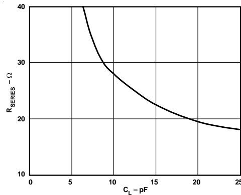
Figure 61. Recommended R_{SERIES} vs. Capacitive Load
