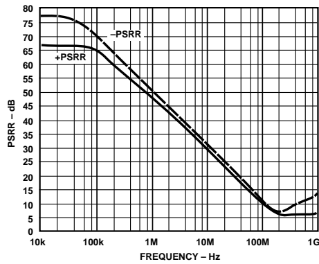
Figure 40. AD9631 PSRR vs. Frequency
