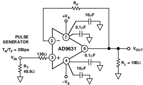
Figure 3. Noninverting Configuration, G = +1
