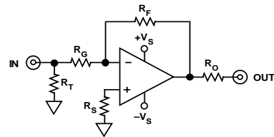
Inverting Configuration
