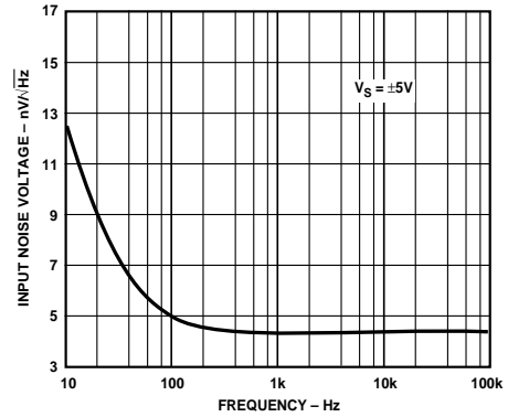
Figure 42. AD9632 Noise vs. Frequency
