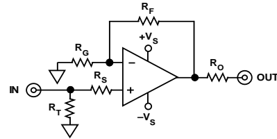
Noninverting Configuration
