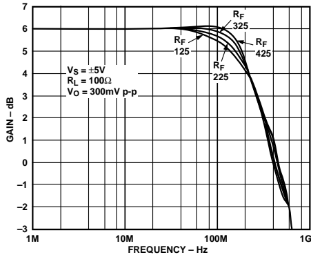
Figure 27. AD9632 Small Signal Frequency Response, G = +2
