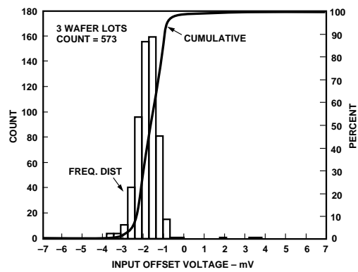
Figure 56. AD9632 Input Offset Voltage Distribution
