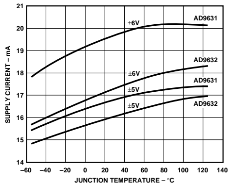
Figure 51. Supply Current vs. Temperature
