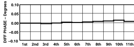
Figure 24. AD9631 Differential Gain and Phase Error, G = +2 , R_L = 150 \Omega
