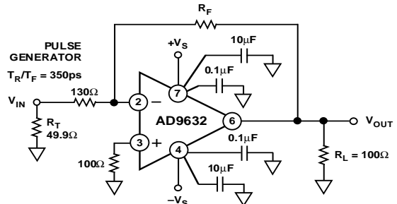
Figure 12. Inverting Configuration, G = -1
