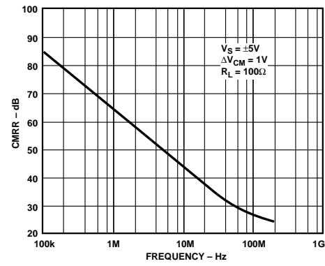
Figure 44. AD9632 CMRR vs. Frequency
