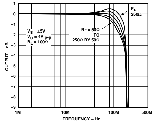
Figure 19. AD9631 Large Signal Frequency Response, G = +1
