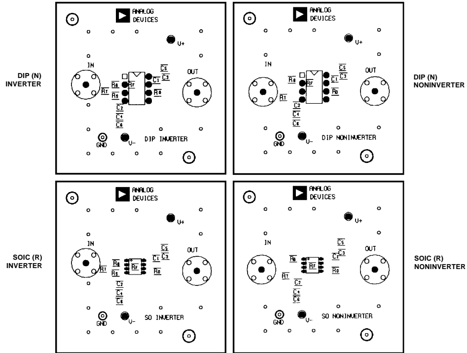
Figure 66. Evaluation Board Silkscreen (Top)
