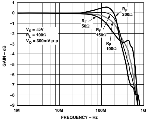
Figure 15. AD9631 Small Signal Frequency Response G = +1
