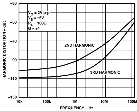
Figure 22. AD9631 Harmonic Distortion vs. Frequency, R_L = 100 \Omega
