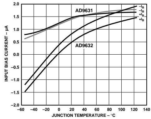
Figure 55. Input Bias Current vs. Temperature
