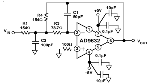
Figure 63. Active Filter Circuit
