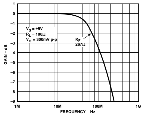
Figure 20. AD9631 Small Signal Frequency Response, G = -1
