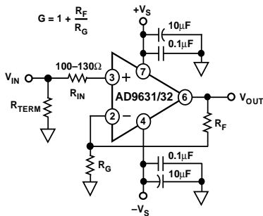
Figure 57. Noninverting Operation
