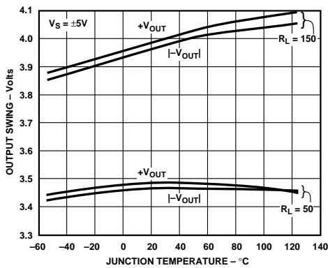
Figure 47. AD9631/AD9632 Output Swing vs. Temperature
