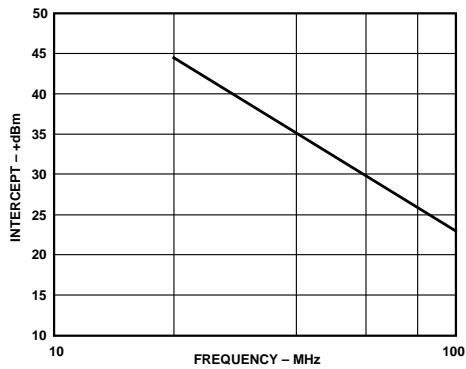
Figure 35. AD9632 Third Order Intercept vs. Frequency
