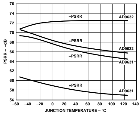
Figure 49. PSRR vs. Temperature
