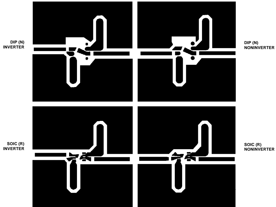
Figure 67. Board Layout (Solder Side)
