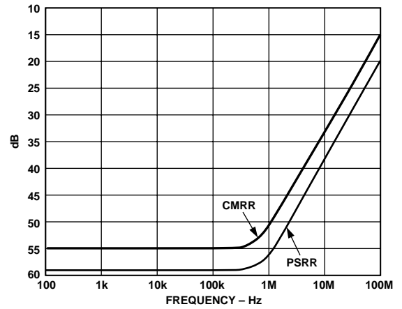
Figure 4. CMRR and PSRR
