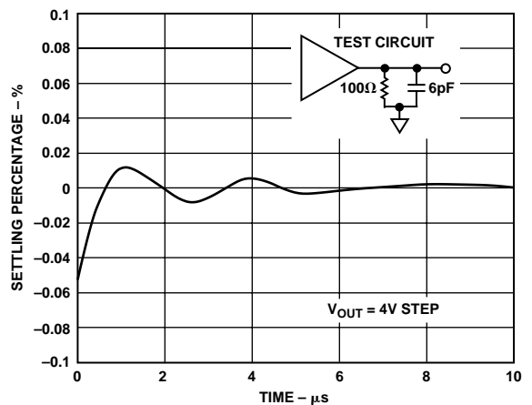
Figure 6. Long Term Settling Time
