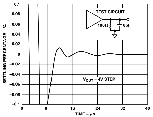
Figure 5. Settling Time
