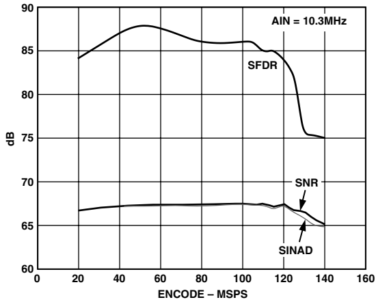
Figure 7. SNR/SINAD/SFDR vs. f_s : f_{IN} = 10.3 \text{ MHz}
