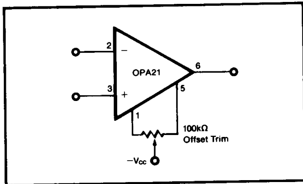
FIGURE 1. Voltage Offset Trim.
