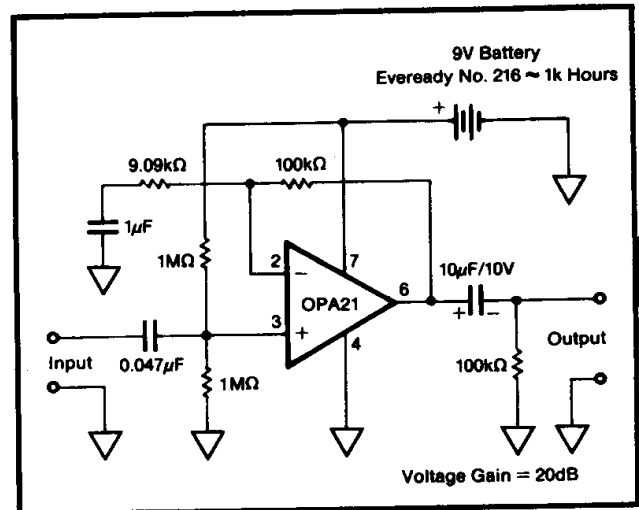
FIGURE 4. AC Amplifier.
