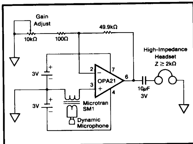
FIGURE 3. Portable Microphone Amplifier.
