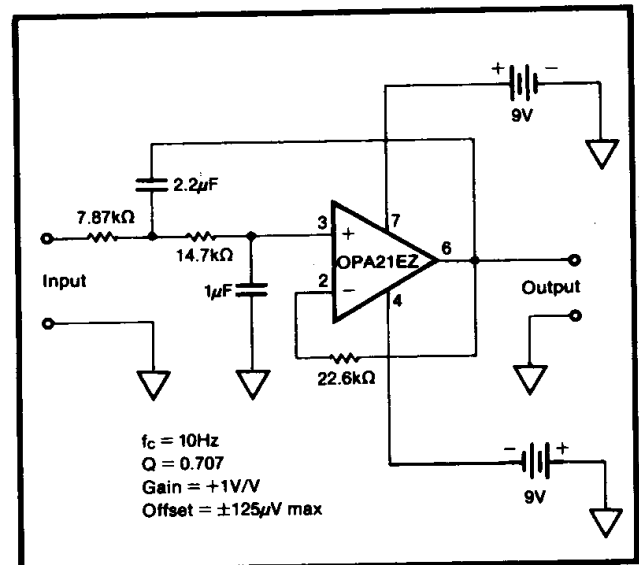
FIGURE 5. Second-Order 10Hz Low-Pass Filter.
