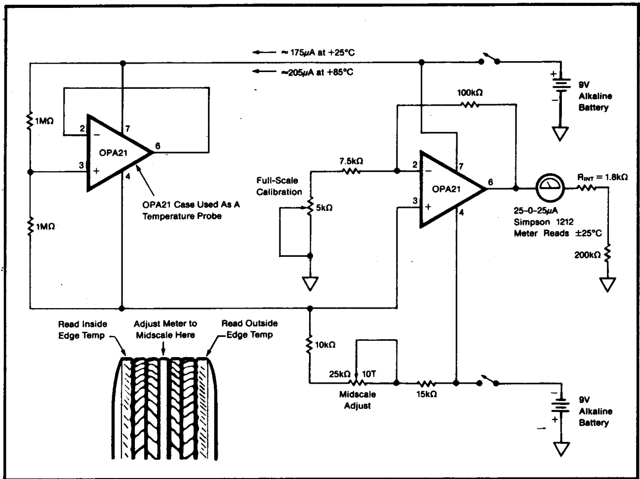
FIGURE 6. Portable Tire Pyrometer.
