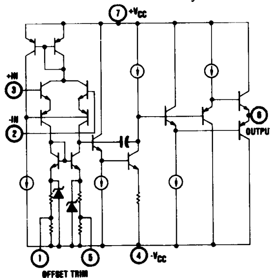
SIMPLIFIED CIRCUIT
