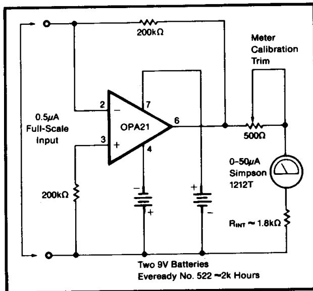
FIGURE 2. Fully-Floating Current Meter.
