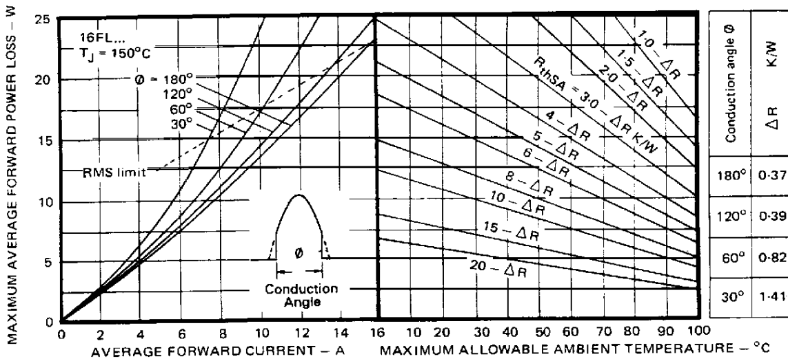
Fig. 9 – Current Rating Nomogram (Sinusoidal Waveforms), 16FL Series
