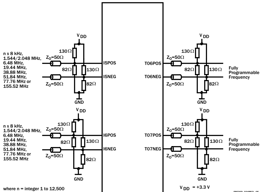
Figure 23 Recommended Line Termination for PECL Input/Output Ports
