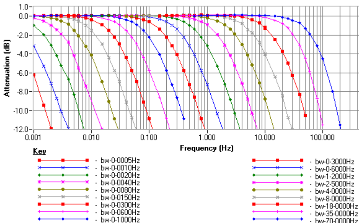
Figure 8 TO DPLL Wander and Jitter Measured Transfer Characteristics (Jitter = 0.2 UI pk-pk)
