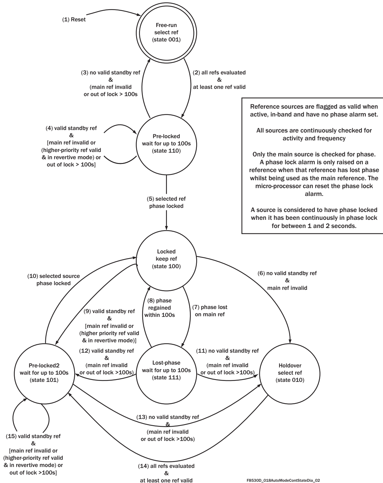
Figure 5 Automatic Mode Control State Diagram
