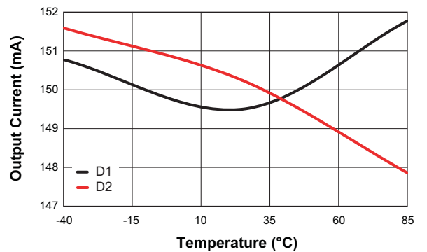
Flash Current Matching vs. Temperature (V IN = 3.6V; 150mA/Channel)
