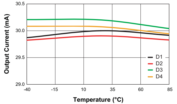
Backlight Current Matching vs. Temperature (V IN = 3.6V; 30mA/Channel)
