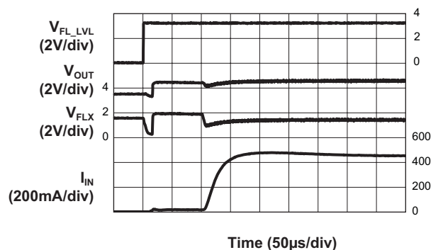
Flash Mode Turn-On Characteristic ( V_{IN} = 3.6V ; 300mA/Channel; 1.5x Mode)
