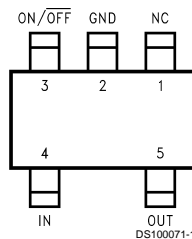
Top View SOT-23 Package 5-Lead, Molded-Plastic Small-Outline Transistor (SOT) Package Package Code MA05B(Notes 1)
