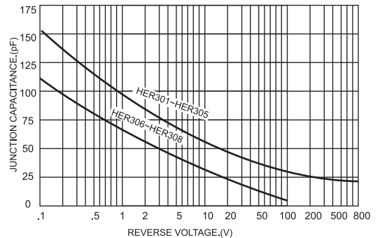
FIG.6-TYPICAL JUNCTION CHARACTERISTICS
