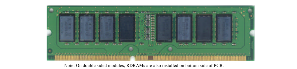
Figure 1 : 32 bit RIMM module with heat spreader removed
