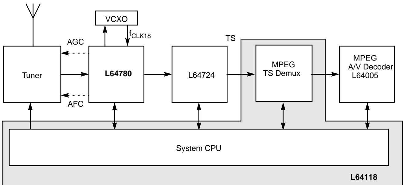
Figure 1.1 Typical Terrestrial-Only Receiver
