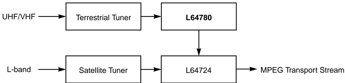
Figure 1.3 Receiver Architecture for Satellite and Terrestrial Reception
