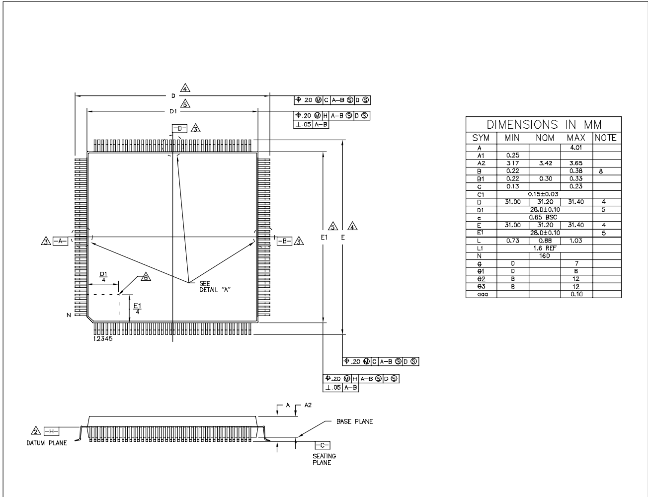
Figure 6.5 160 PQFP Mechanical Drawing: Top and Side Views
