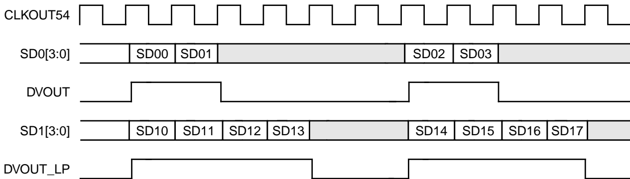
Figure 3.11 Hierarchical, Two FEC Decoders, 64 QAM Constellation
