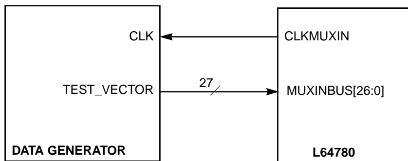
Figure 3.15 MUXIN Signals Interface
