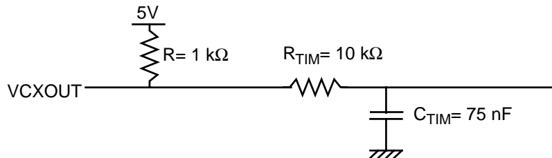
Figure 2.4 External Low-Pass Loop Filter
