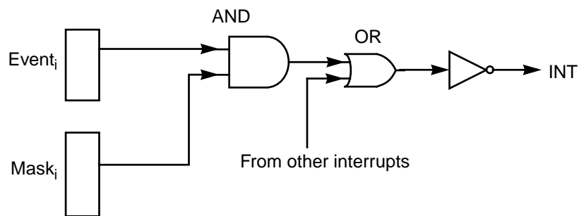
Figure 4.4 Interrupt Generation
