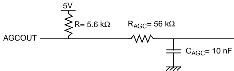
Figure 2.3 AGC Loop Pass Filter
