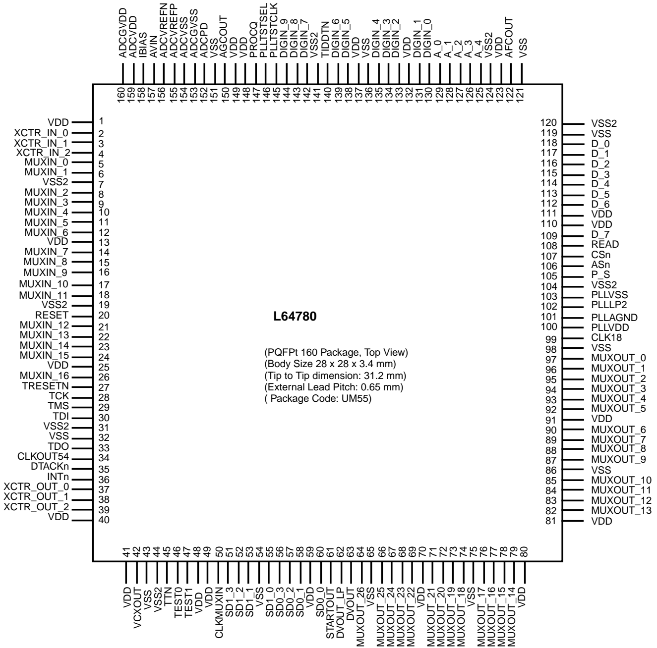
Figure 6.4 Package Pin Layout
