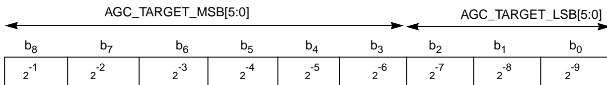
Figure 2.2 Structure of 9-Bit AGC_TARGET Register
