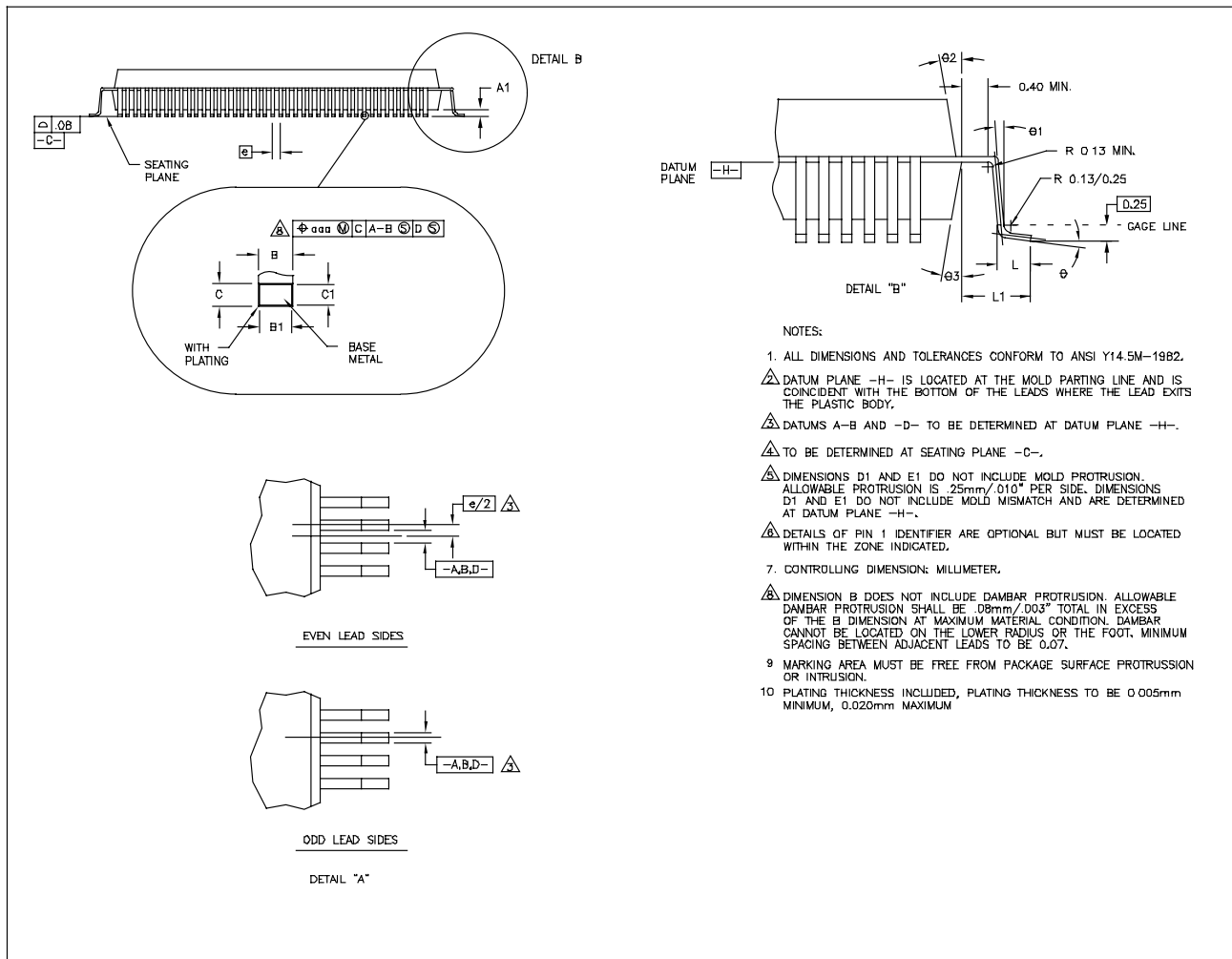
Figure 6.6 160 PQFP Mechanical Drawing: Detail
