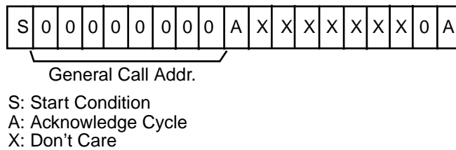
Figure A.2 General Call Address
