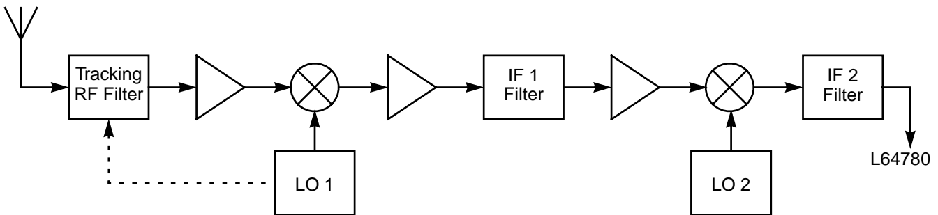
Figure 1.2 UHF Tuner Example
