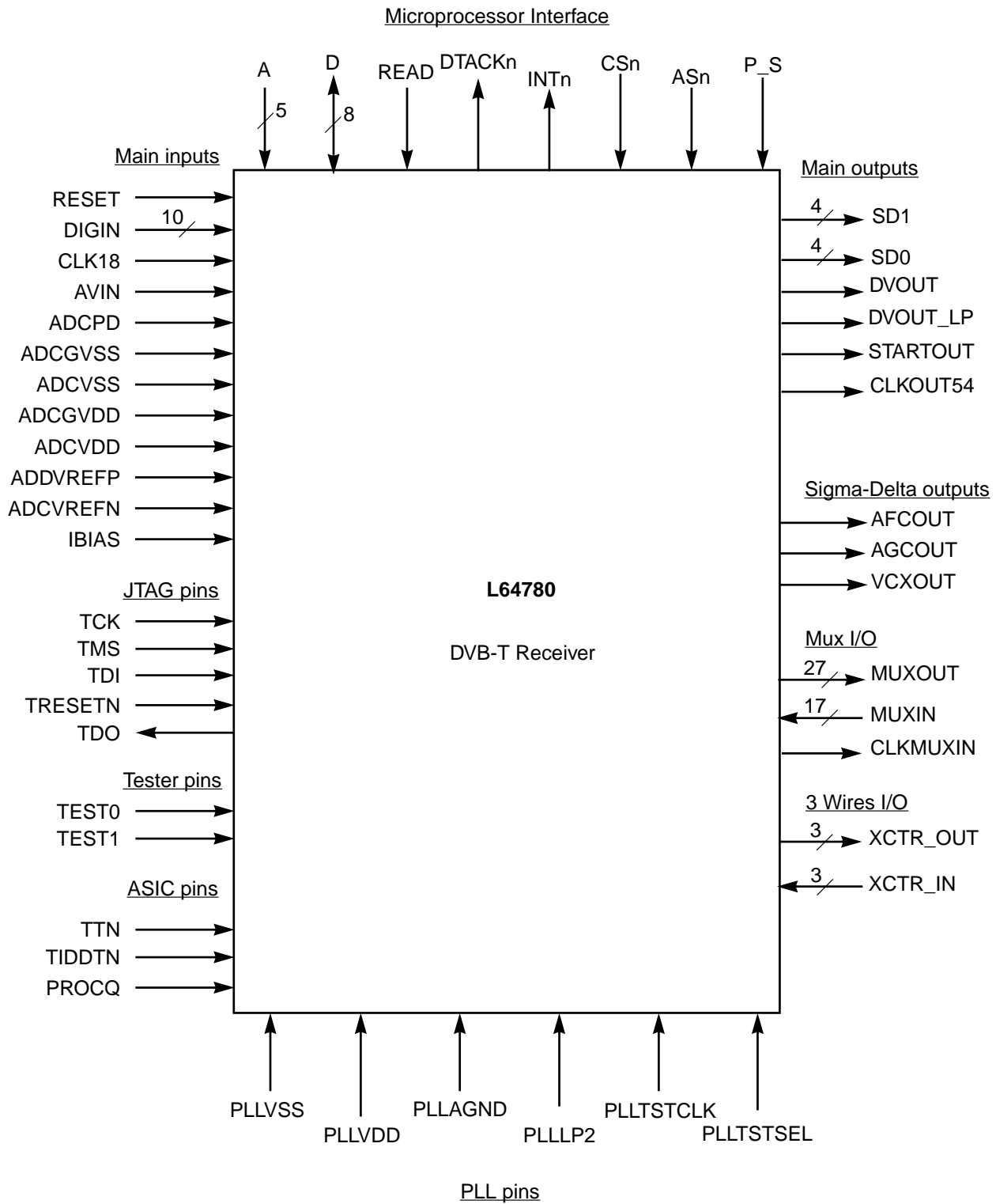
Figure 5.1 L64780 Logic Symbol
