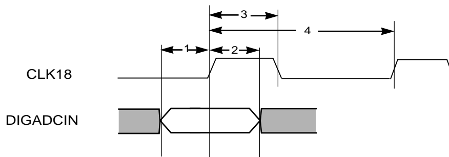
Figure 6.1 Input Data AC Timing
