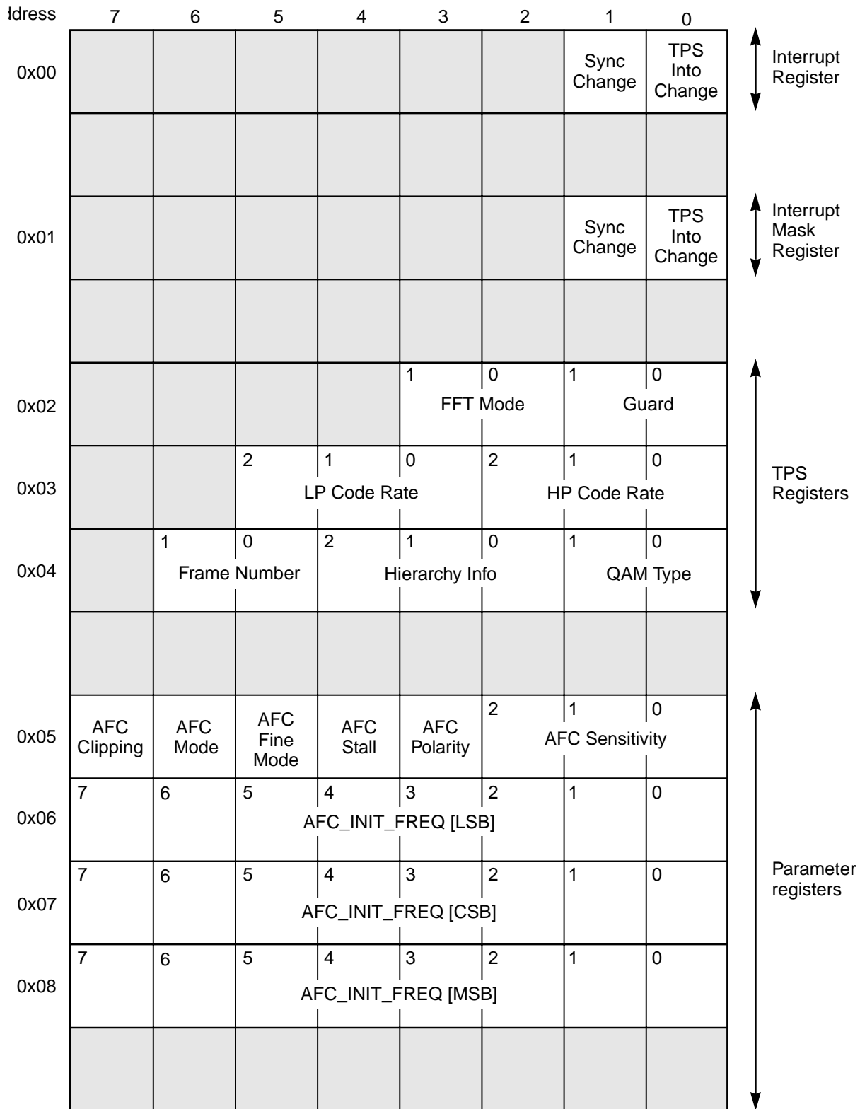
Figure 4.1 Graphical View of the L64780 Register Address Space 1
