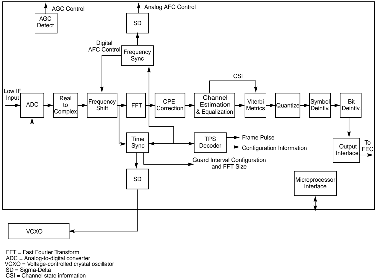
Figure 2.1 DTTV Demodulator Architecture
