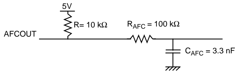
Figure 2.5 AFC Loop Pass Filter
