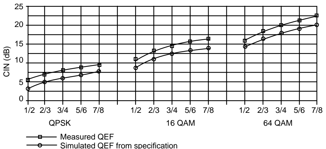
Figure 1.4 Performance with Additive White Gaussian Noise (AWGN)
