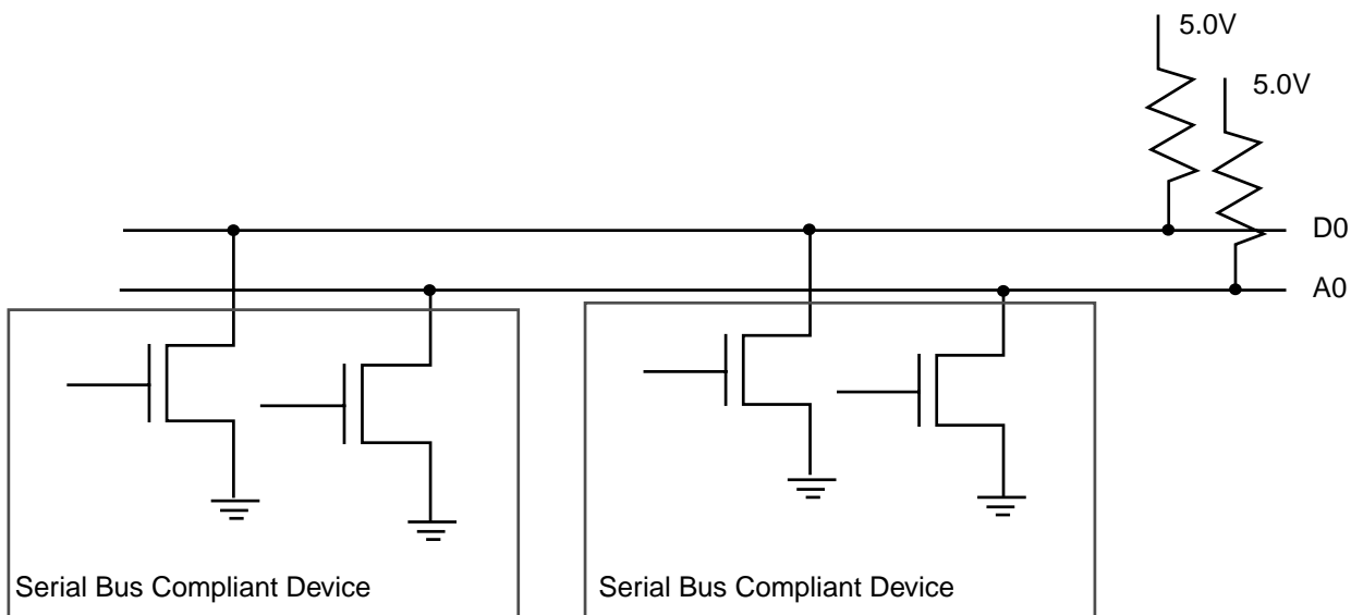
Figure A.1 Serial Bus Overview
