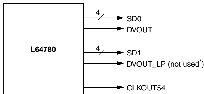
Figure 3.5 Output Interface in Nonhierarchical and Parallel Modes
