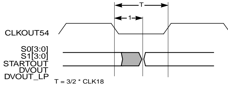
Figure 6.2 Output Data AC Timing
