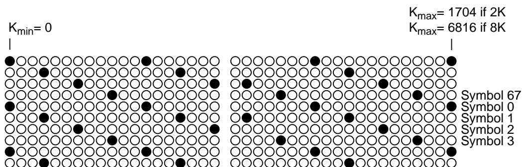
Figure 2.6 Scattered Pilot Structure
