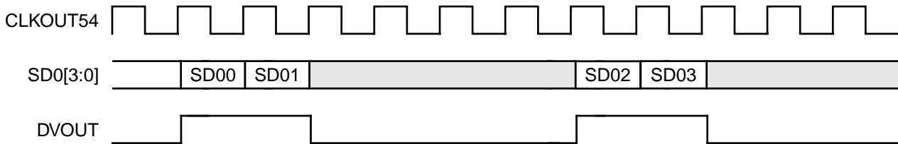
Figure 3.13 Hierarchical, One FEC Decoder Mode With 16 QAM (HP or LP Selected) or 64 QAM (LP Selected only)
