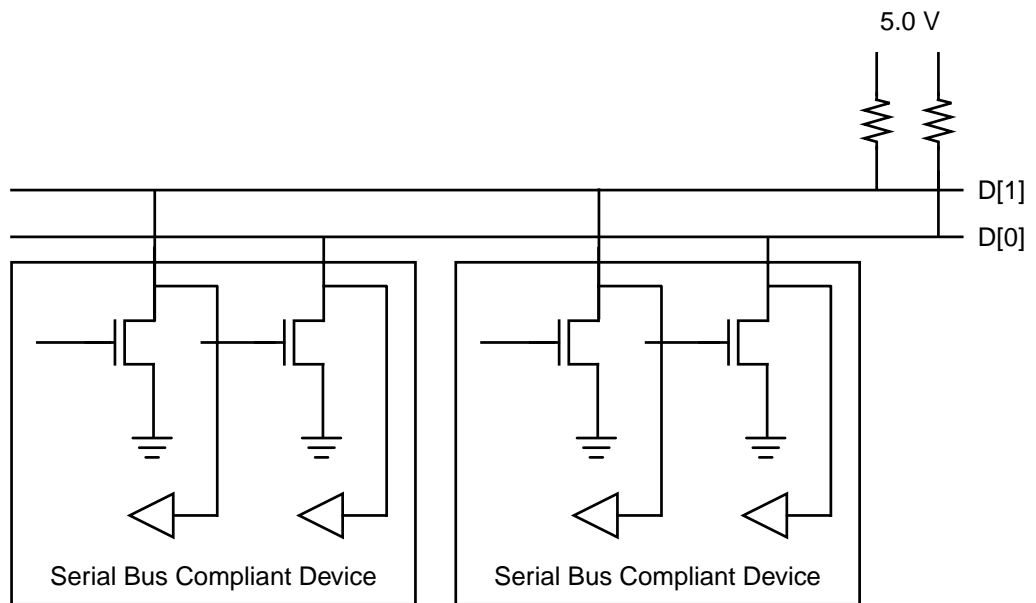
Figure A.1 Serial Bus Architecture
