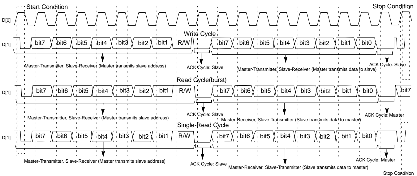
Figure A.3 Serial Bus Write/Read Cycle Overview
