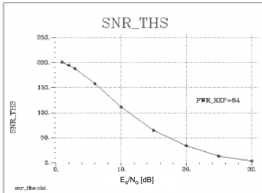
Figure 5.7 SNR Threshold vs. E_s/N_o
