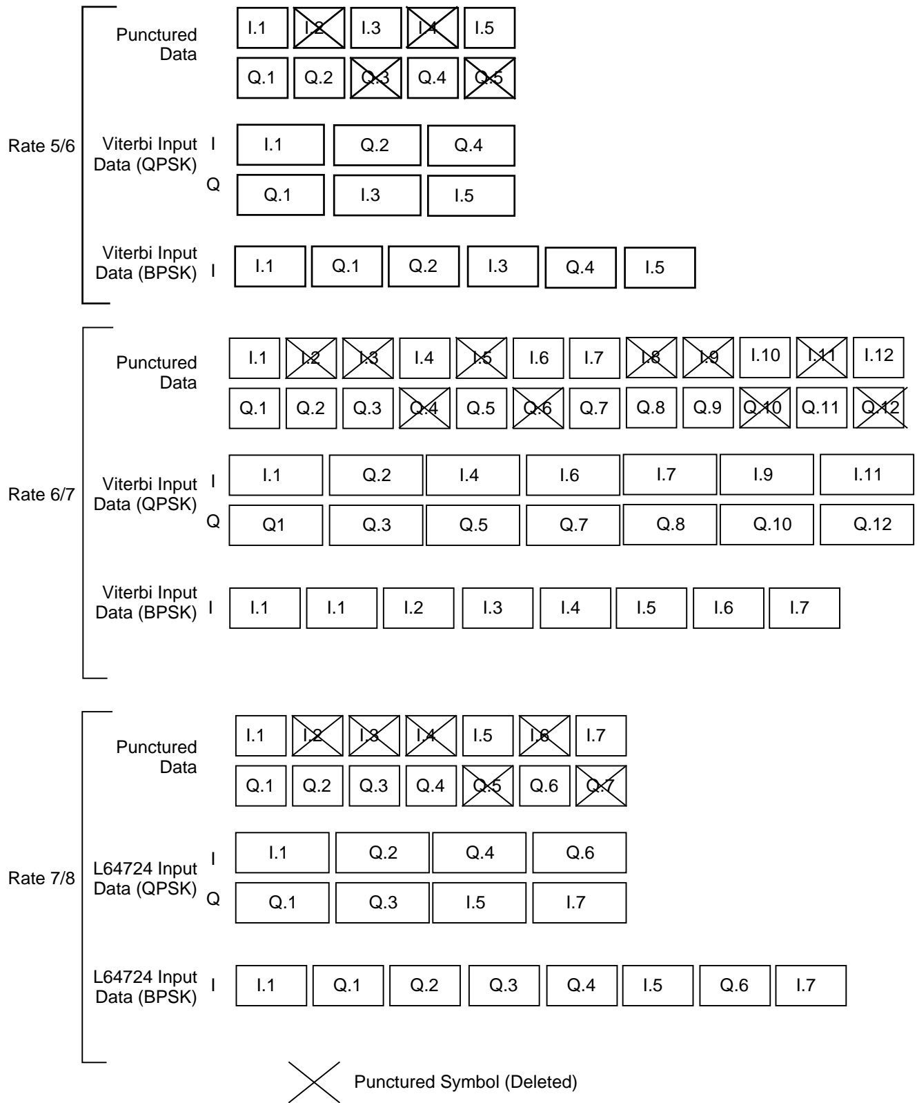
Figure 7.3 Puncture Pattern for Different Code Rates (Cont.)
