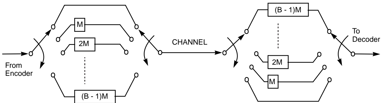
Figure 7.5 Interleaving/Deinterleaving Operation for DVB
