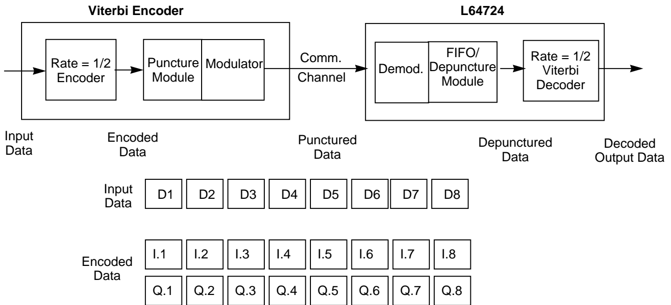
Figure 7.2 Puncturing and Depuncturing Block Diagram
