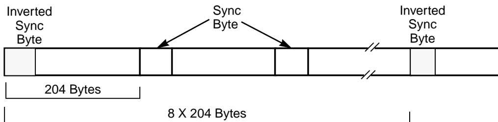
Figure 6.16 L64724 Transport Packet
