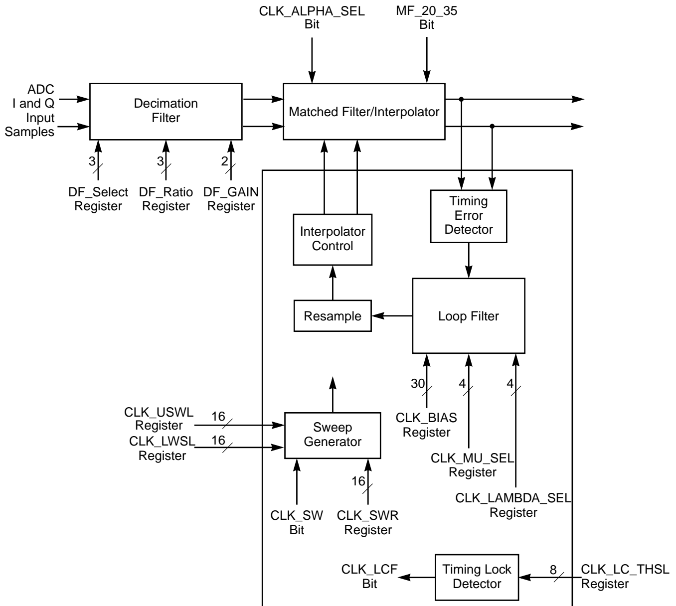
Figure 5.3 Clock Recovery Loop
