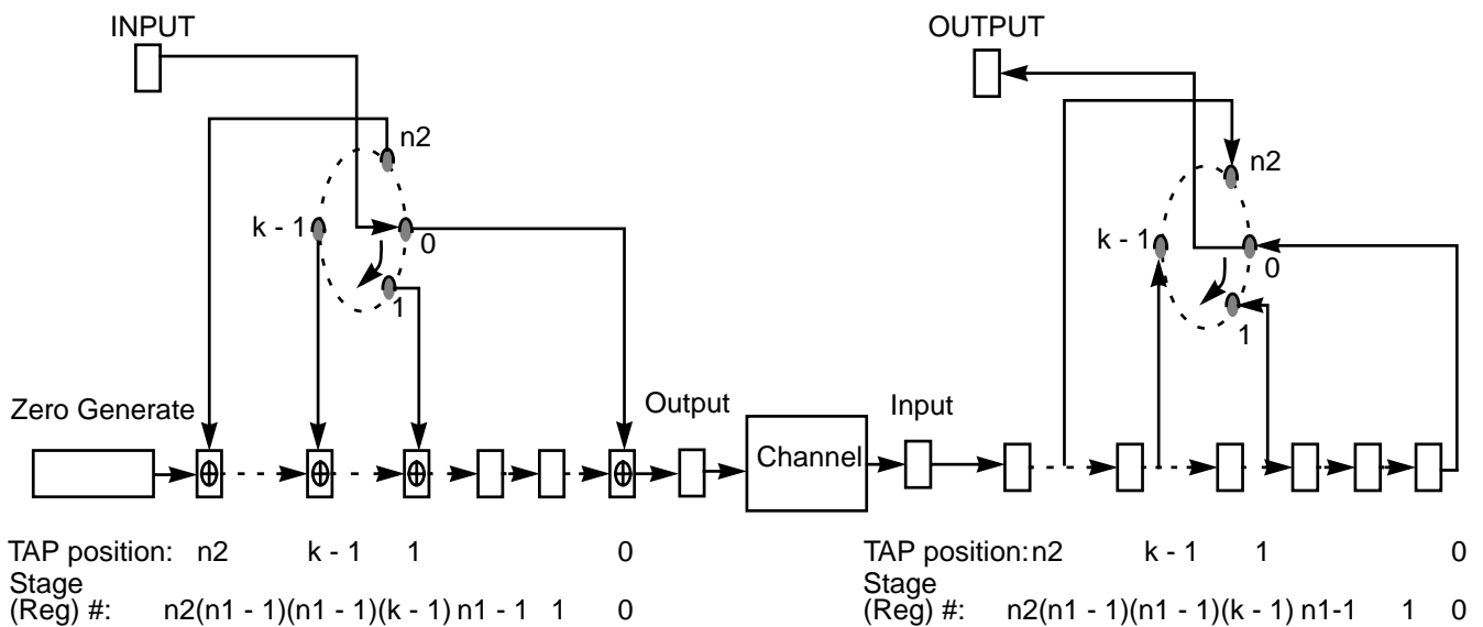
Figure 7.6 Interleaving/Deinterleaving Operation for DSS
