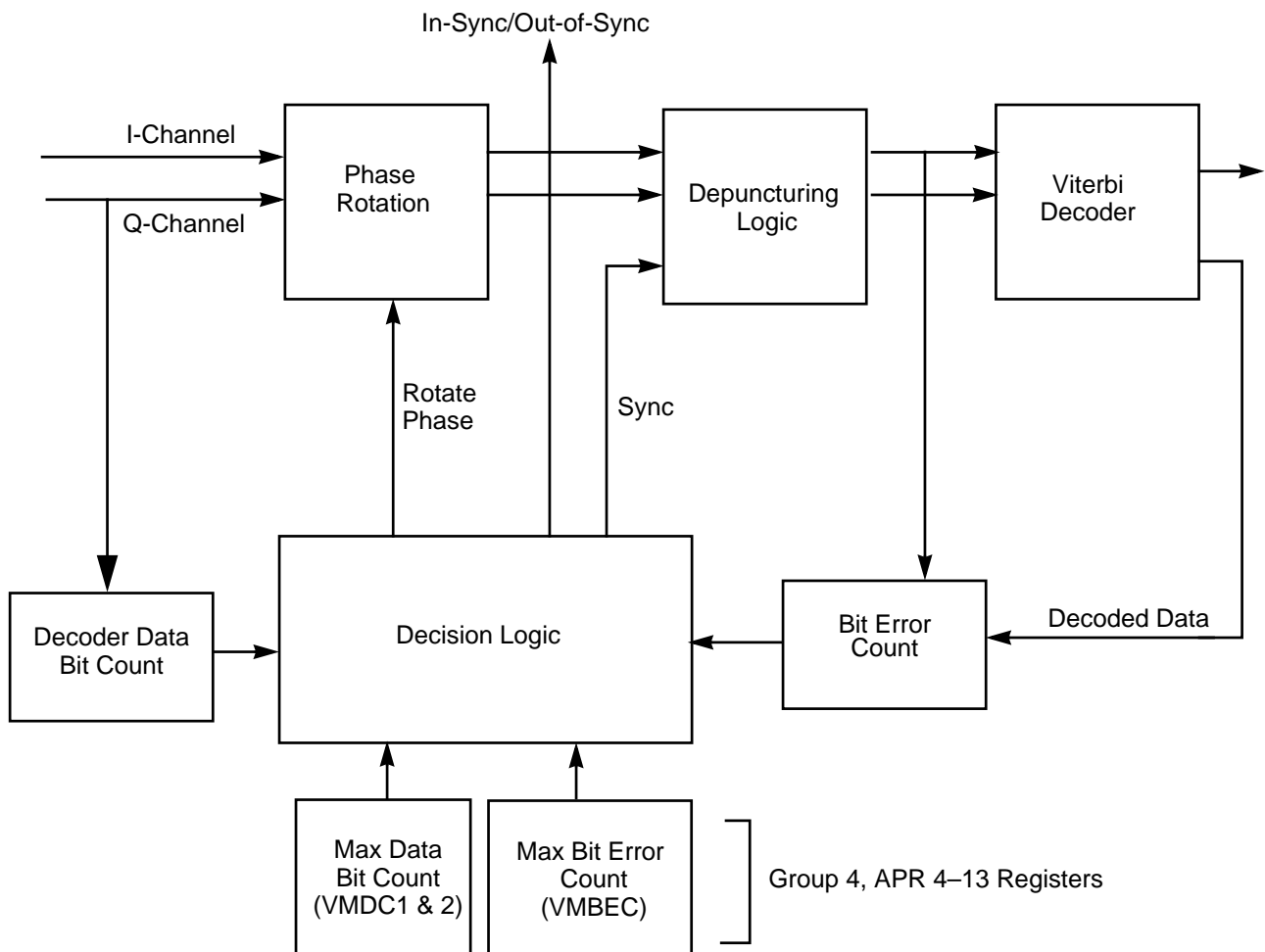
Figure 6.2 Viterbi Decoder Synchronization
