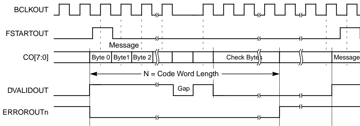
Figure 4.7 Descrambler Parallel Output Waveforms
