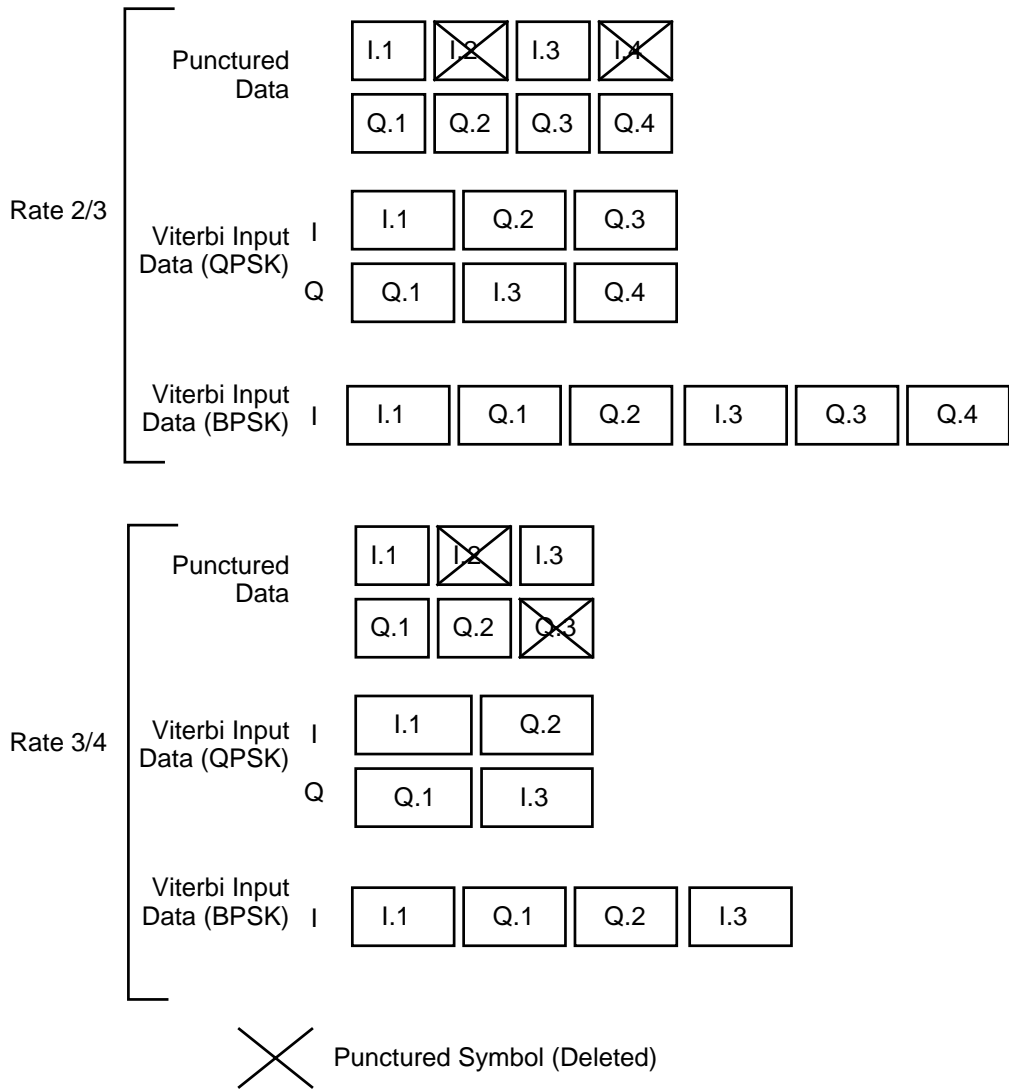
Figure 7.3 Puncture Pattern for Different Code Rates
