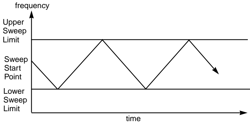
Figure 5.4 Timing Loop Sweep Operation
