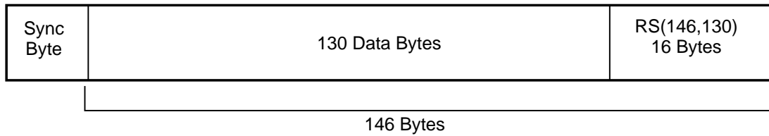
Figure 6.14 DSS Packet
