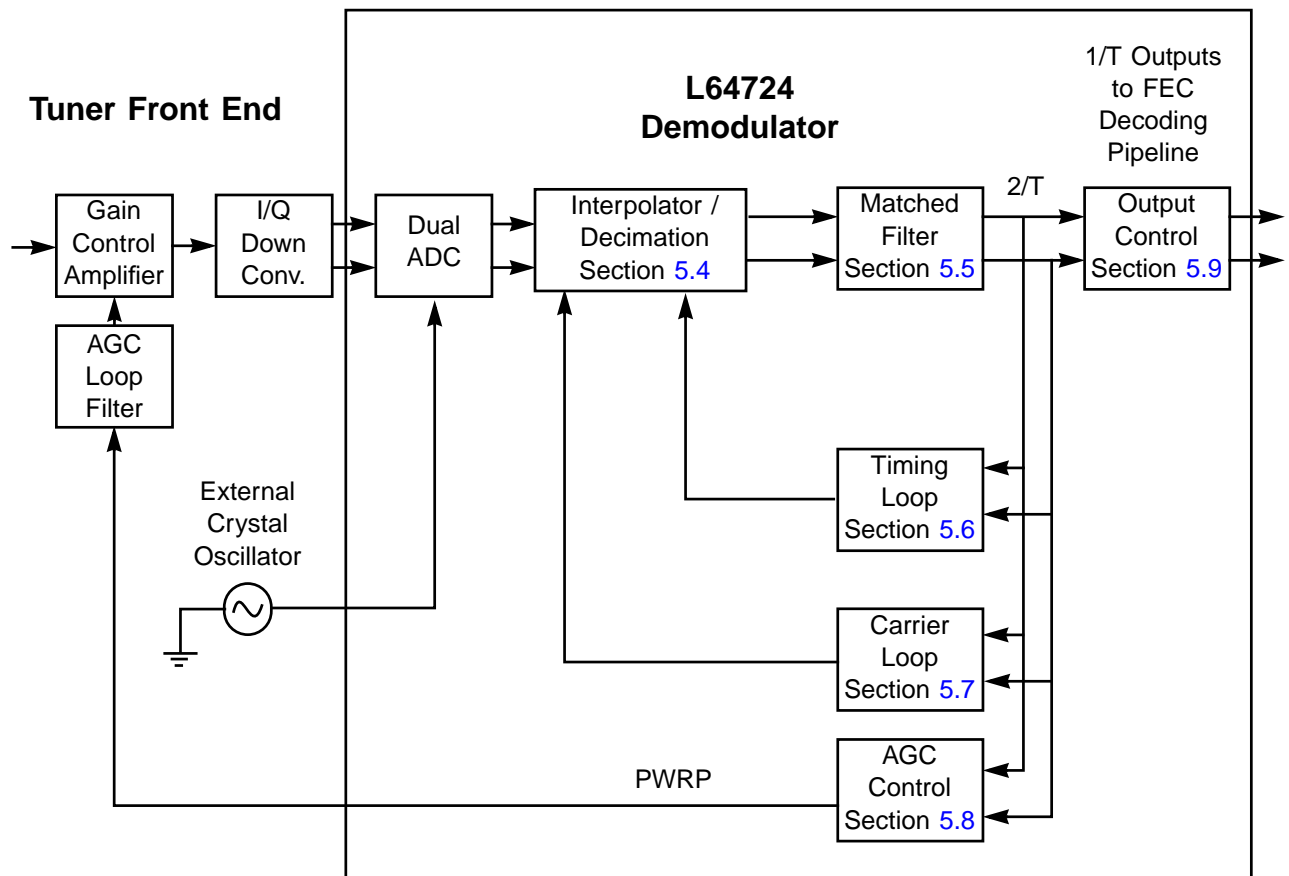
Figure 5.1 Demodulator Module and Associated Circuitry
