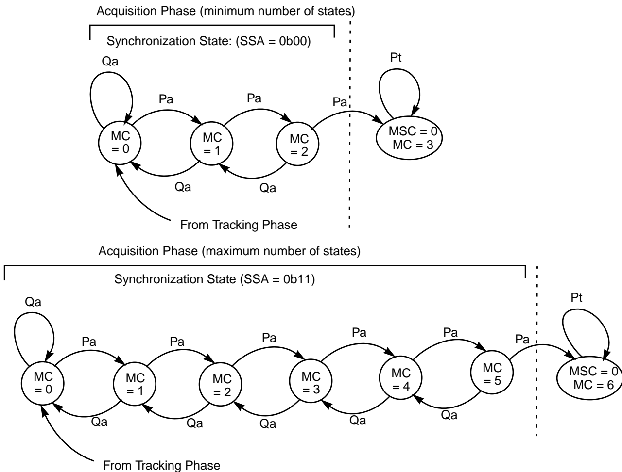
Figure 6.12 Minimum and Maximum Number of States in the Acquisition Phase
