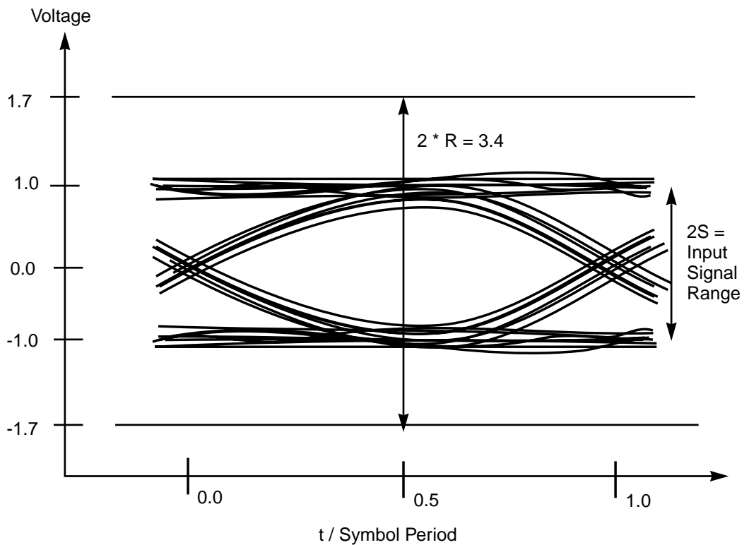
Figure 5.9 Eye Pattern and ADC Range
