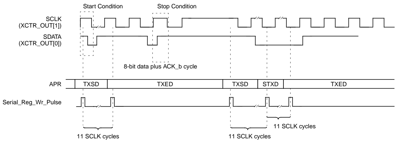
Figure C.1 2-Wire Compliant Interface
