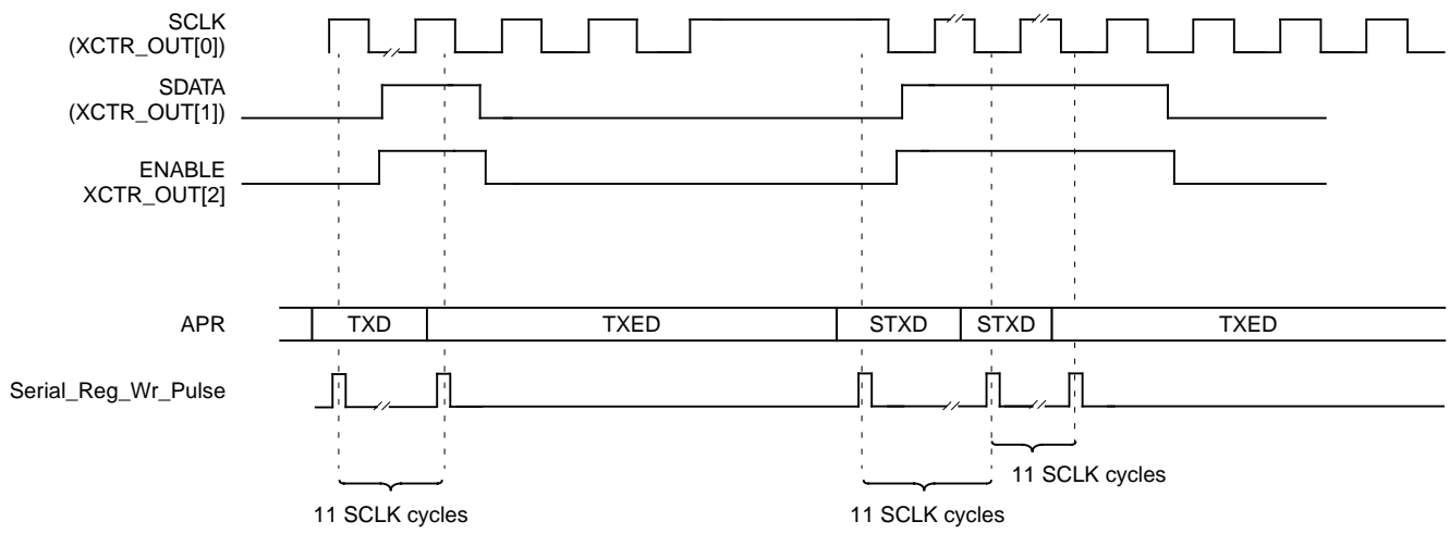
Figure C.2 3-Wire Interface
