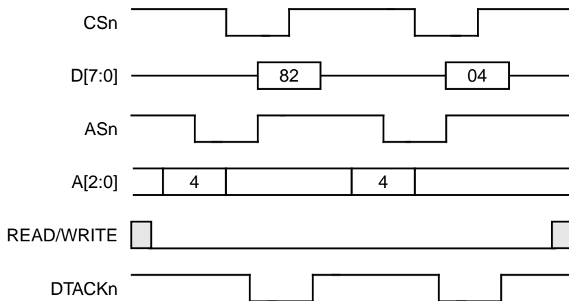
Figure 3.4 Write Locations 0 and 1 in Group 4
