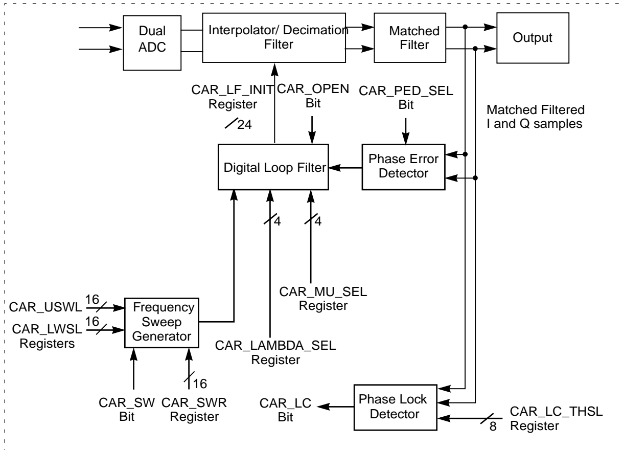
Figure 5.5 Carrier Recovery Loop
