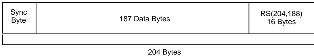
Figure 6.15 MPEG-2 Transport Packet
