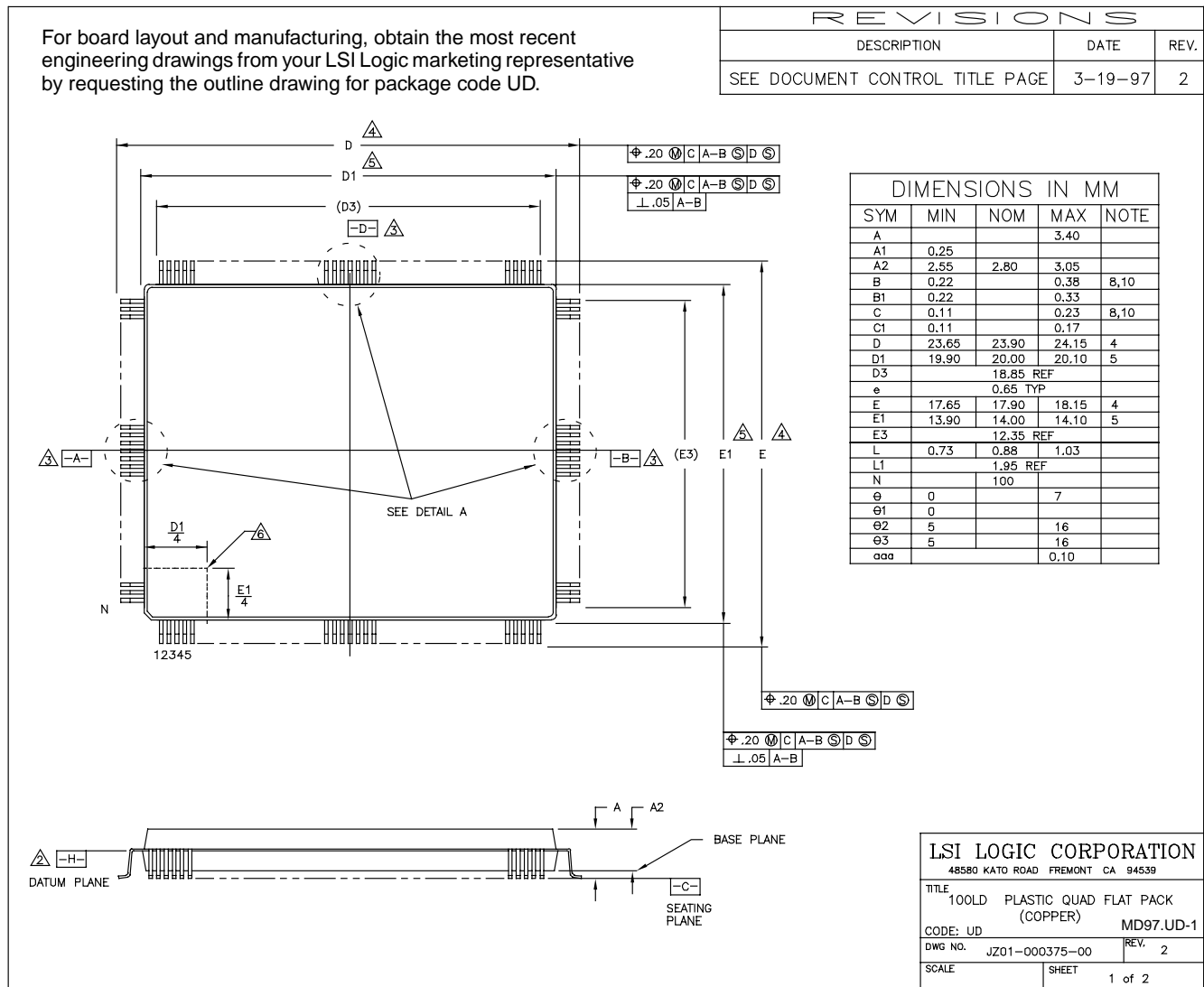
Figure 8.9 100-Pin PQFP/MQFP Mechanical Drawing
