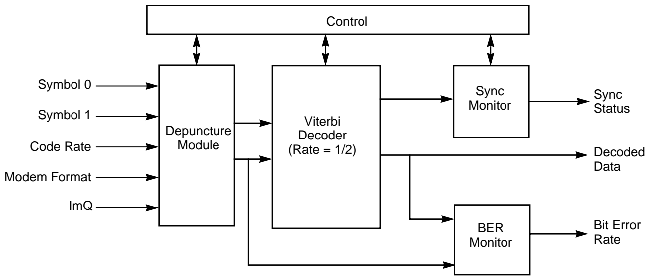
Figure 7.1 Viterbi Decoder Block Diagram
