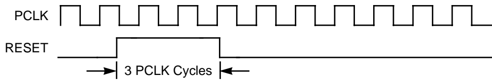
Figure 3.2 Issue a Hard Reset
