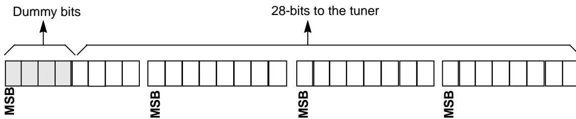
Figure C.3 28-Bit Write Using 3-Wire Mode
