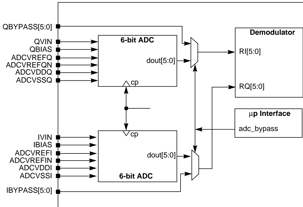
Figure D.1 ADC Connections for L64724
