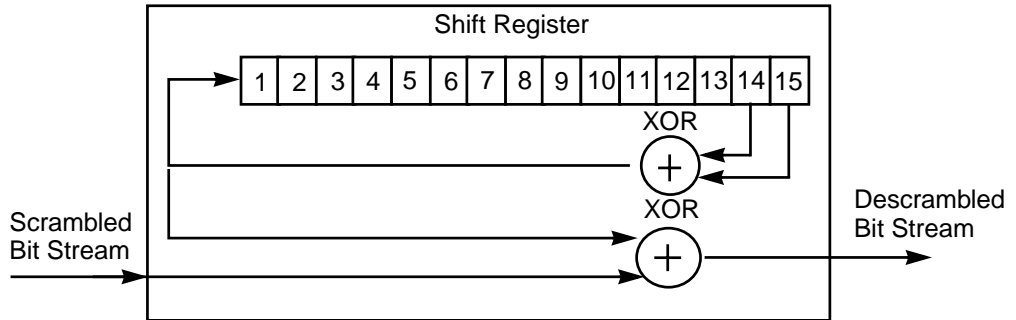
Figure 7.10 Descrambler Block Diagram
