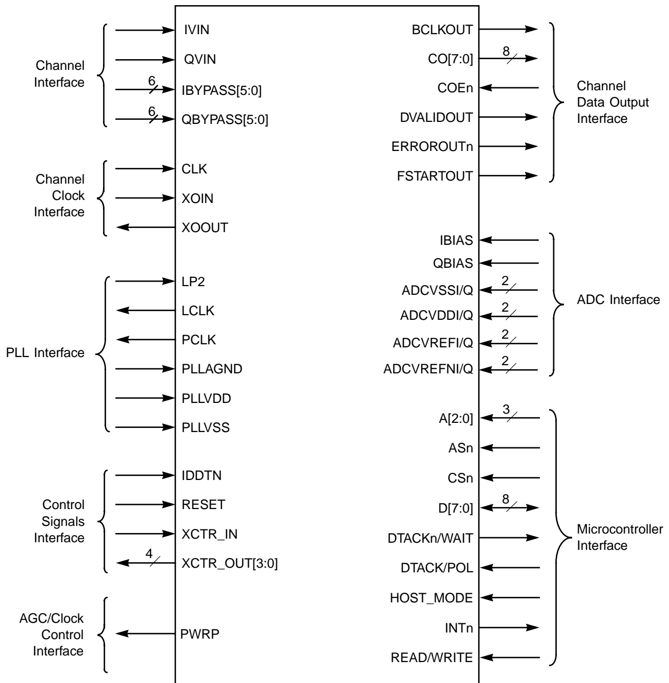
Figure 2.1 L64724 Logic Symbol
