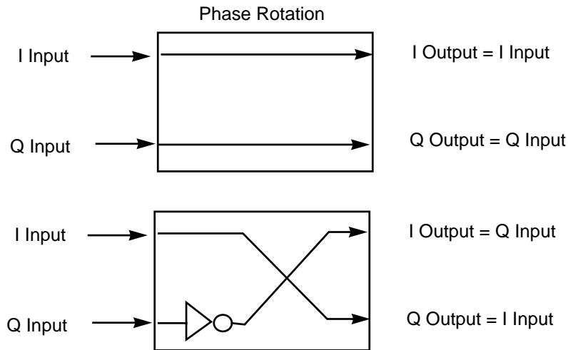
Figure 6.3 Phase Rotation for Synchronization
