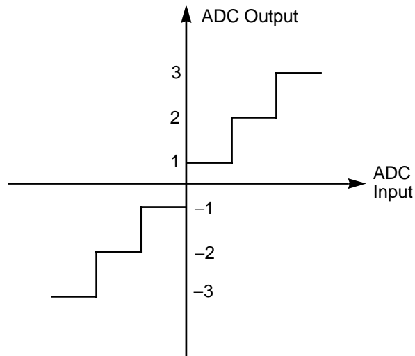
Figure 5.2 Input Quantization
