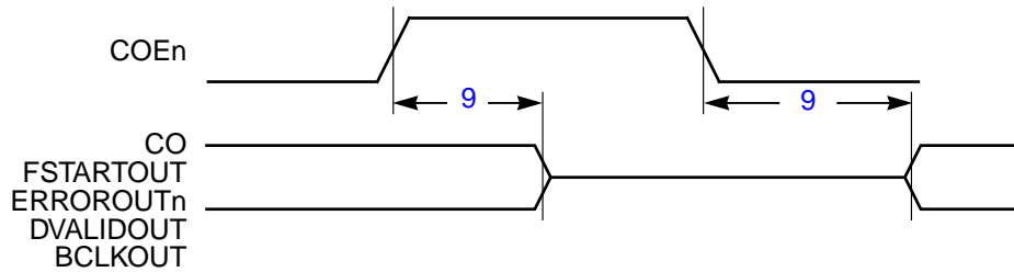
Figure 8.5 L64724 Bus 3-State Delay Timing
