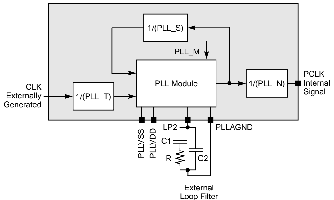
Figure 4.2 PLL Clock Synthesis
