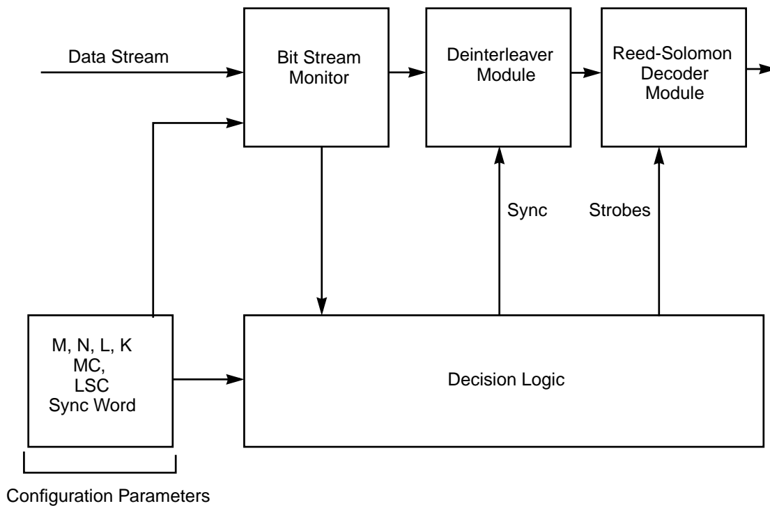
Figure 6.10 Reed-Solomon, Deinterleaver Synchronization
