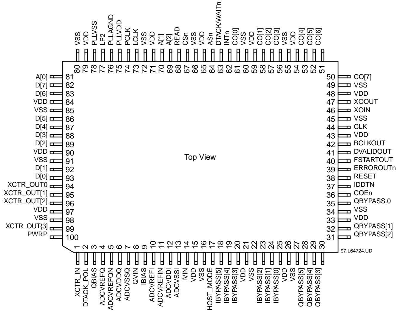
Figure 8.8 100-Pin PQFP/MQFP Pinout
