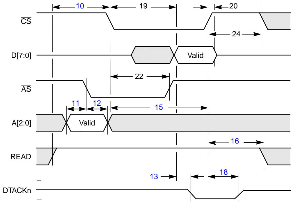
Figure 8.7 L64724 Decoder Write Cycle
