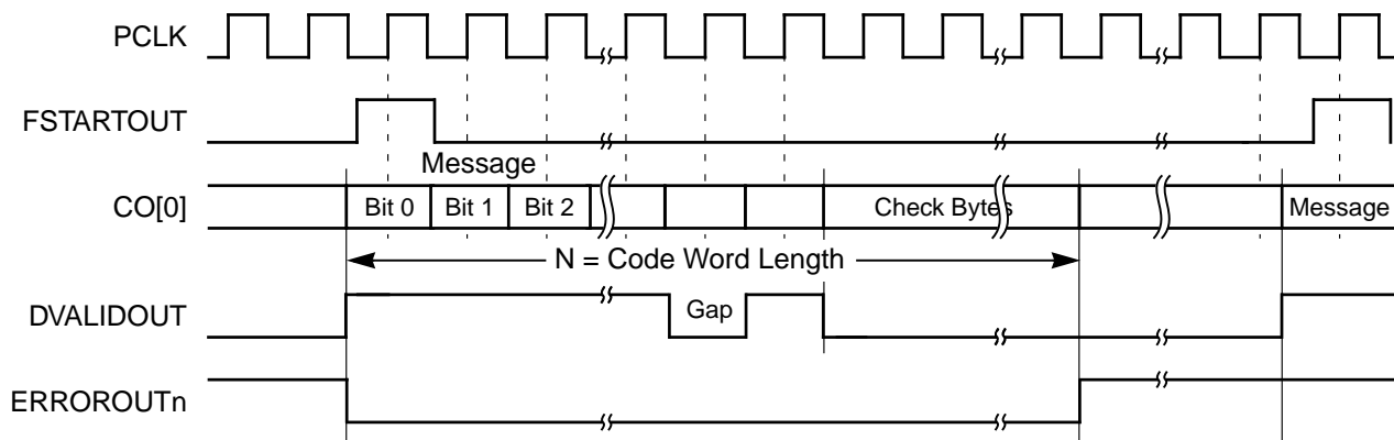
Figure 4.8 Descrambler Serial Output Waveforms
