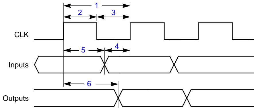
Figure 8.3 L64724 Synchronous AC Timing
