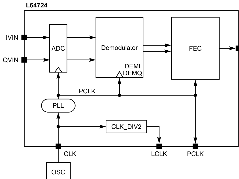
Figure 4.1 L64724 Clocking: Internal PLL
