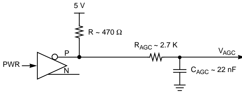
Figure 5.10 AGC Loop Control
