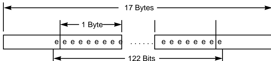
Figure 7.9 122-Bit Burst Example
