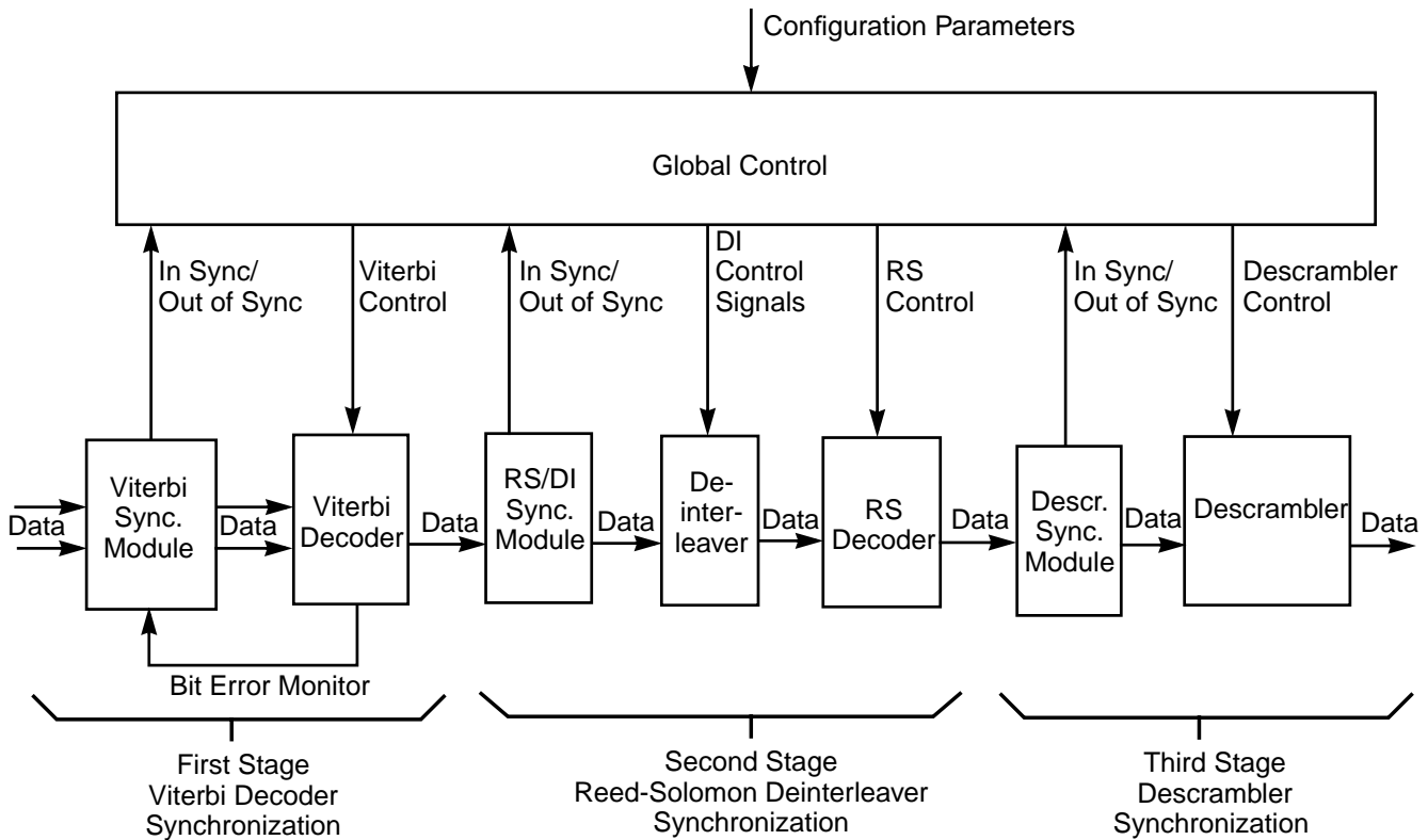
Figure 6.1 Synchronization Module
