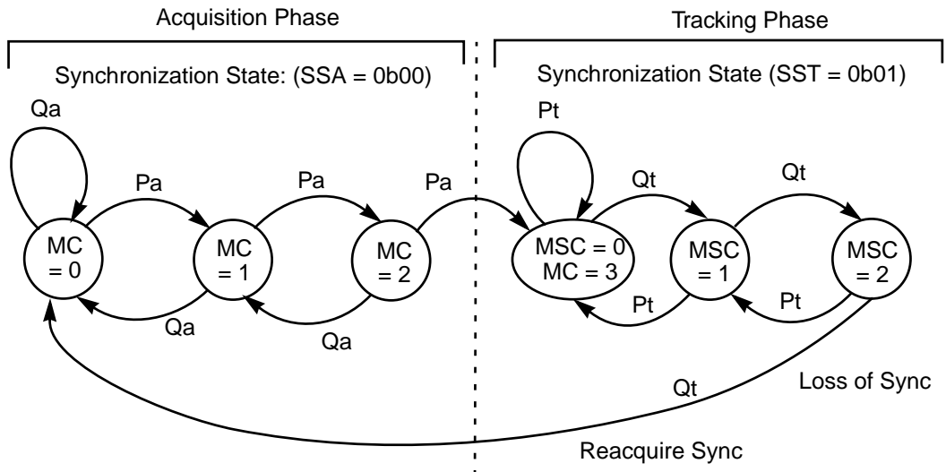
Figure 6.11 Synchronization, Tracking, and Loss of Sync for Three Missed Sync Words
