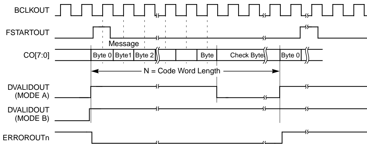
Figure 4.6 Parallel Output Interface Waveforms
