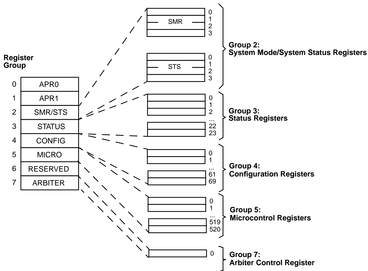
Figure 3.1 Register File Structure
