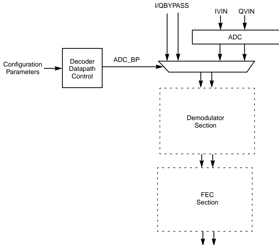
Figure 4.3 L64724 Functional Blocks in the Decoding Pipeline
