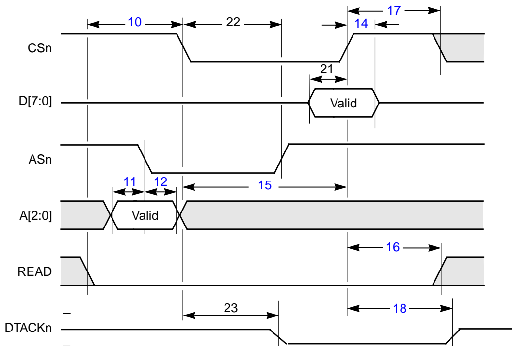
Figure 8.7 L64724 Decoder Write Cycle
