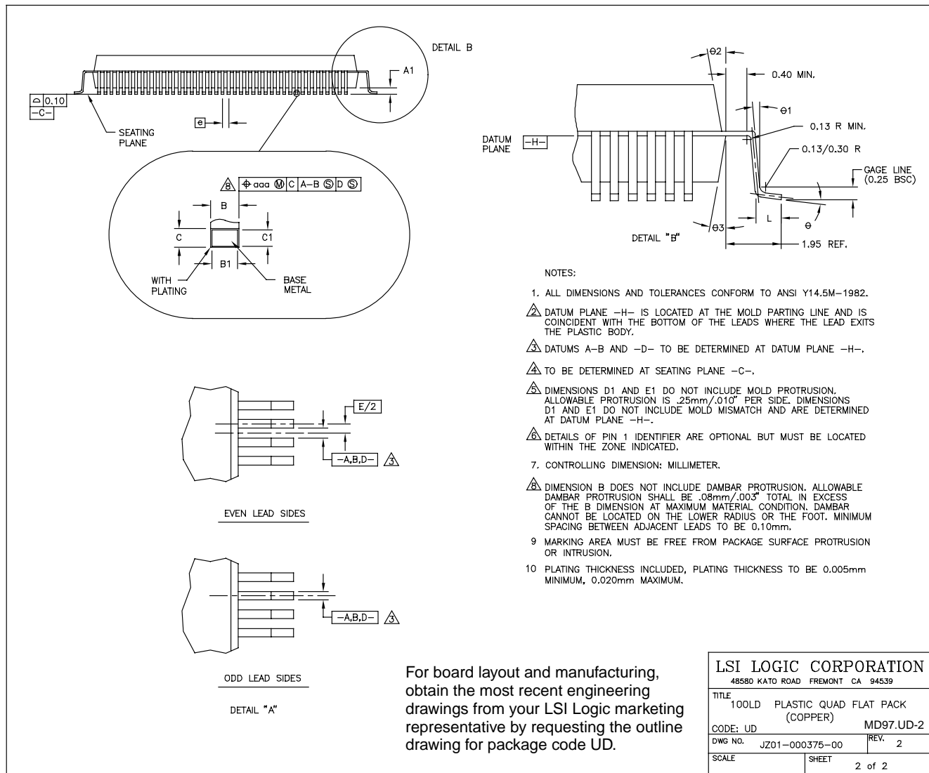
Figure 8.9 100-Pin PQFP/MQFP Mechanical Drawing (Cont.)
