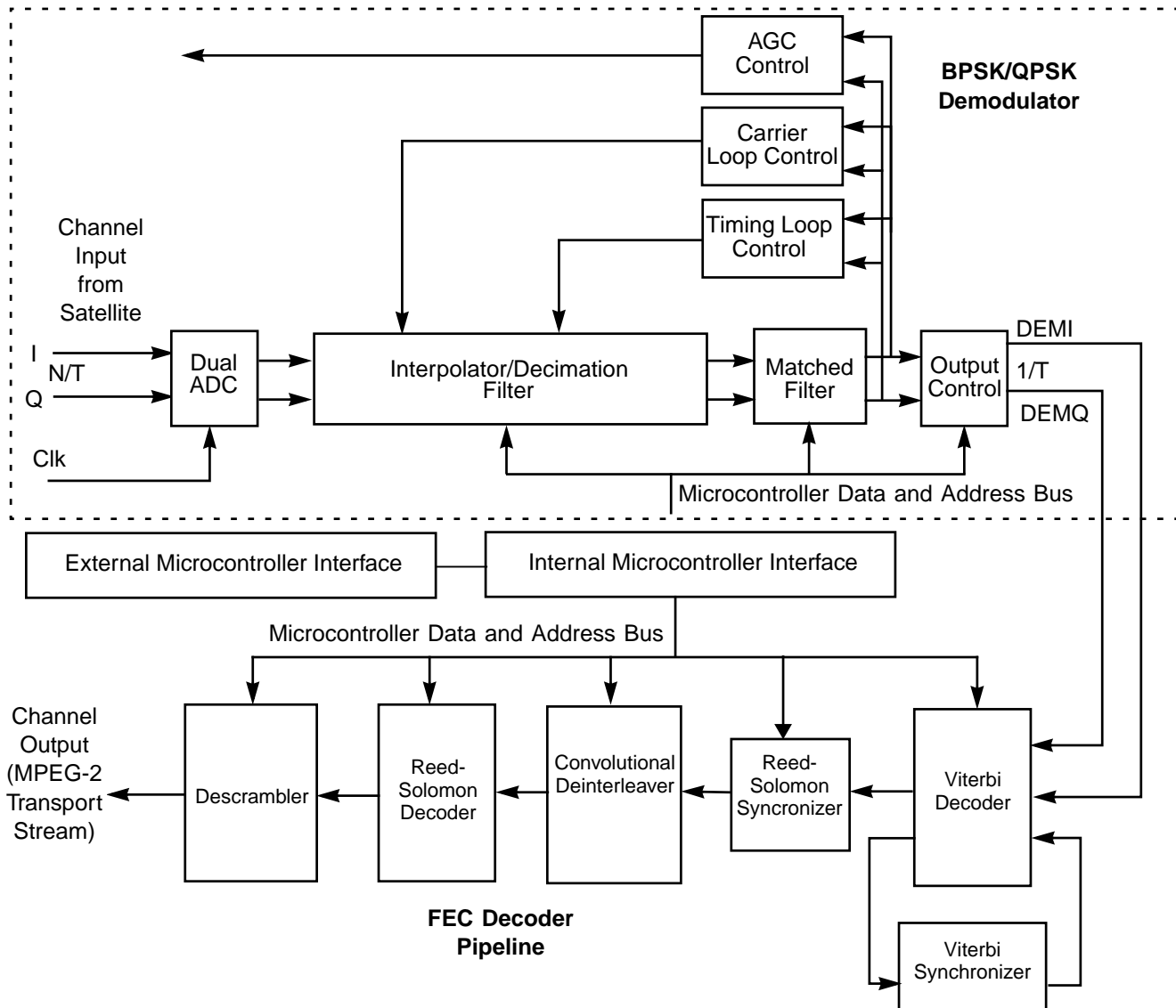
Figure 1.1 L64724 Block Diagram
