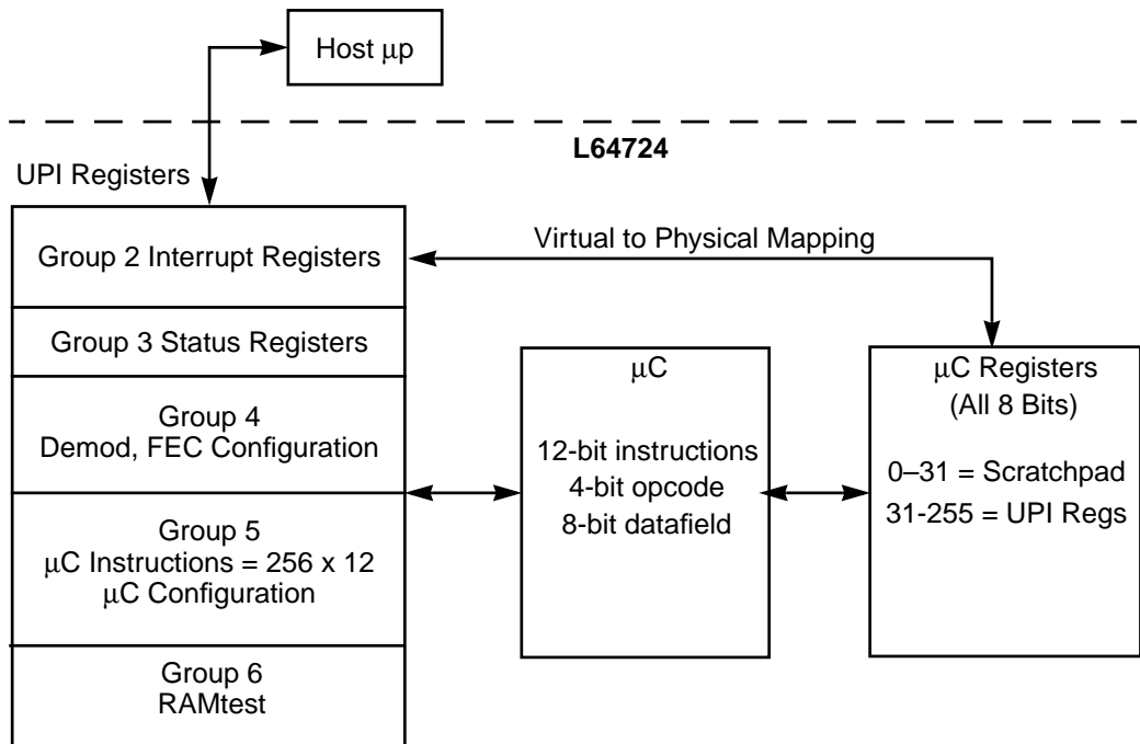
Figure E.1 Registers Shared Between the Host uP and L64724 \mu C
