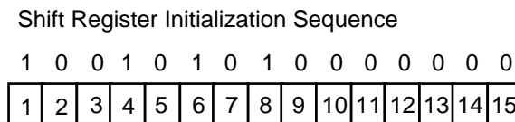
Figure 7.11 15-Bit Shift Register Initialization
