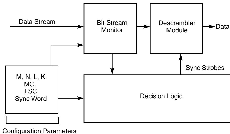
Figure 6.17 Descrambler Synchronization
