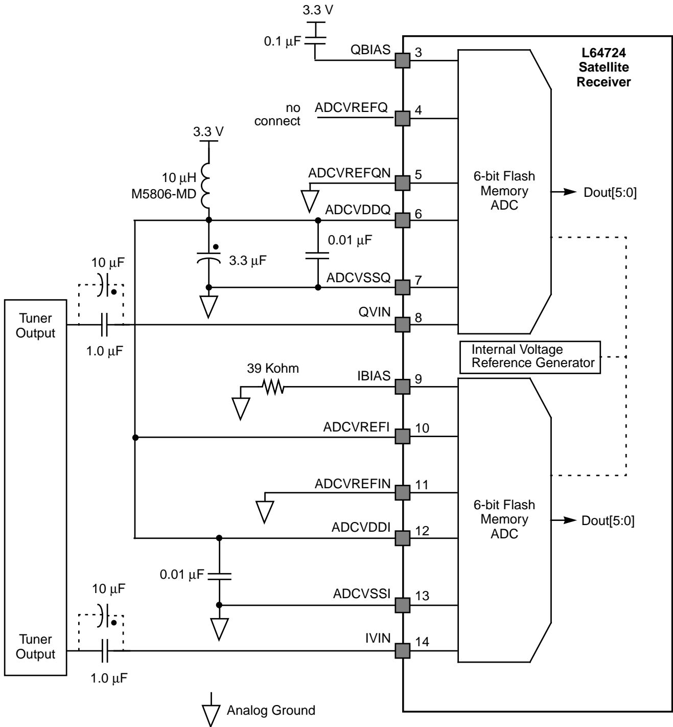
Figure D.2 ADC Board Level Interface
