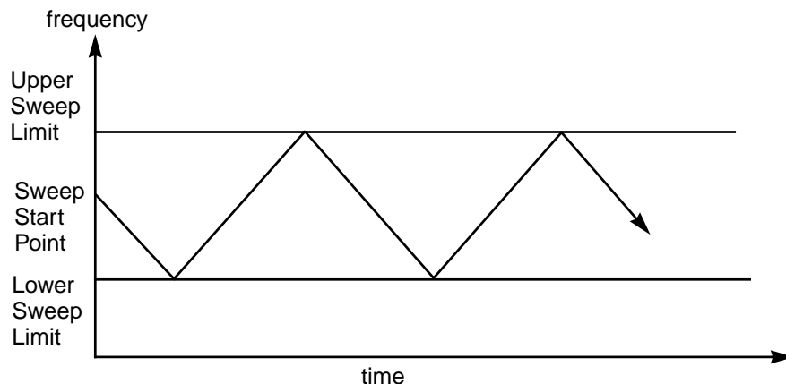
Figure 5.6 Frequency Sweeping
