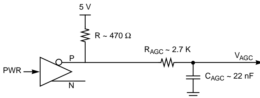
Figure B.1 AGC Loop Control
