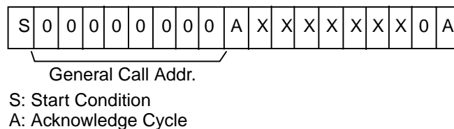
Figure A.4 General Call Structure
