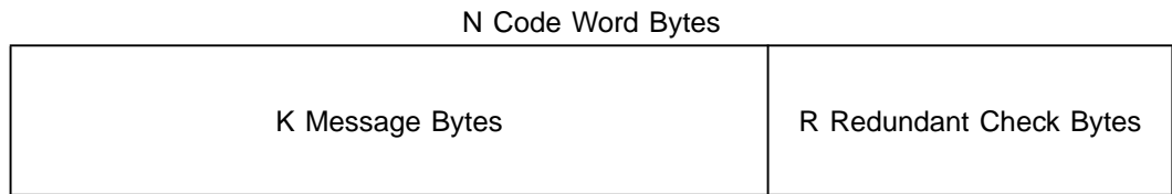
Figure 7.7 Code Word Structure
