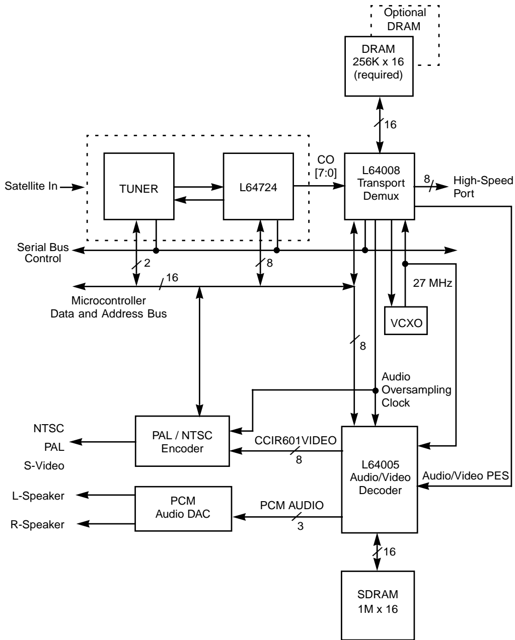
Figure 1.2 Set-Top Decoder Box Block Diagram
