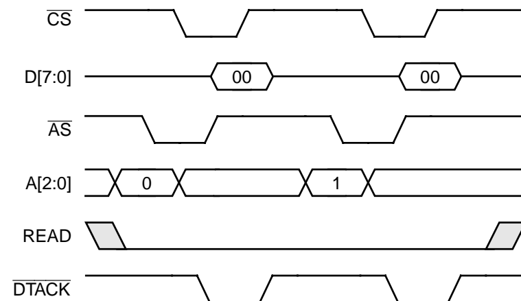
Figure 3.3 Initialize APR0 and APR1 to Zero
