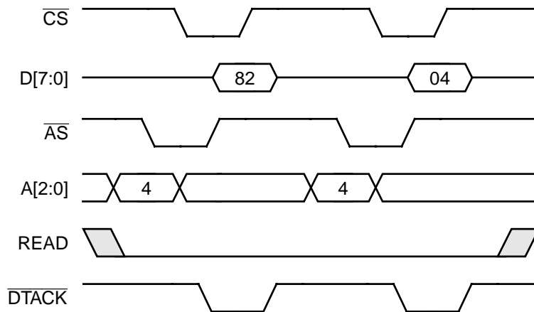
Figure 3.4 Write Locations 0 and 1 in Group 4
