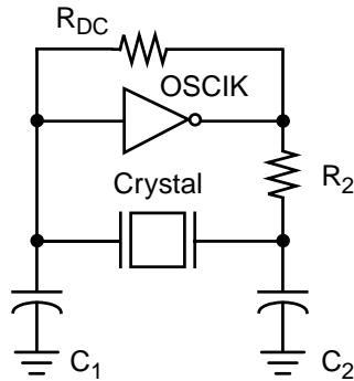
Figure C.4 A Low Frequency Range (kHz) Oscillator Circuit
