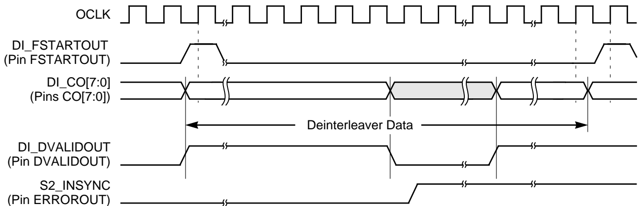
Figure 4.15 Deinterleaver Output Waveforms
