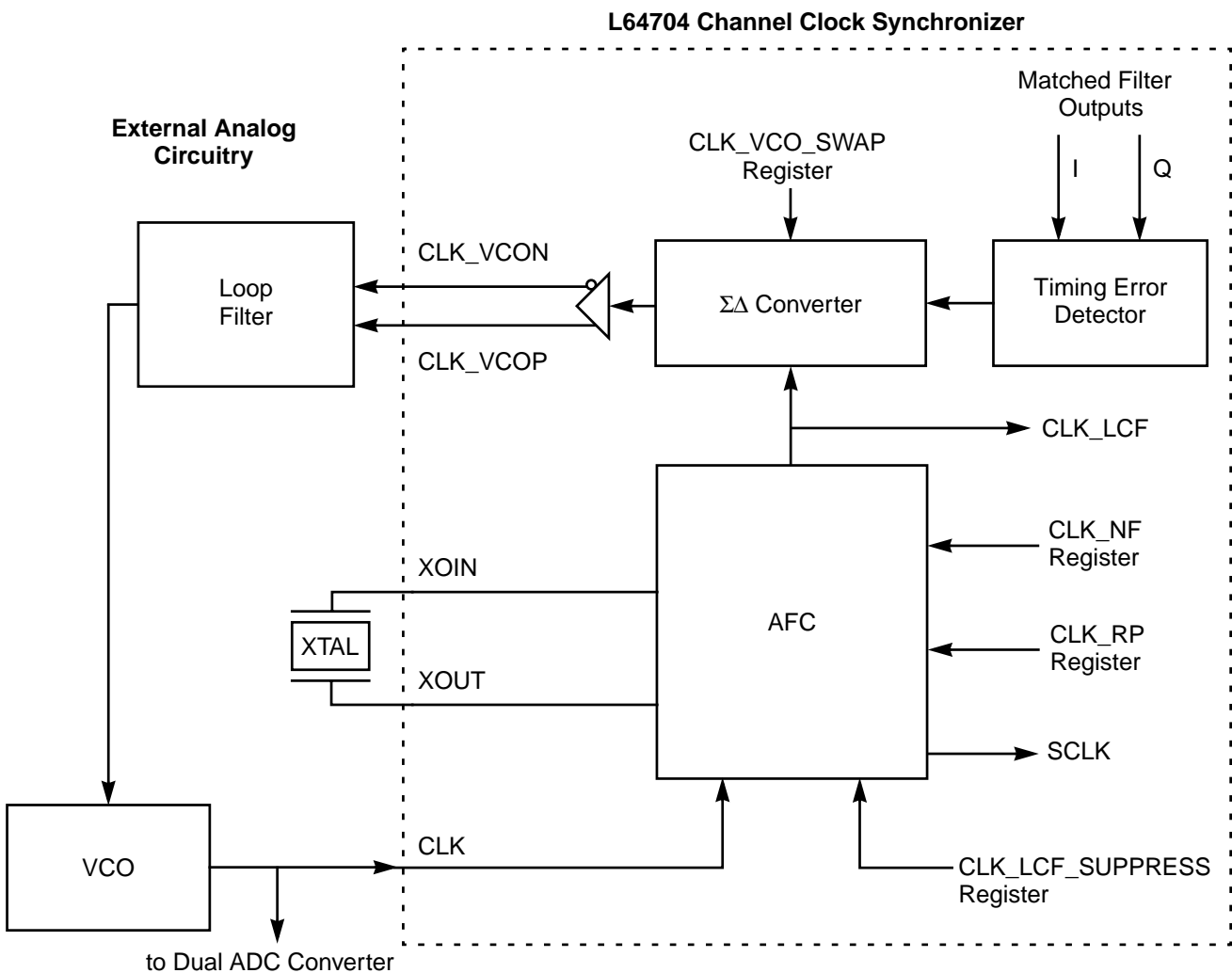
Figure 5.3 Clock Recovery Loop
