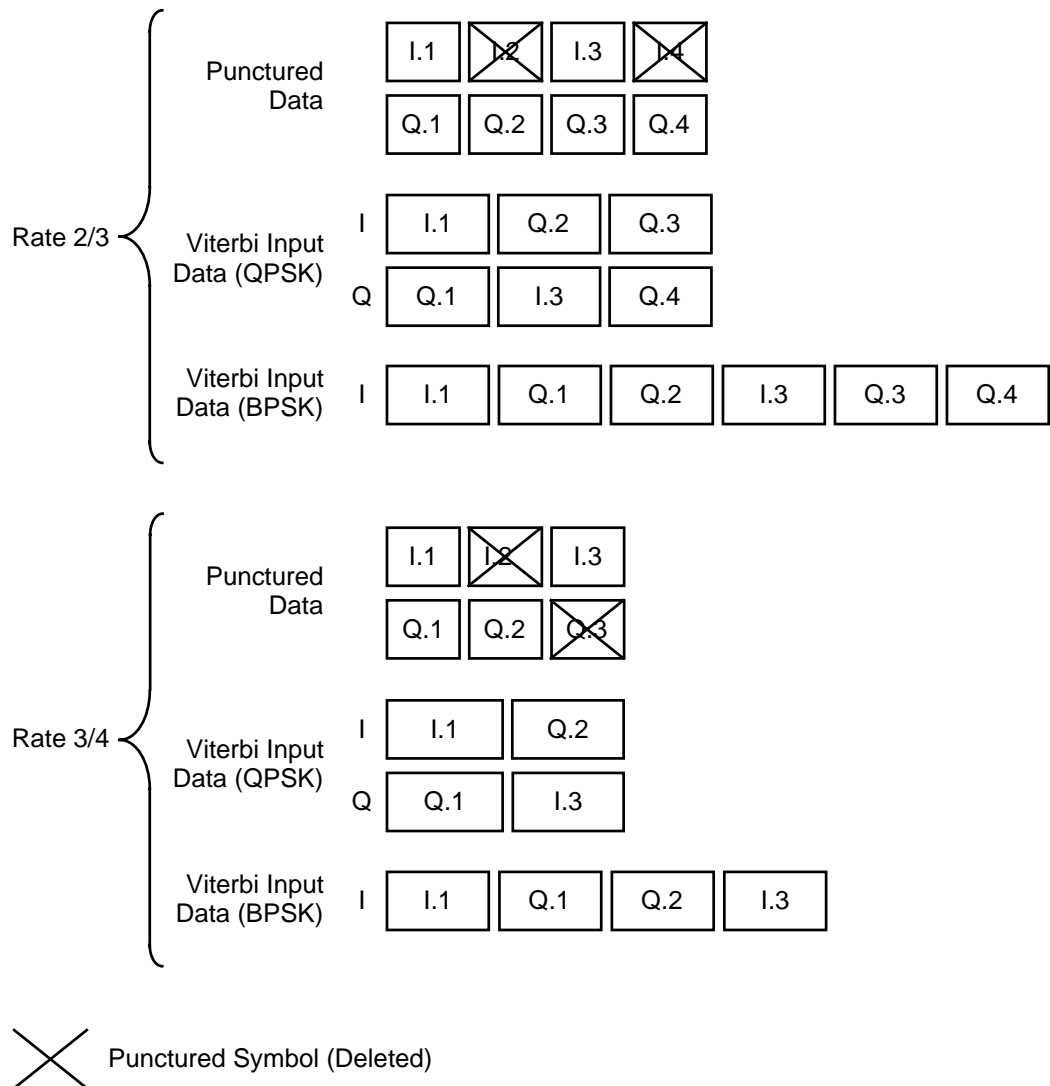
Figure 7.4 Puncture Pattern for Different Code Rates
