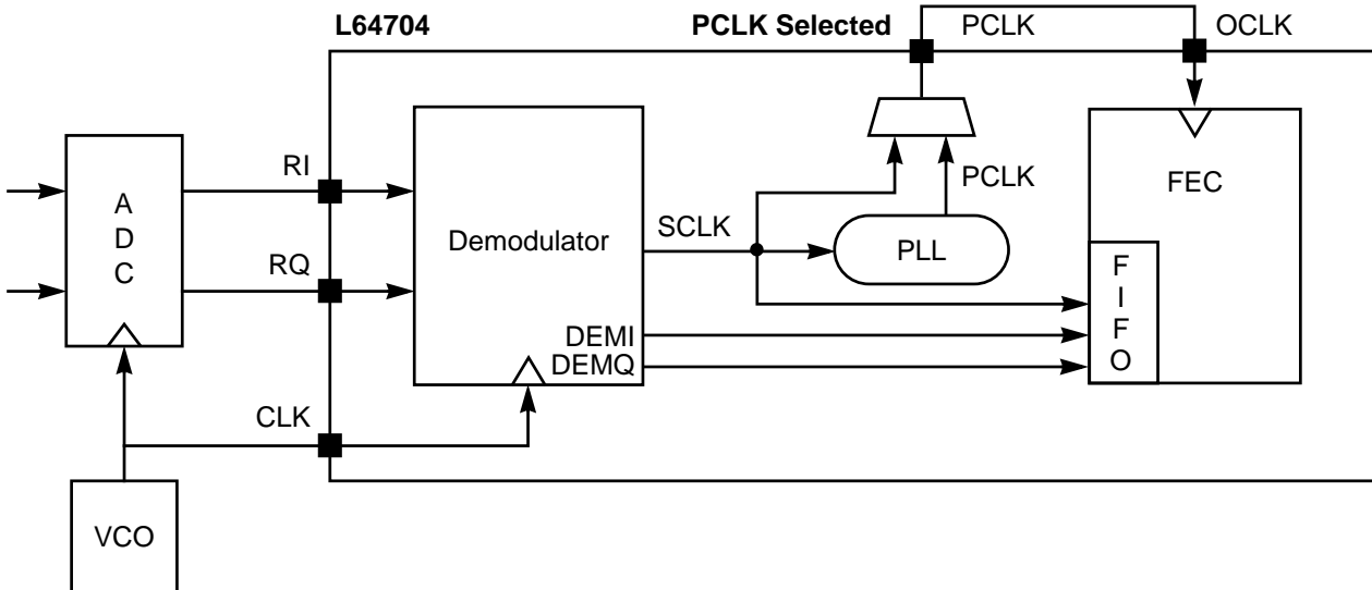
Figure 4.1 L64704 Clocking: Internal PLL
