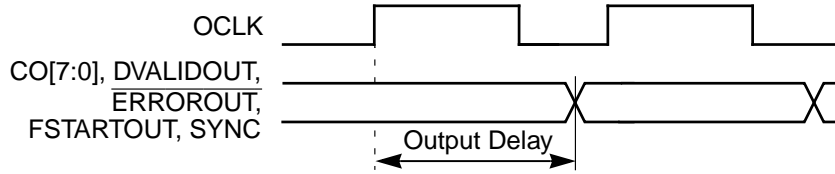
Figure 4.6 OCLK Reference to Channel Data Output
