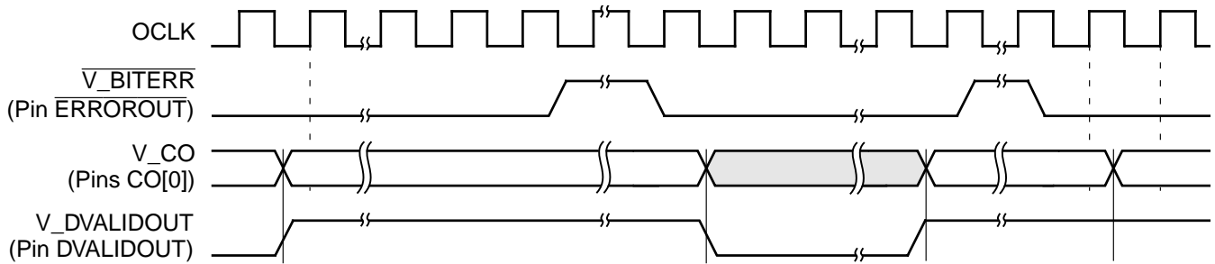
Figure 4.17 Viterbi Decoder Output Waveforms
