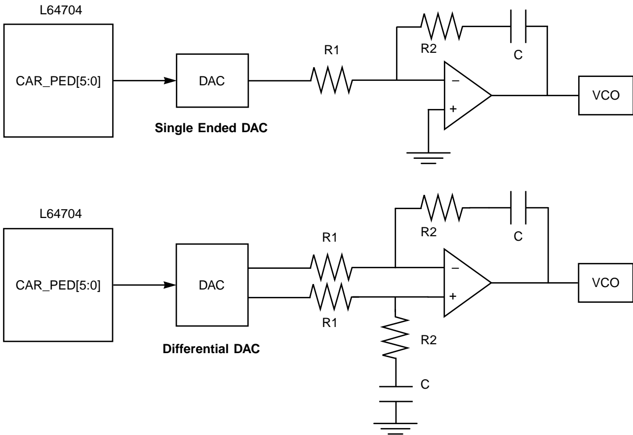
Figure 5.10 Using CAR_PED Outputs
