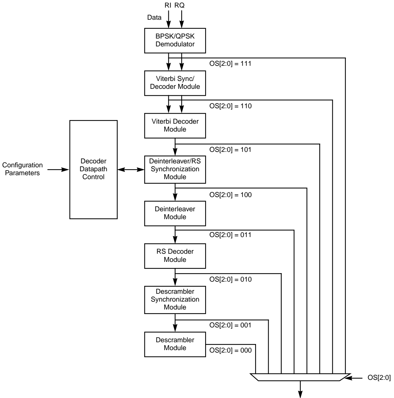
Figure 4.10 L64704 Functional Blocks in the Decoding Pipeline
