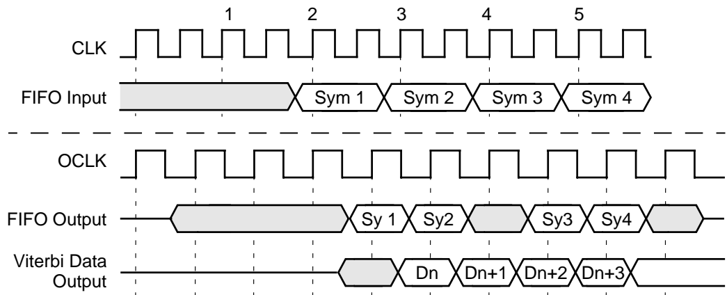
Figure 4.4 Code Rate = 3/4 System; Different OCLK and CLK
