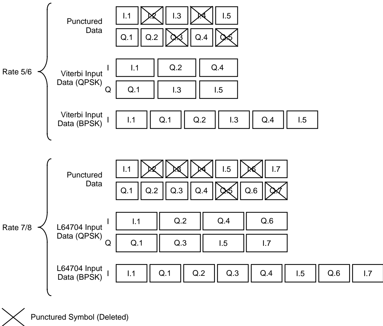
Figure 7.4 (Cont.) Puncture Pattern for Different Code Rates
