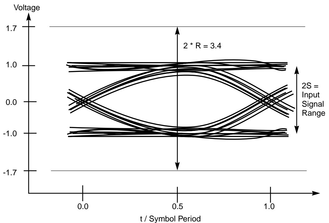
Figure 5.11 Eye Pattern and ADC Range
