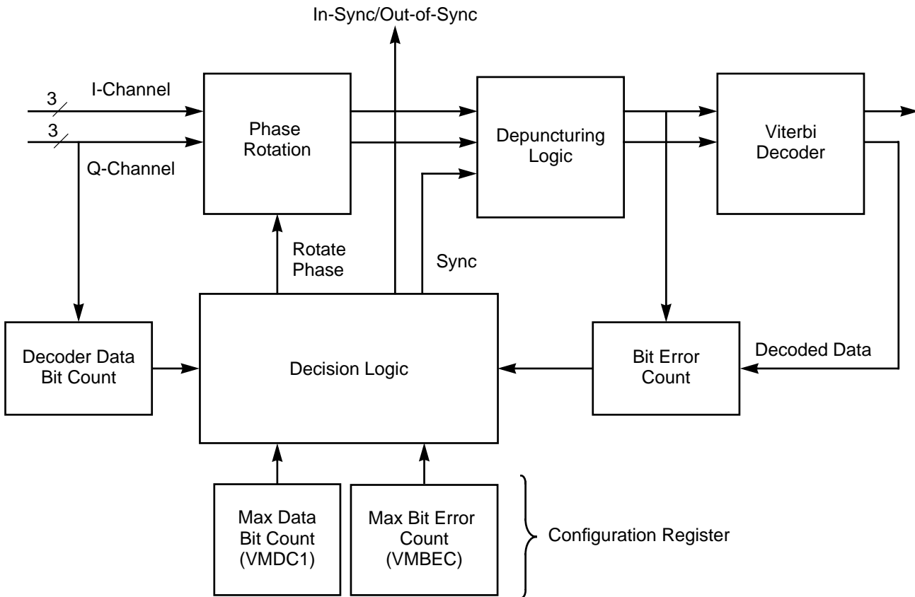
Figure 6.2 Viterbi Decoder Synchronization
