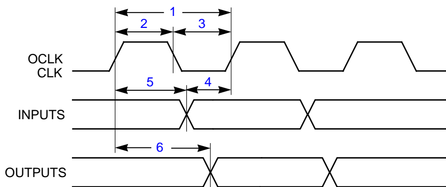
Figure 8.3 L64704 Synchronous AC Timing
