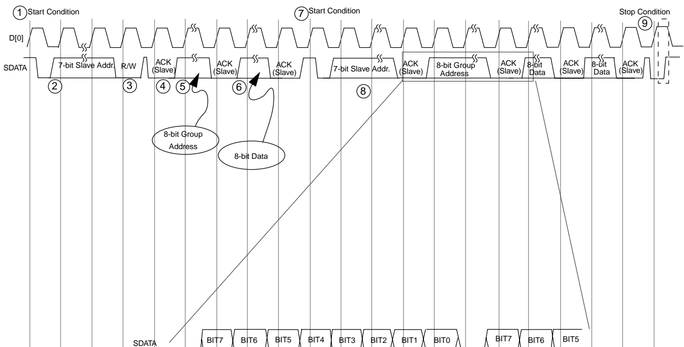
Figure A.4 Burst Write to Slave (Master-Txmitter, Slave-Receiver)
