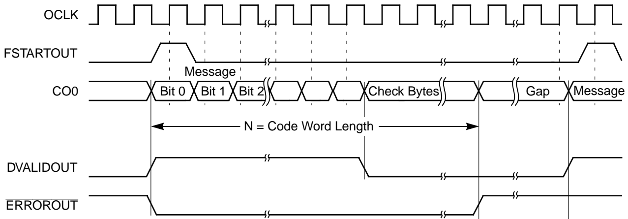
Figure 4.11 Descrambler Serial Output Waveforms
