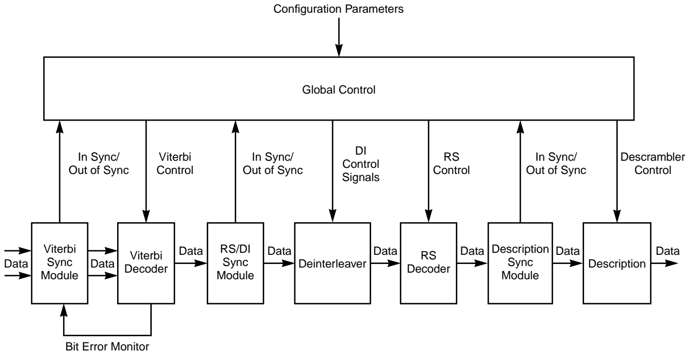
Figure 6.1 Synchronization Module
