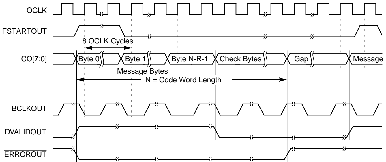
Figure 4.12 Descrambler Parallel Output Format
