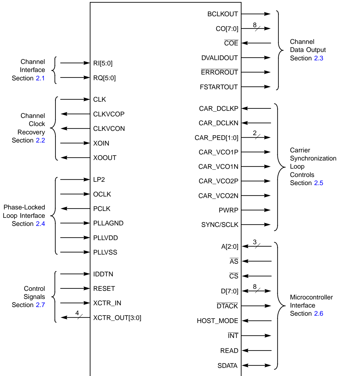
Figure 2.1 L64704 Logic Diagram
