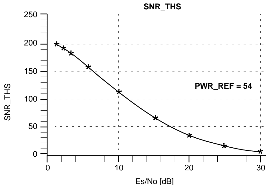
Figure 5.7 SNR Threshold vs. ES/No
