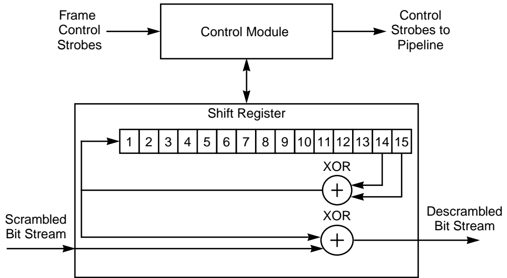
Figure 7.18 Descrambler Block Diagram
