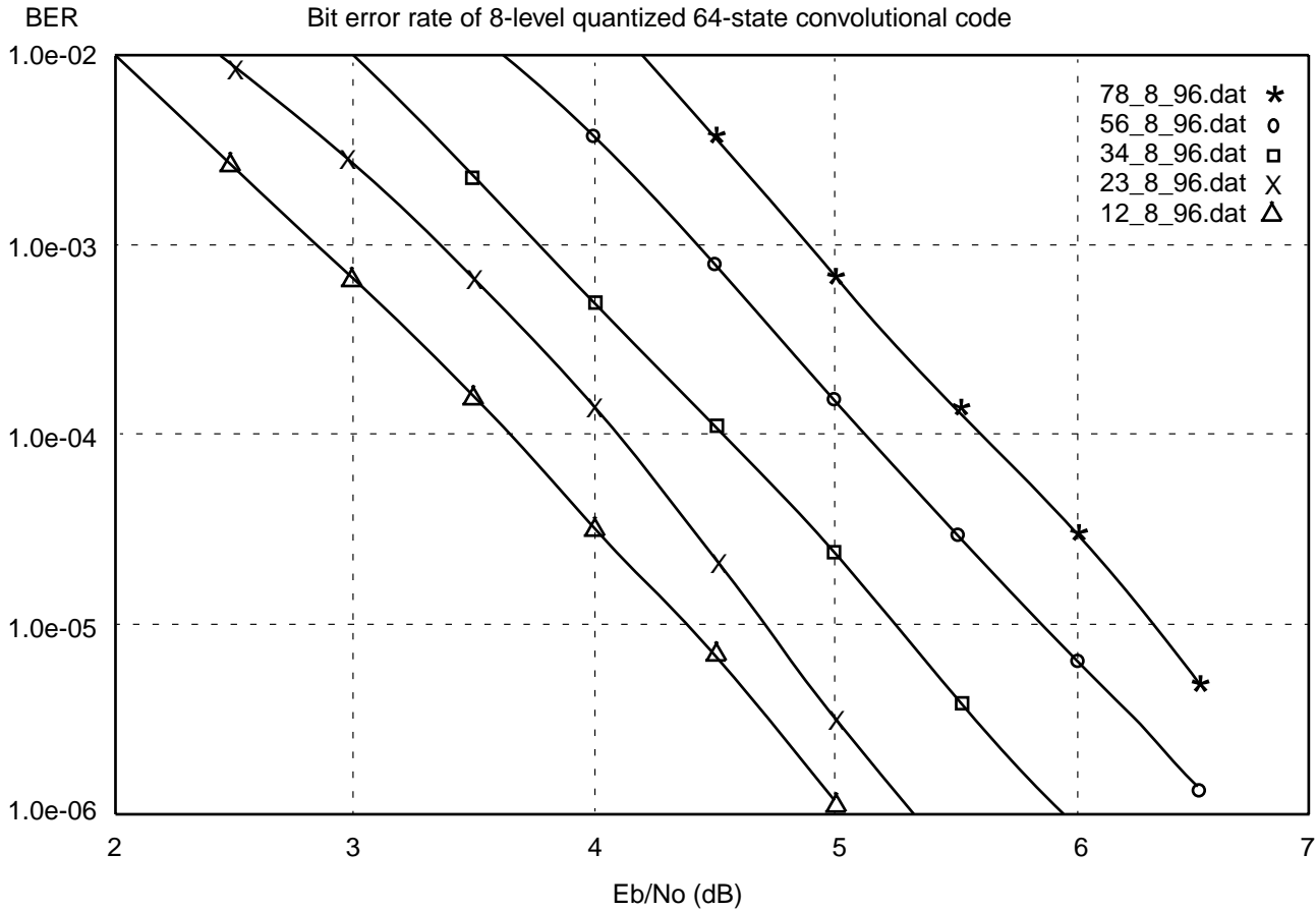
Figure 7.2 Code Performance for Viterbi Decoder
