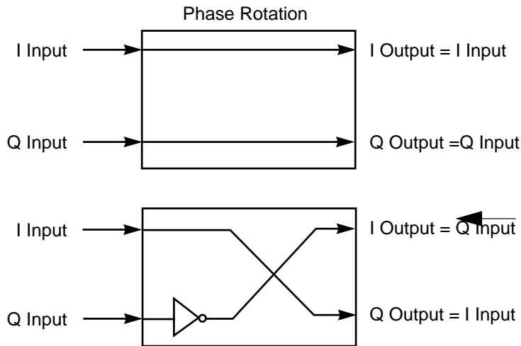
Figure 6.3 Phase Rotation for Synchronization
