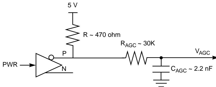
Figure 5.12 AGC Loop Control
