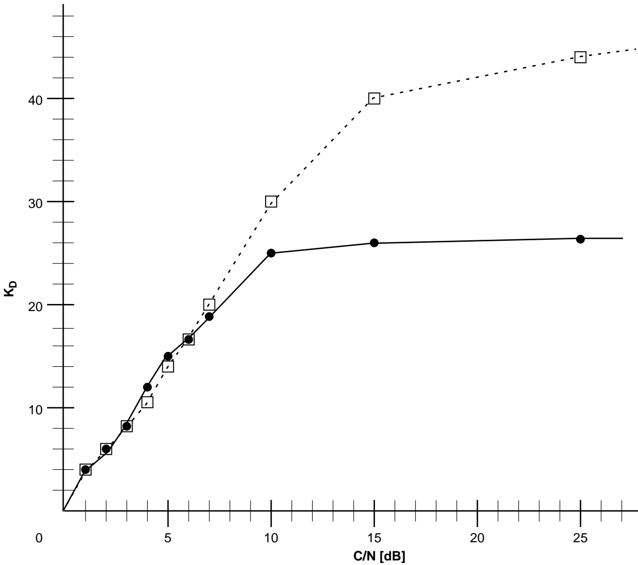
Figure 5.9 PED Slope
