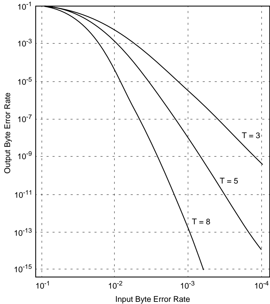
Figure 7.17 (255, 255-2T) Code Performance
