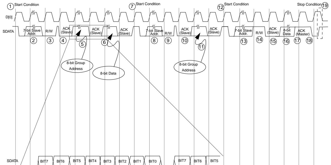
Figure A.5 Single Read From Slave
