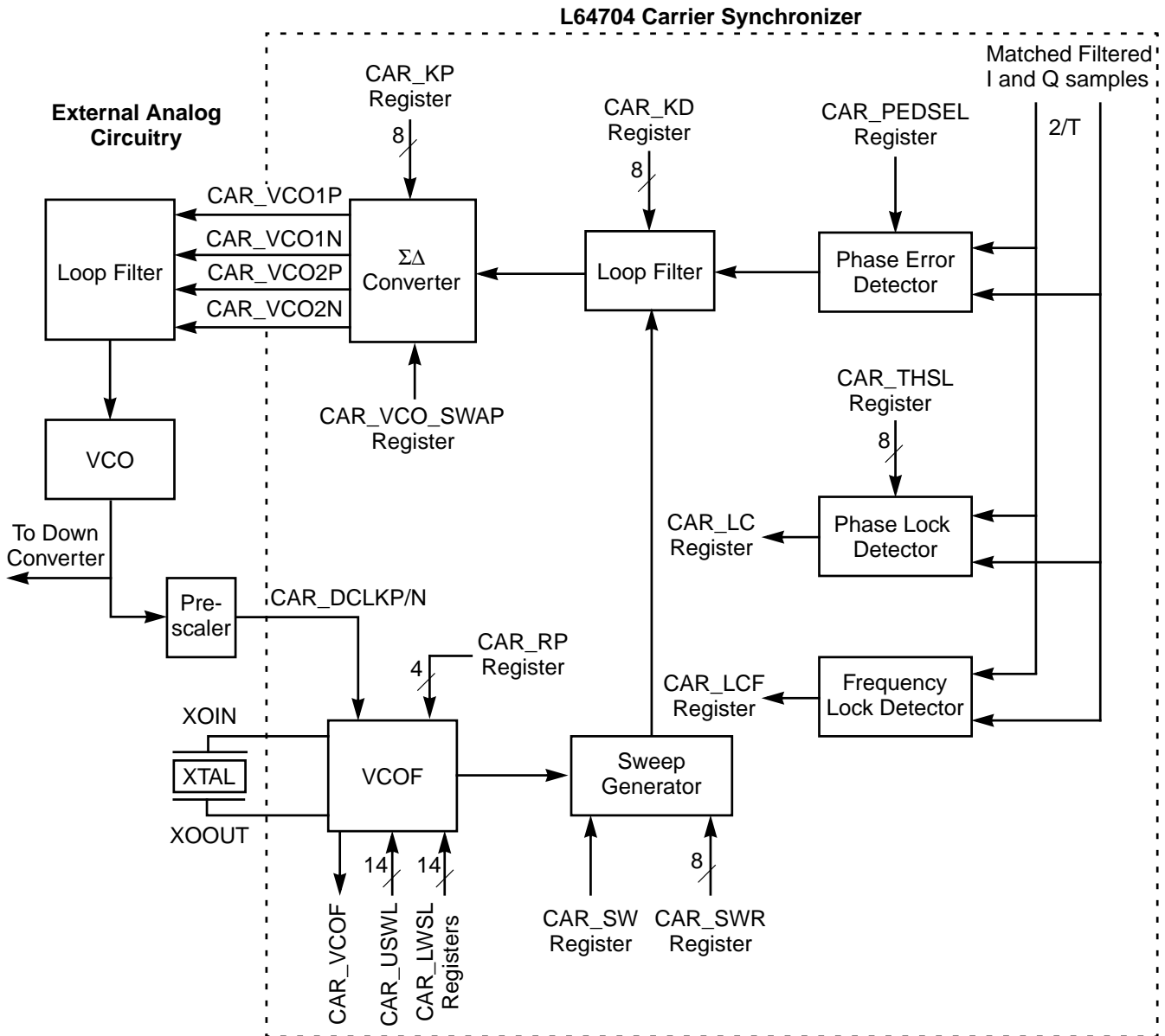
Figure 5.5 Carrier Recovery Loop
