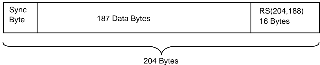
Figure 6.8 MPEG-2 Transport Packet
