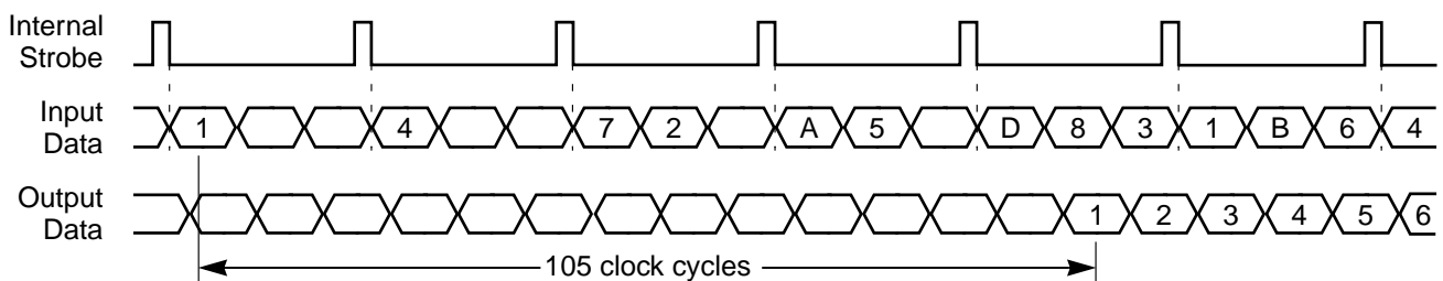
Figure 7.13 Deinterleaver Output Example
