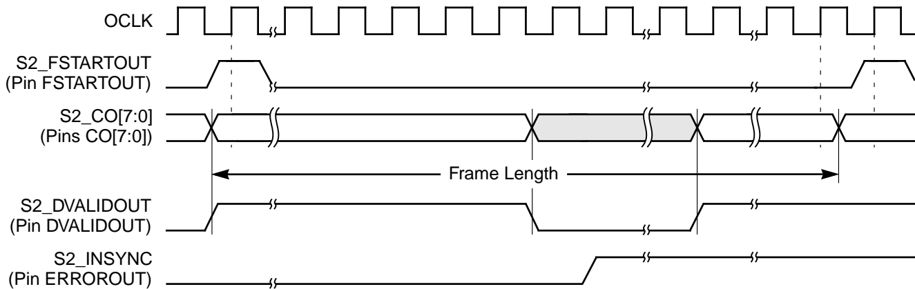
Figure 4.16 Synchronization Stage 2 Output Waveforms
