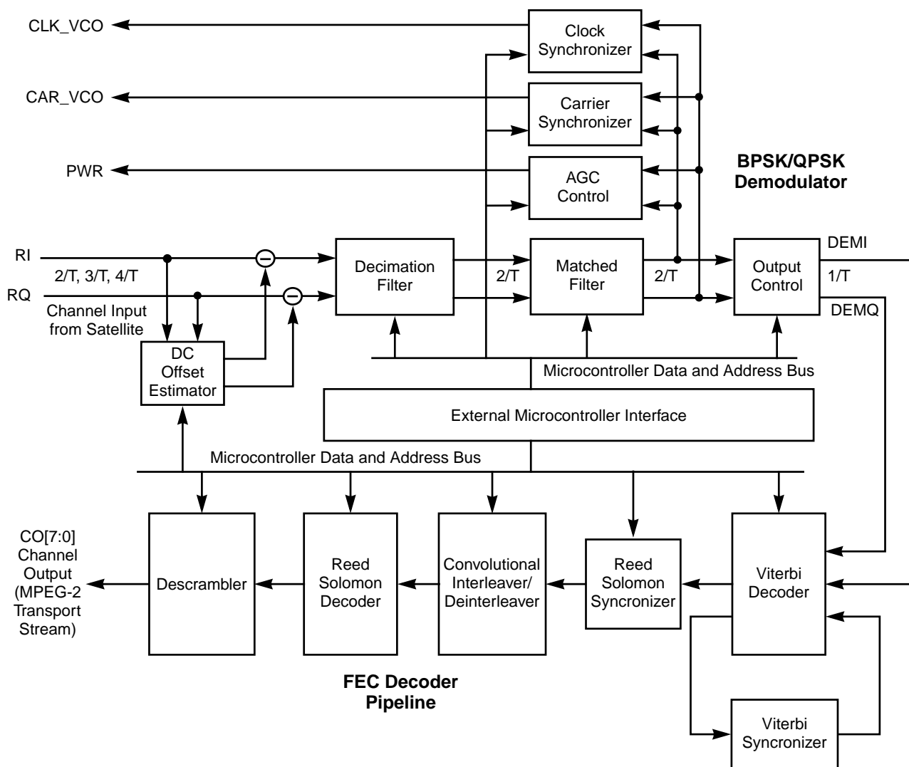
Figure 1.1 L64704 Block Diagram
