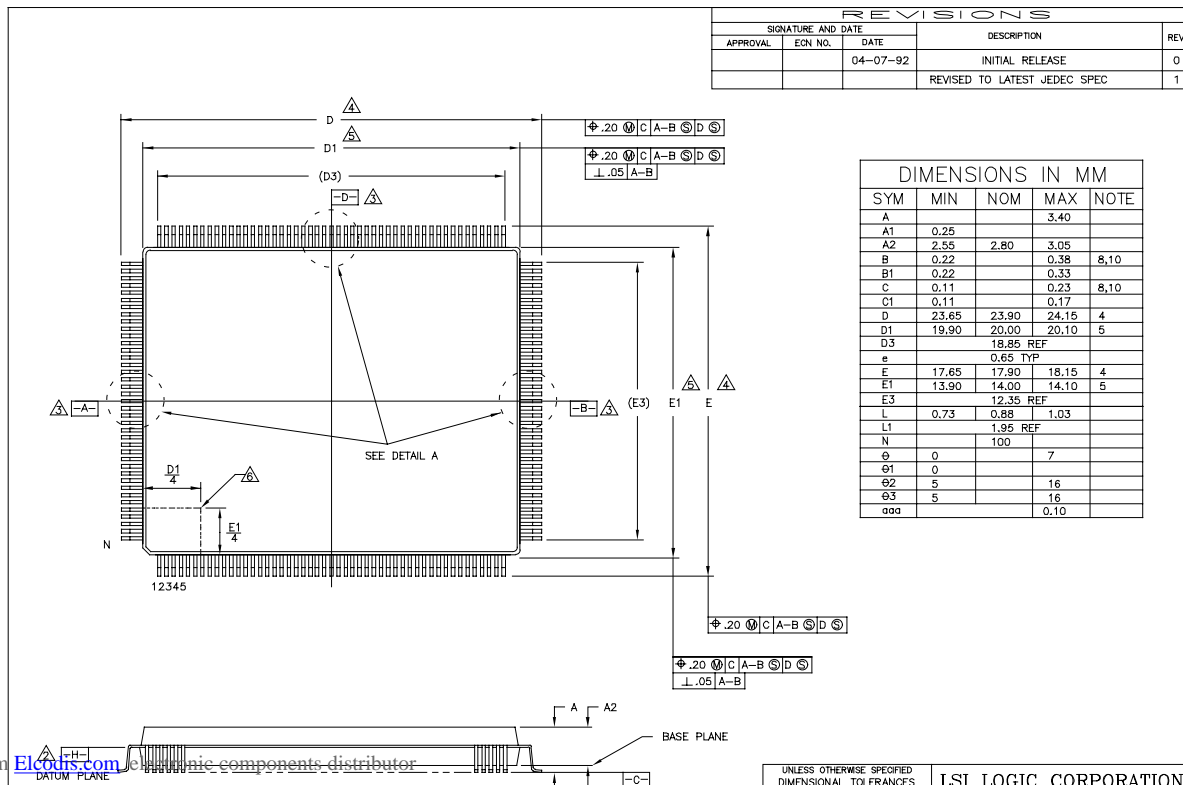
Figure 8.9 100-Pin PQFP Mechanical Drawing (Sheet 1 of 2)
