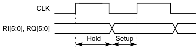
Figure 4.5 CLK Reference to Channel Data Input
