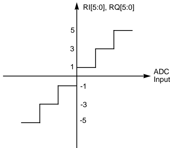
Figure 5.2 Input Quantization with AC Coupling
