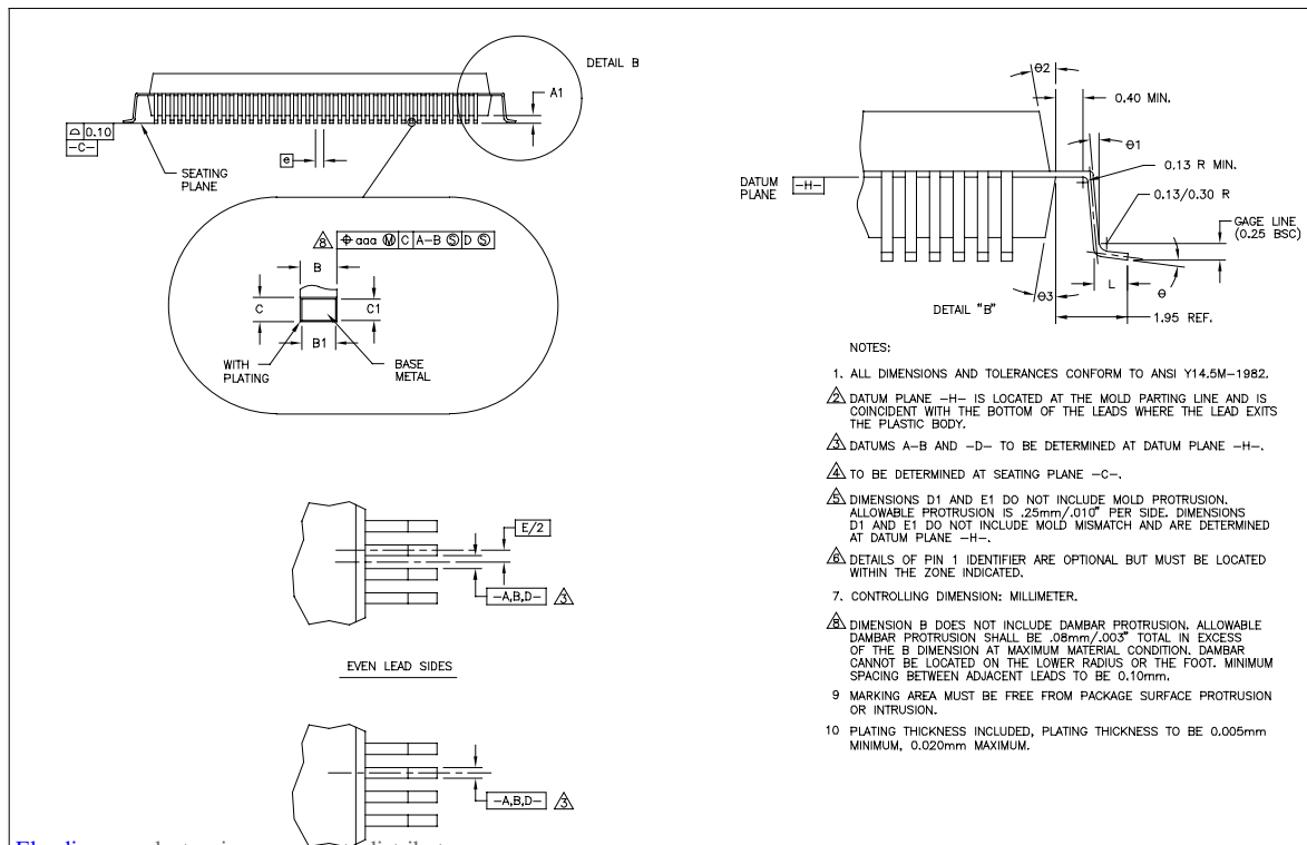
Figure 8.9 (Cont.) 100-Pin PQFP Mechanical Drawing (Sheet 2 of 2)
