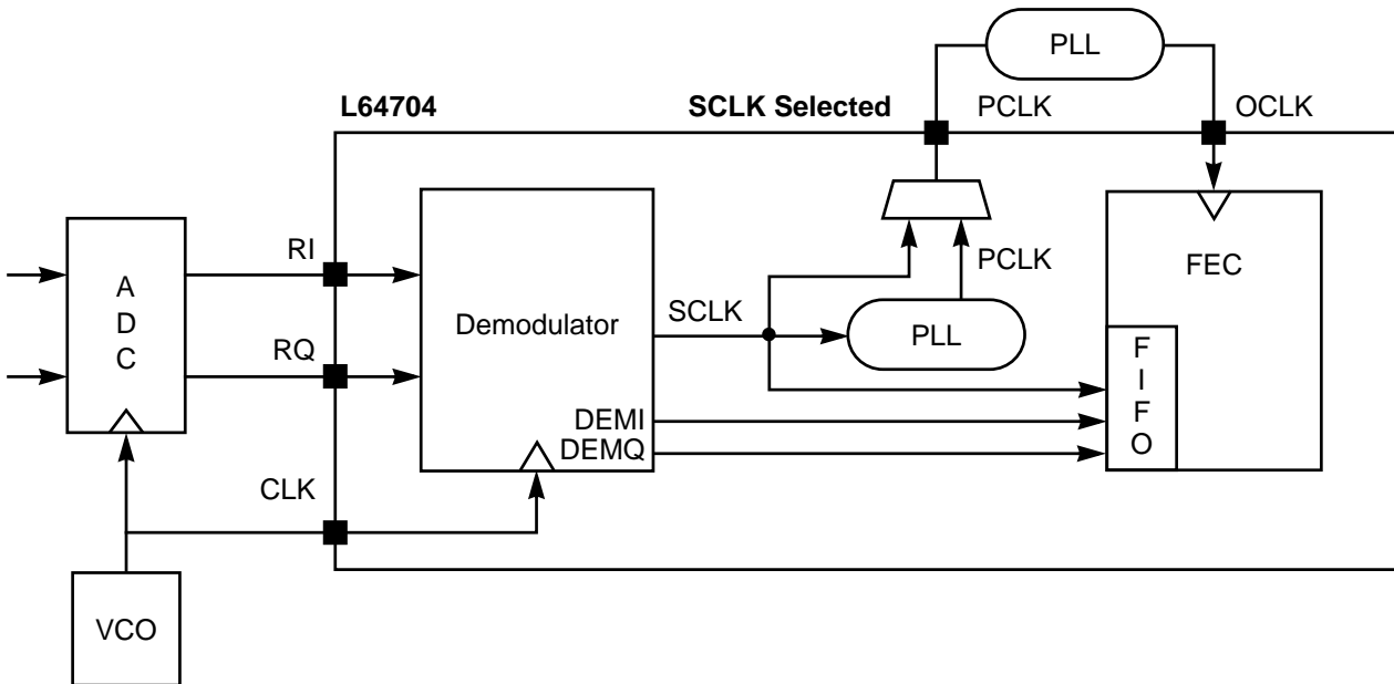
Figure 4.2 L64704 Clocking: External PLL
