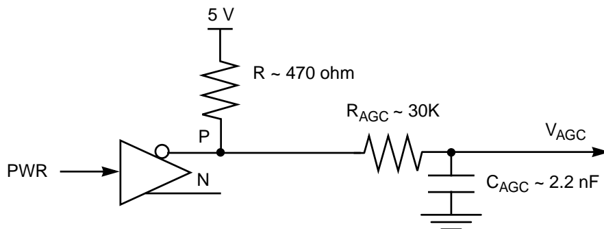
Figure B.2 AGC Loop Control
