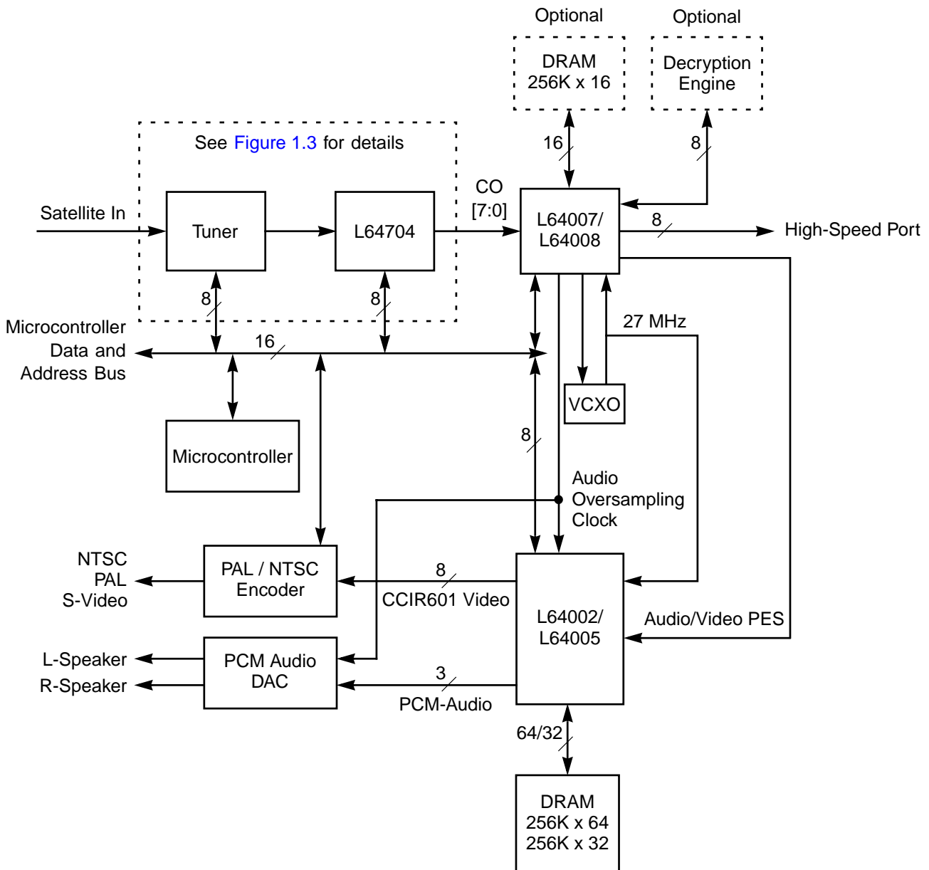
Figure 1.2 Set-Top Decoder Box Block Diagram
