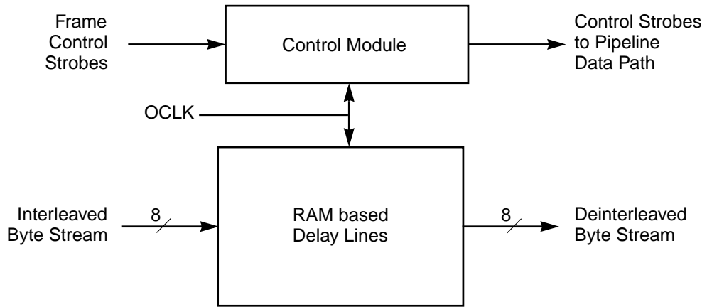
Figure 7.12 Block Diagram of Deinterleaver Core
