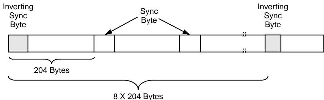
Figure 6.9 L64704 Transport Packet
