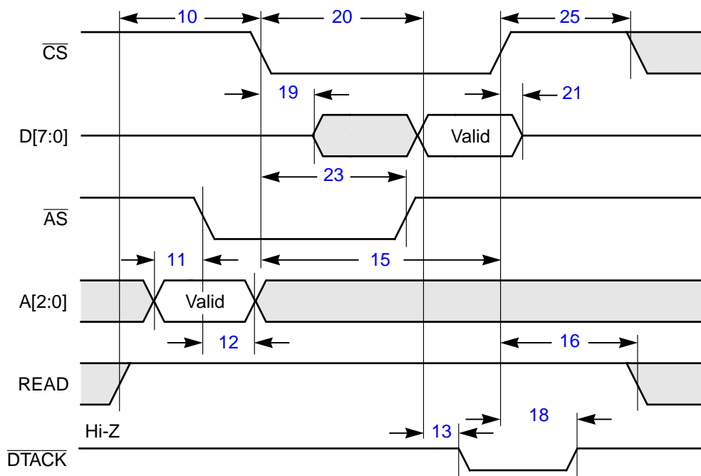
Figure 8.6 L64704 Decoder Read Cycle
