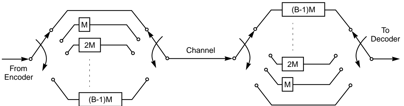
Figure 7.11 Interleaving/ Deinterleaving Operation
