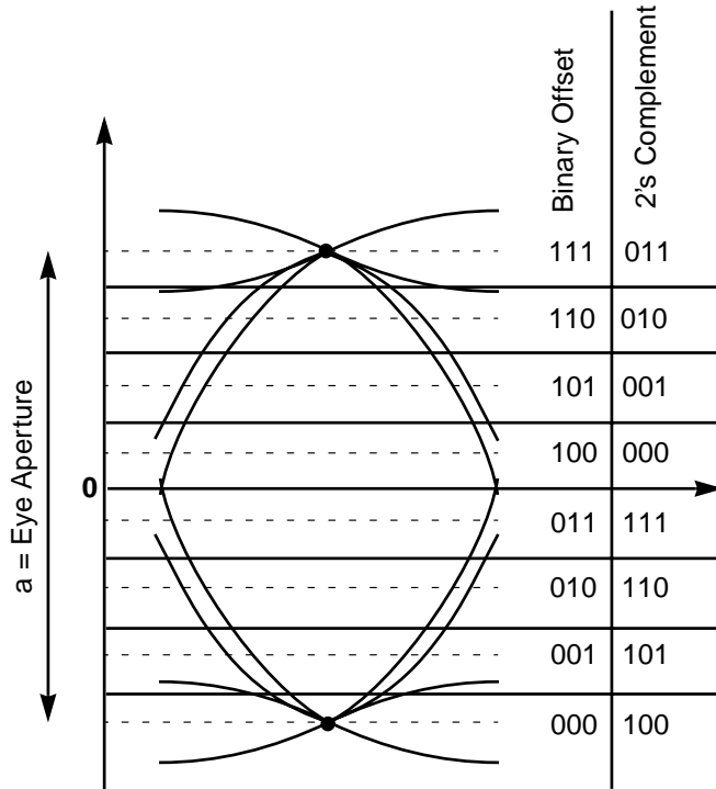
Figure 5.13 Eye Pattern and Soft Decision Thresholds
