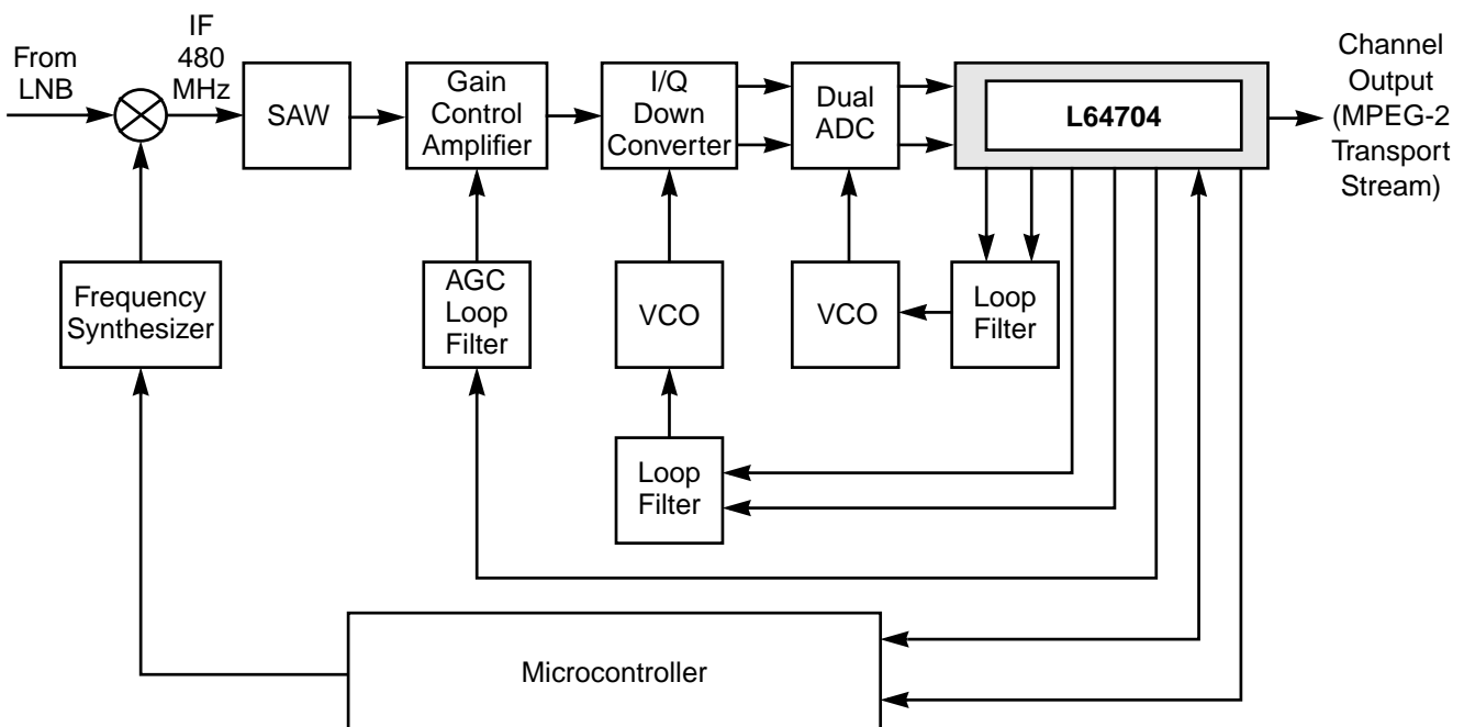
Figure 1.3 Typical Receiver Block Diagram with L64704
