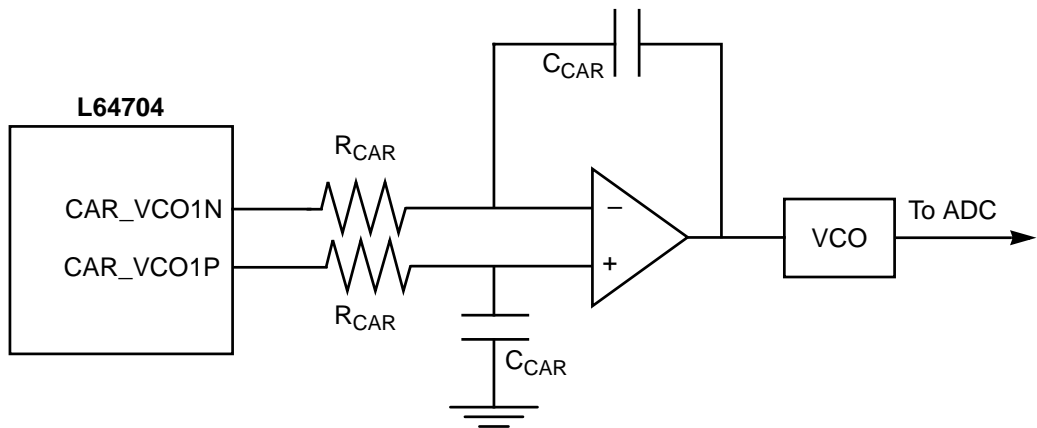
Figure 5.8 Carrier Loop Filter Schematic
