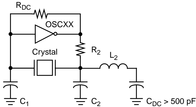
Figure C.3 A Third Overtone (Higher Frequency) Oscillator Circuit
