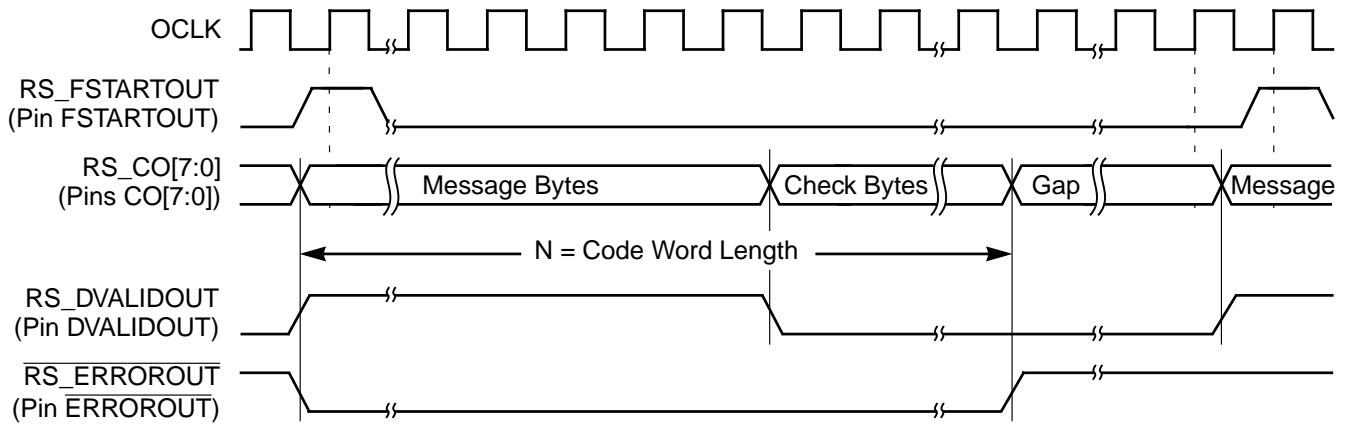
Figure 4.14 Reed-Solomon Decoder Output Waveforms
