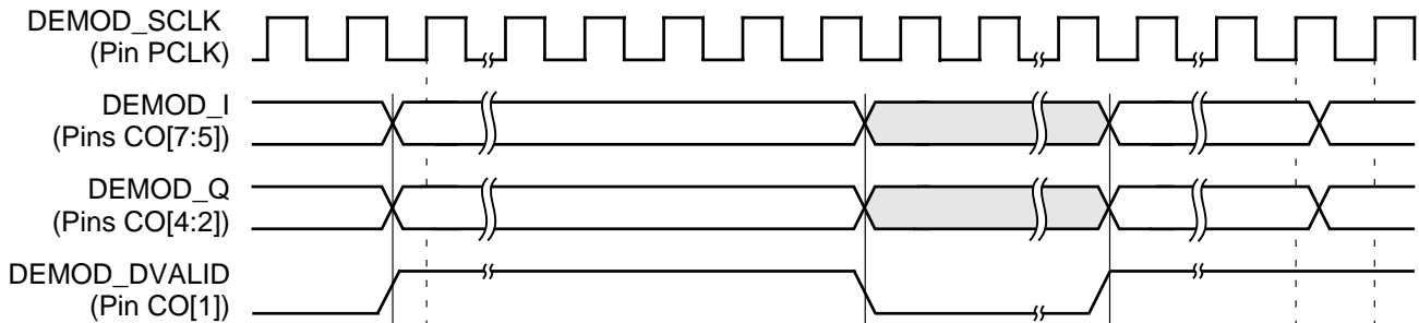
Figure 4.19 QPSK Demodulator Output Waveforms
