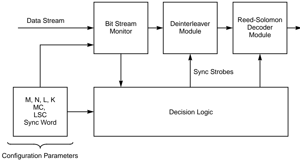
Figure 6.4 Reed-Solomon, Deinterleaver Synchronization
