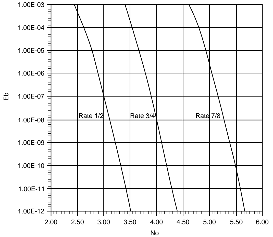
Figure 1.4 Concatenated Decoding Performance for L64704
