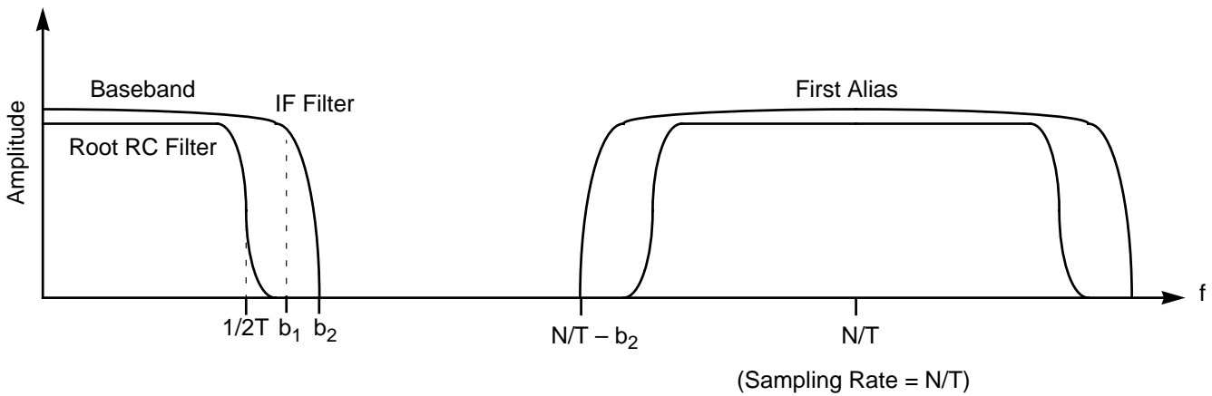
Figure 5.4 Spectrum of Oversampled Signal
