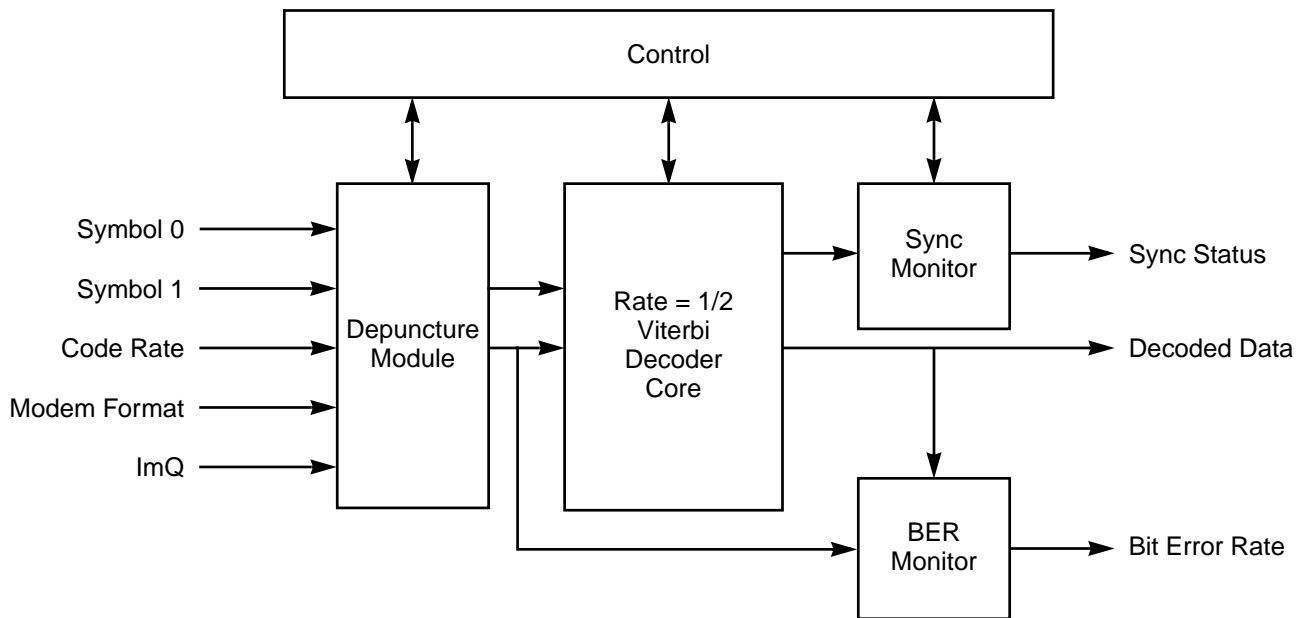
Figure 7.1 Block Diagram of Viterbi Decoder Core
