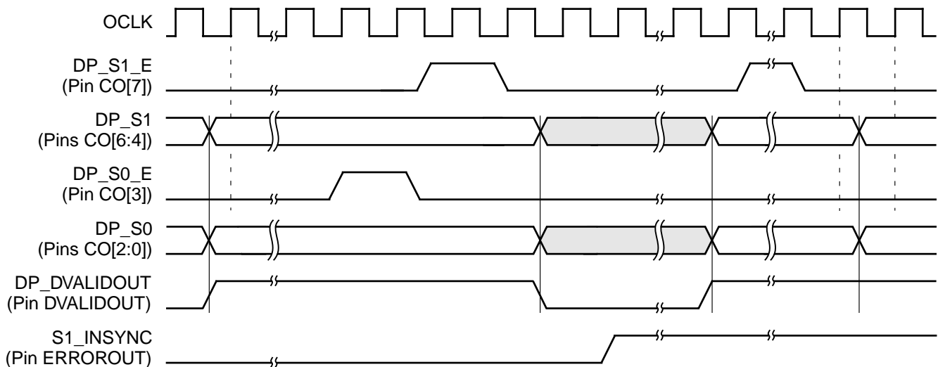
Figure 4.18 Viterbi Depuncture/ Synchronization Output Waveforms
