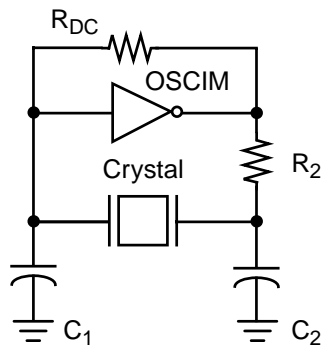
Figure C.2 Pierce Crystal Oscillator Circuit
