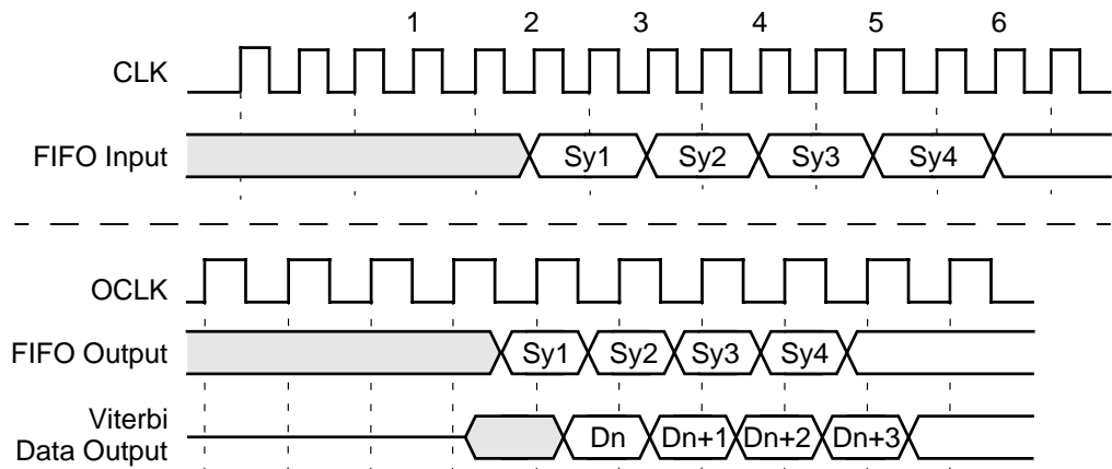
Figure 4.3 Code Rate = 1/2 System
