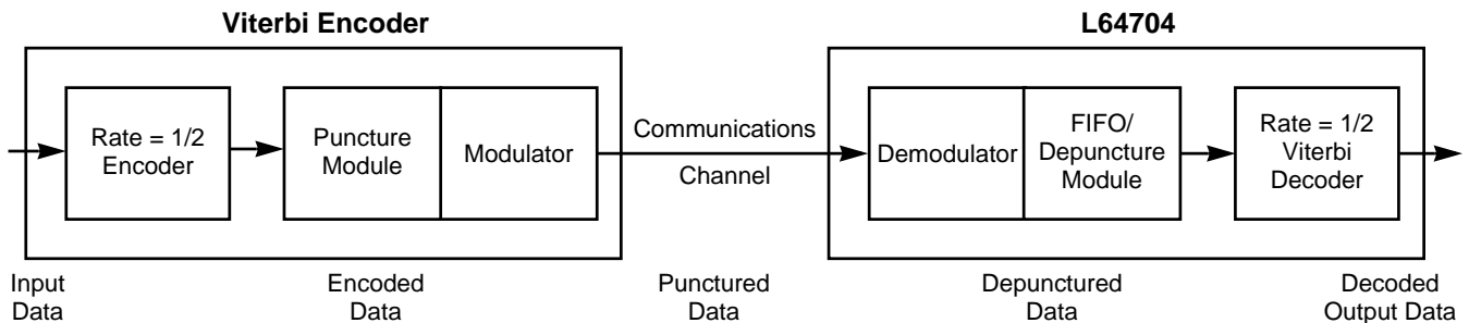
Figure 7.3 Puncturing and Depuncturing Block Diagram
