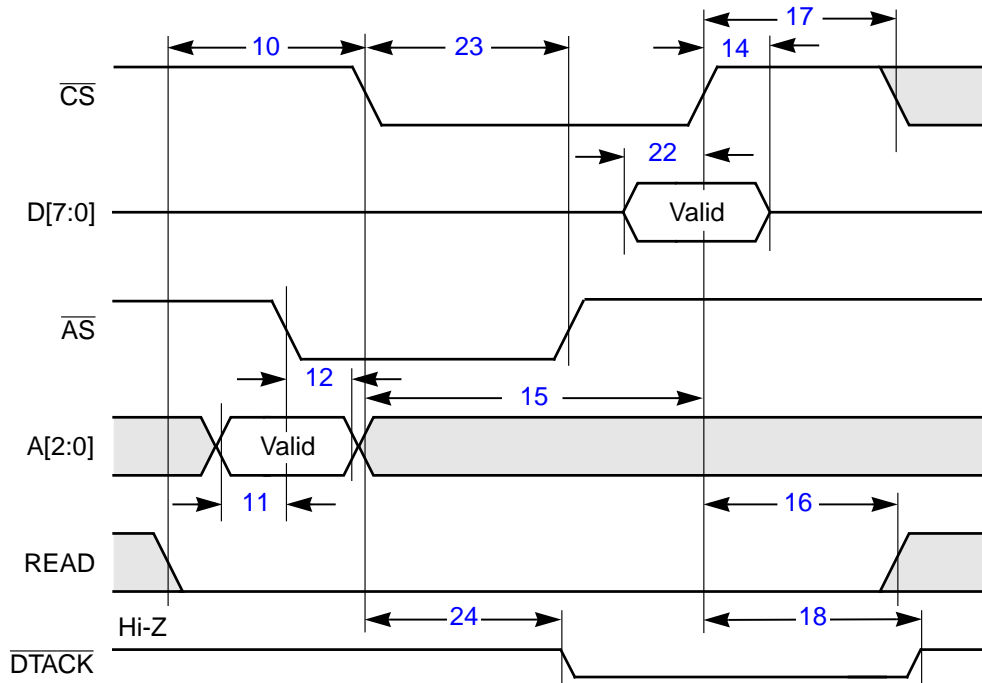
Figure 8.7 L64704 Decoder Write Cycle
