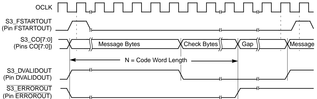
Figure 4.13 Synchronization Stage 3 Output Waveforms
