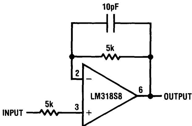
Voltage Follower
