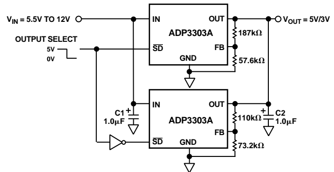
Figure 23. Crossover Switch
