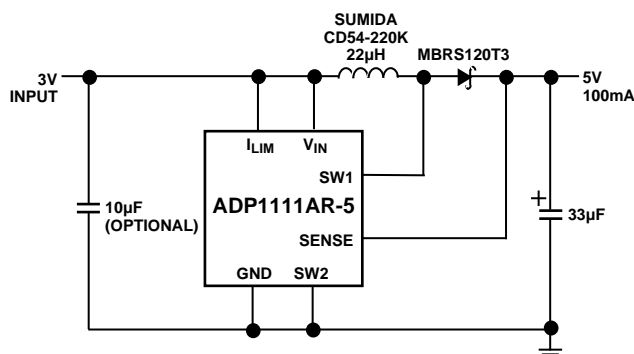
Figure 1. 3 V to 5 V Step-Up Converter
