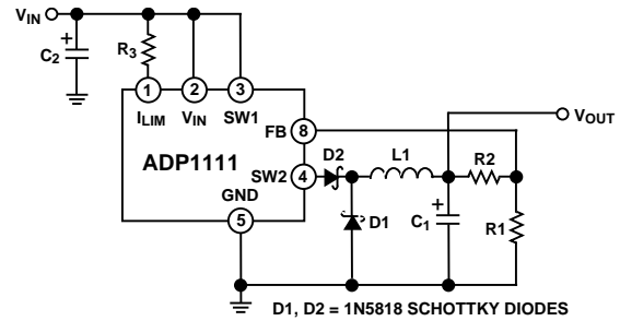
Figure 20. Step-Down Model, V_{OUT} > 6.2 V
