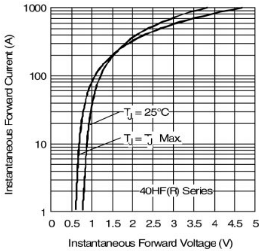
Fig. 11 - Forward Voltage Drop Characteristics
