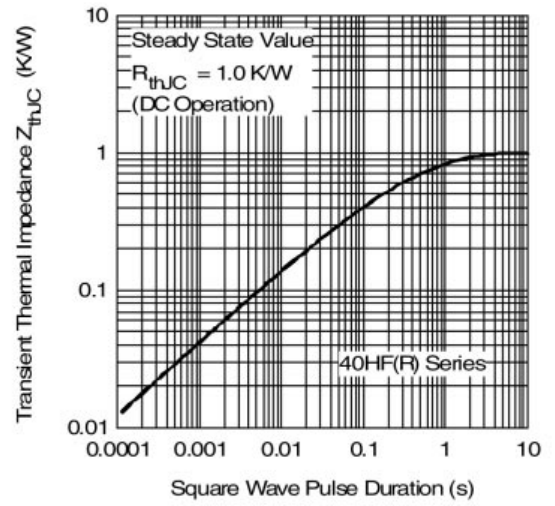
Fig. 12 - Thermal Impedance Z_{thJC} Characteristics
