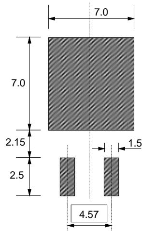
Fig.13. SOT428 : minimum pad sizes for surface mounting.
