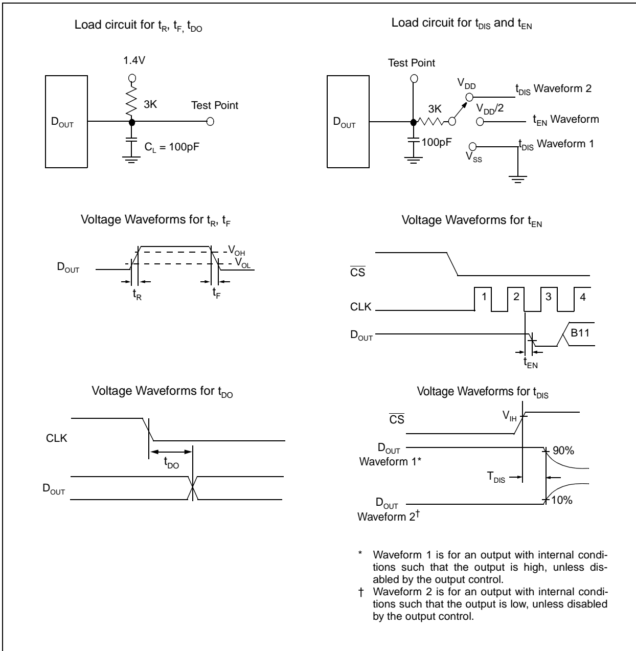
FIGURE 1-2: Test Circuits.
