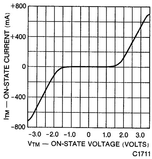
Fig. 1 On-State Characteristics
