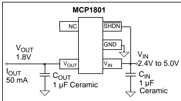
FIGURE 6-1: Typical Application Circuit.
