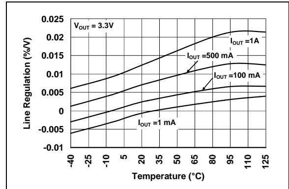
FIGURE 2-16: Line Regulation vs. Temperature (3.3V Fixed).
