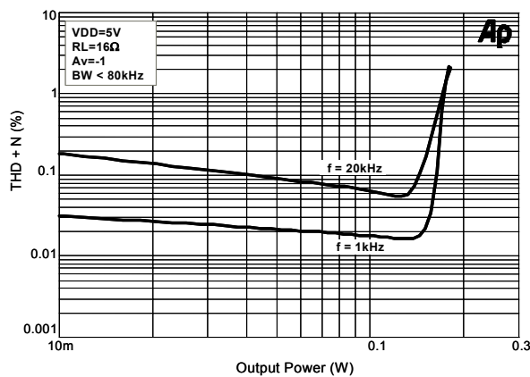
Figure 2. THD+N vs. Output Power
