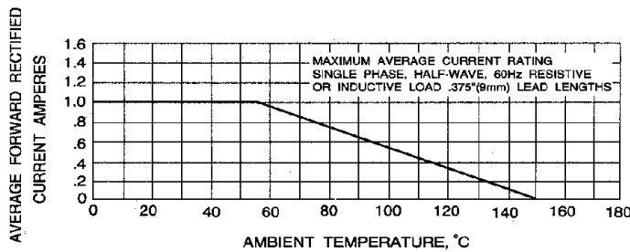
Fig. 3 - MAXIMUM AVERAGE FORWARD CURRENT RATING
