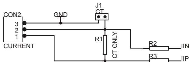
Figure 4: Current sensing using a CT
