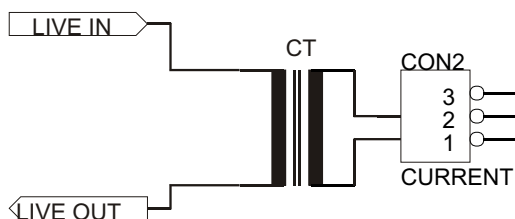
Figure 5: Current connection diagram for CT
