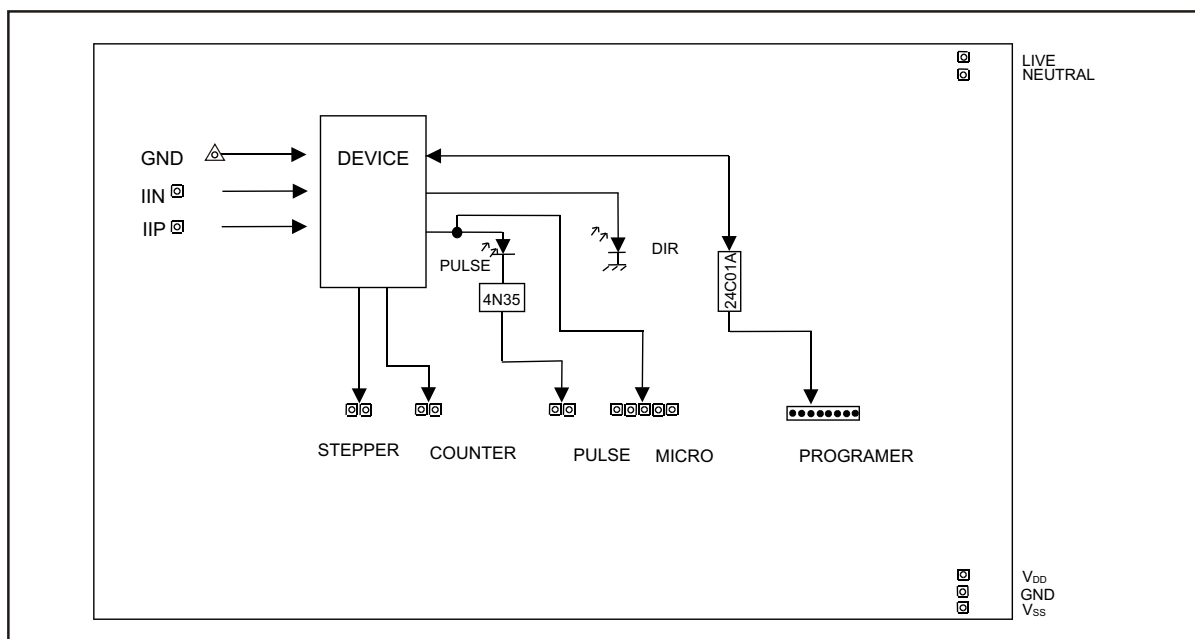
Figure 1: Functional Diagram
