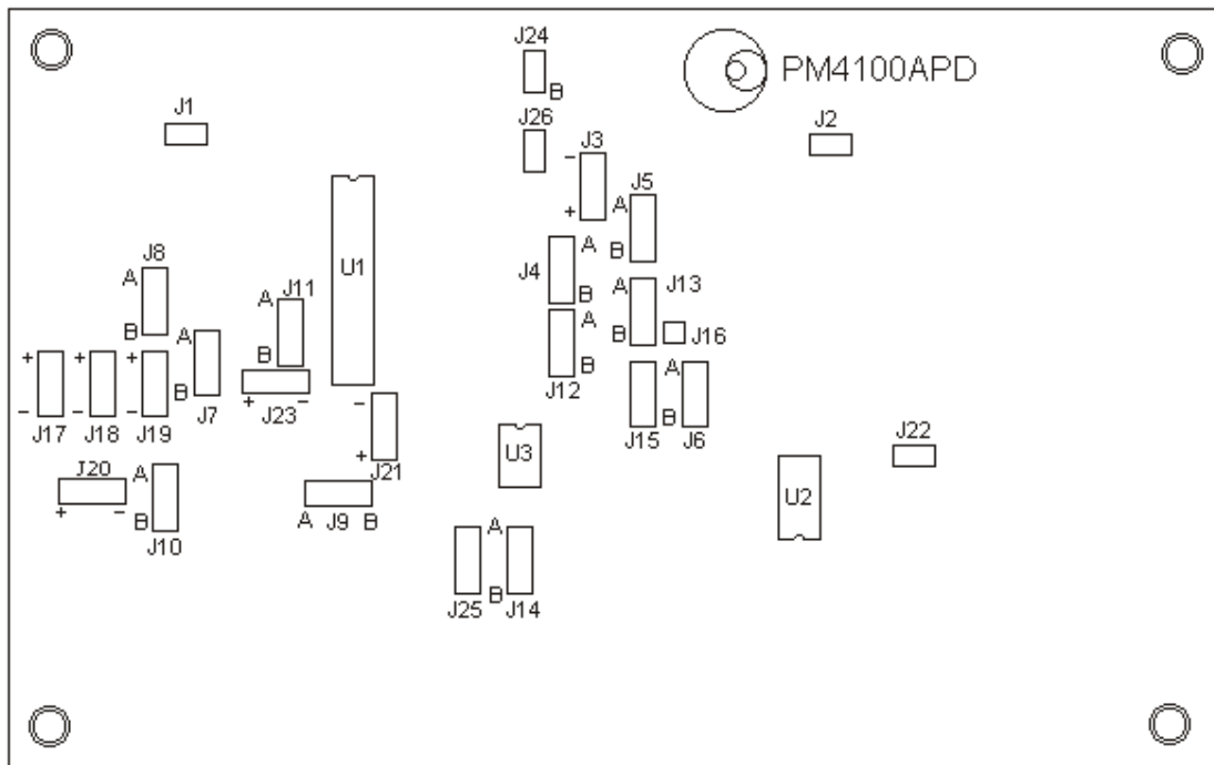
Figure 9: Jumper positions
