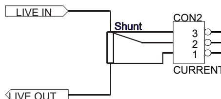
Figure 6: Current connection diagram for Shunt
