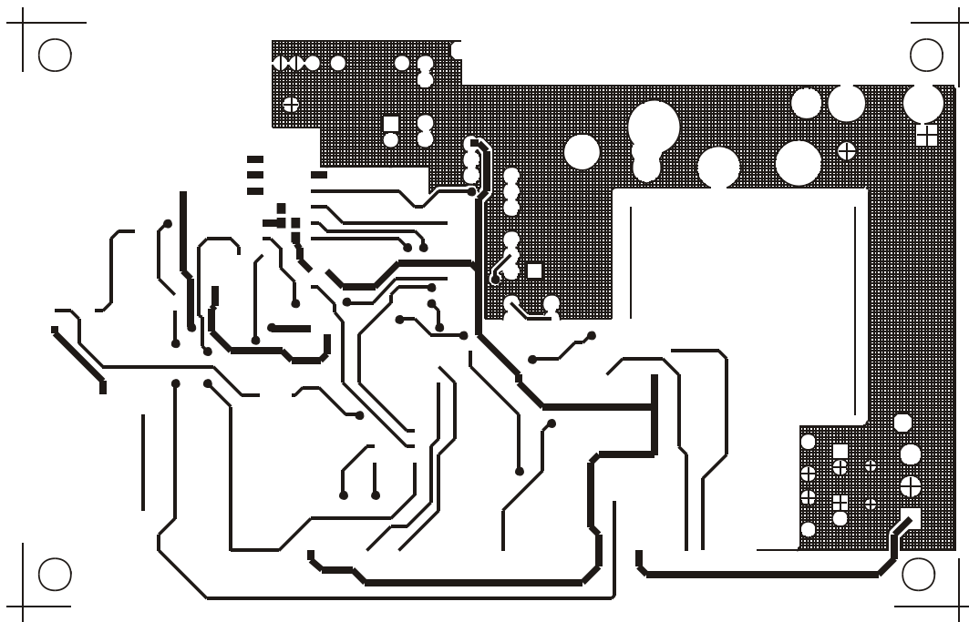
Figure 14: Bottom PCB Layout
