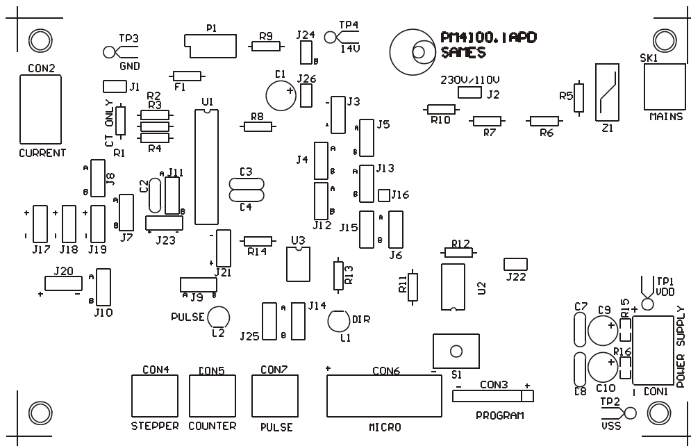
Figure 11: Top Silkscreen
