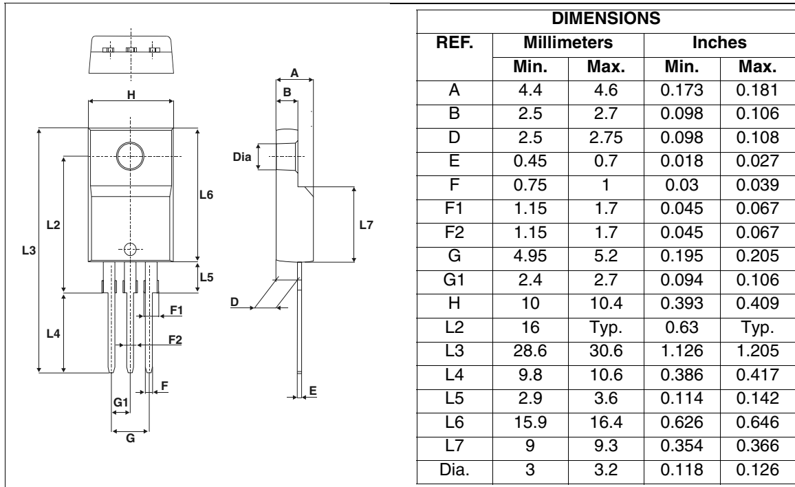
Figure 10: TO-220FPAB Package Mechanical Data
