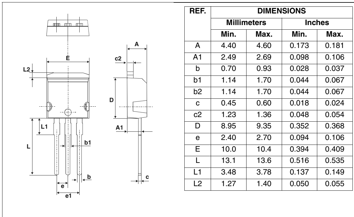
Figure 11: I 2 PAK Package Mechanical Data
