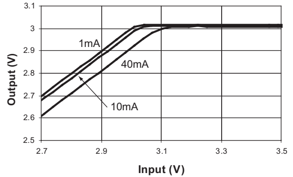
Output Voltage v. Input Voltage
