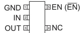
AAT3222 SOT23-5 (Top View)
