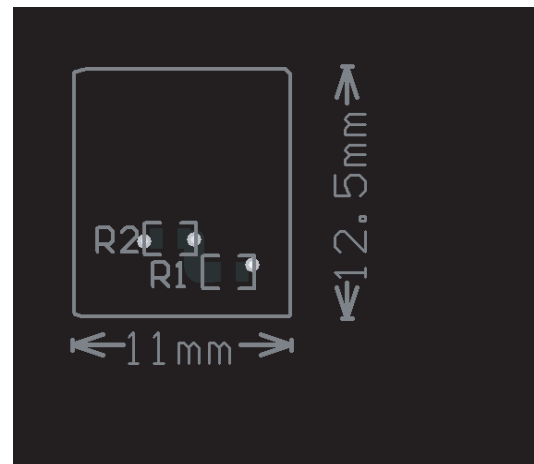
Figure 3. AAT1217 Evaluation Board Layout Example Bottom Layer
