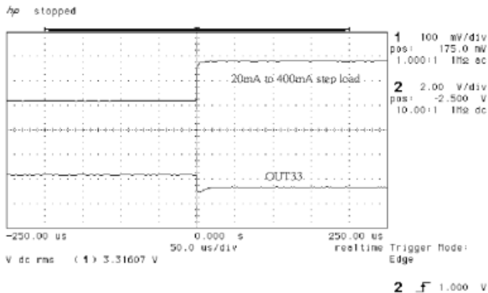
Figure 9. 3.3V Load Transient Response Rising
