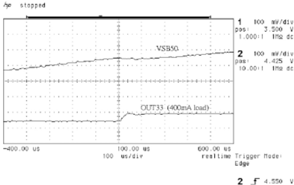
Figure 5. 3.3V VSB50 Power Up(AUX33=3.3V)
