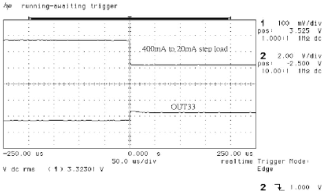
Figure 8. 3.3V Load Transient Response Falling.
