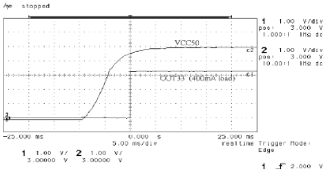
Figure 1. 3.3V VCC50 Cold Start
