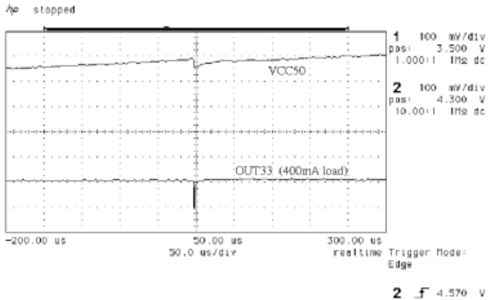
Figure 3. 3.3V VCC50 Power Up(VSB50=5V)
