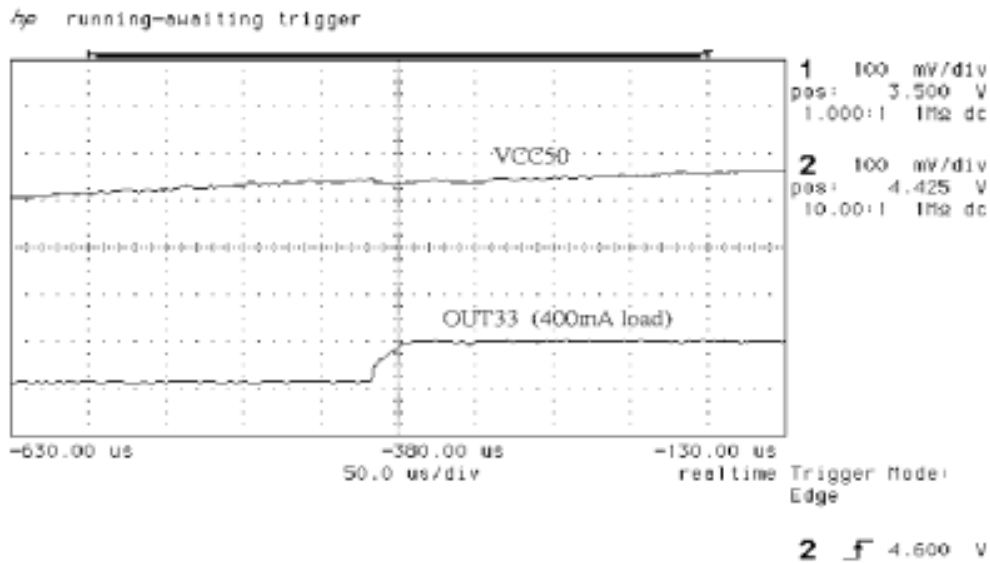
Figure 4. 3.3V VCC50 Power Up(AUX33=3.3V)
