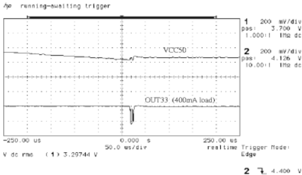
Figure 6. 3.3V VCC50 Power Down(VSB=5V)
