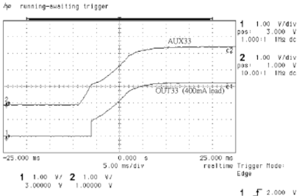
Figure 2. 3.3V AUX33 Cold Start
