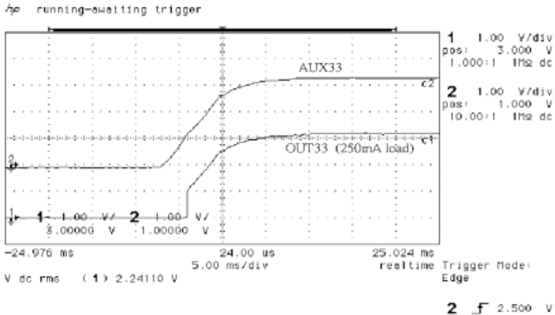
Figure 3. 3.3V AXX33 Cold Start
