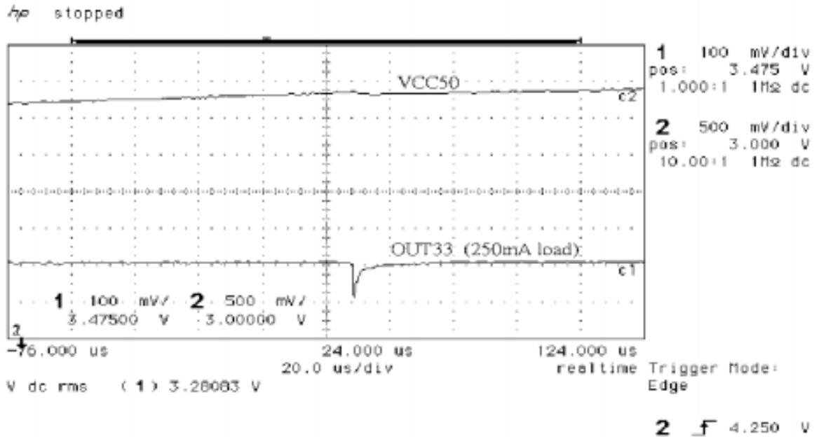
Figure 5. 3.3V VCC50 Power Up(VSB50=5V)
