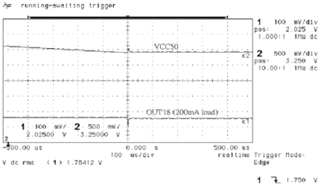
Figure 13. 3.3V VCC50 Power Down(AUX33=3.3V)
