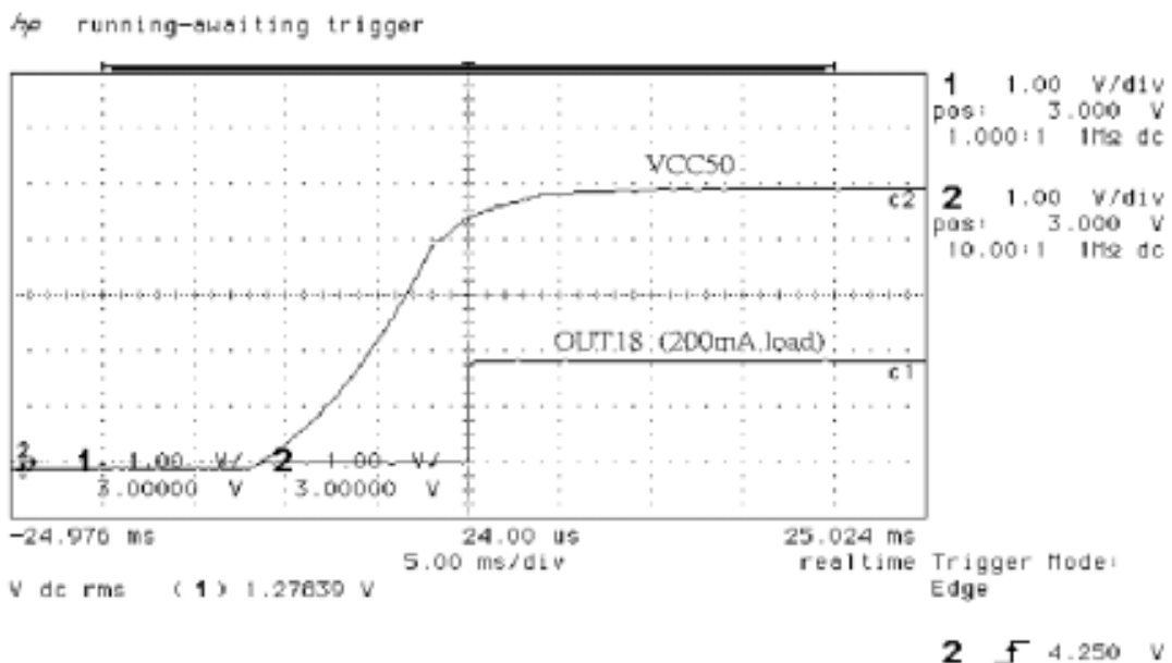
Figure 2. 1.8V VCC50 Cold Start
