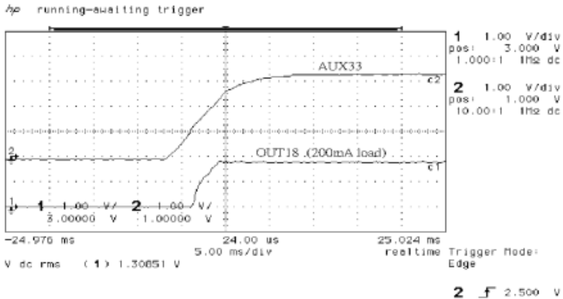
Figure 4. 1.8V AXX33 Cold Start
