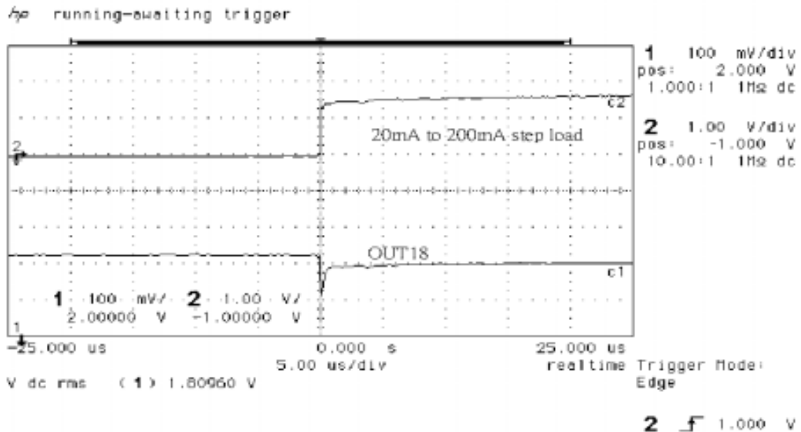
Figure 18. 1.8V Load Transient Response Rising
