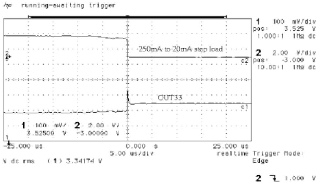
Figure 15. 3.3V Load Transient Response Falling.
