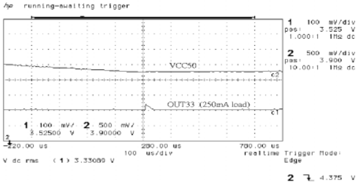
Figure 11. 3.3V VCC50 Power Down(VSB=5V)
