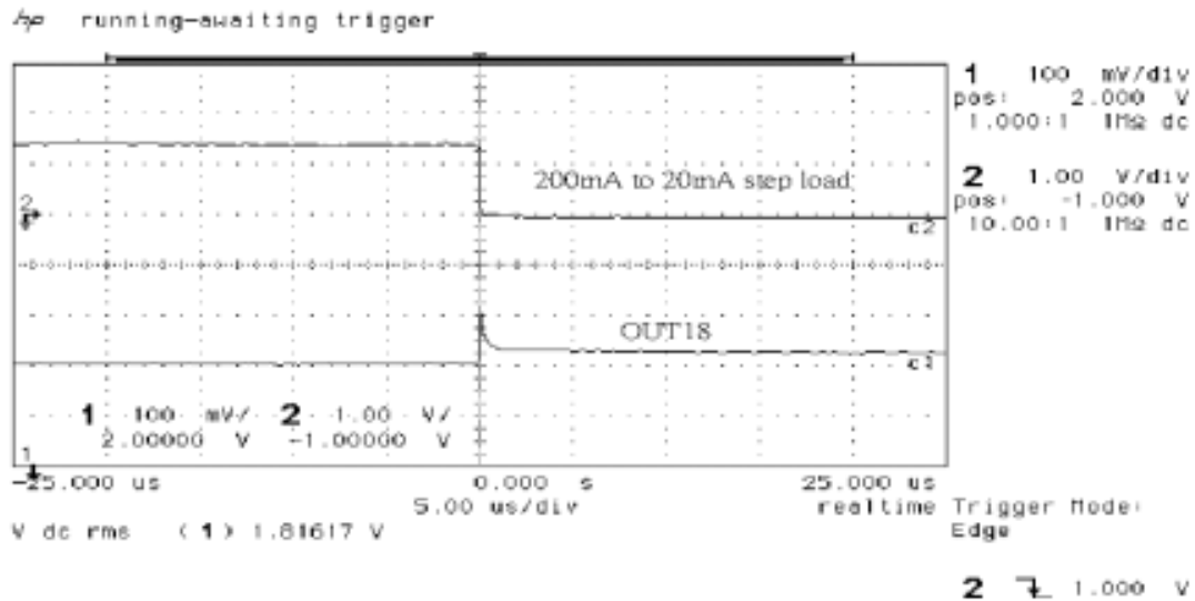
Figure 16. 1.8V Load Transient Response Falling.
