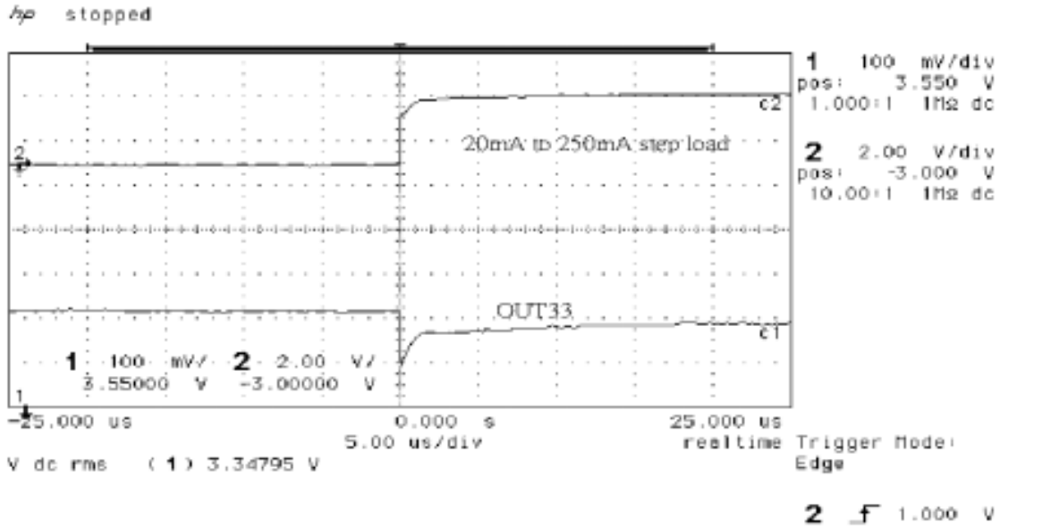
Figure 17. 3.3V Load Transient Response Rising
