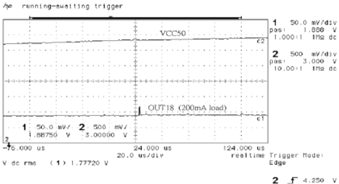
Figure 6. 1.8V VCC50 Power Up(VSB50=5V)
