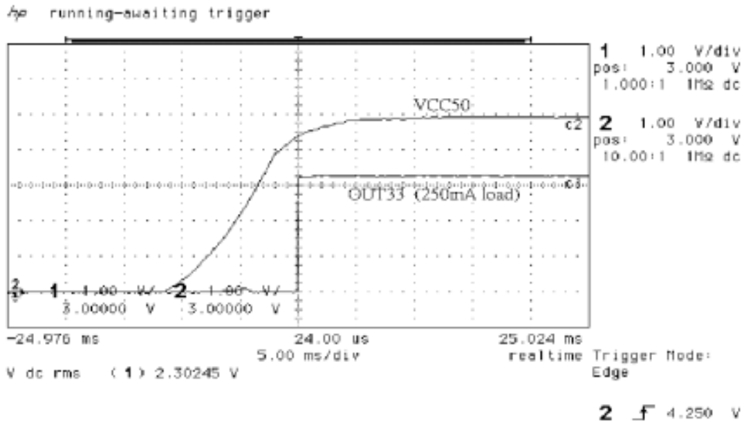
Figure 1. 3.3V VCC50 Cold Start
