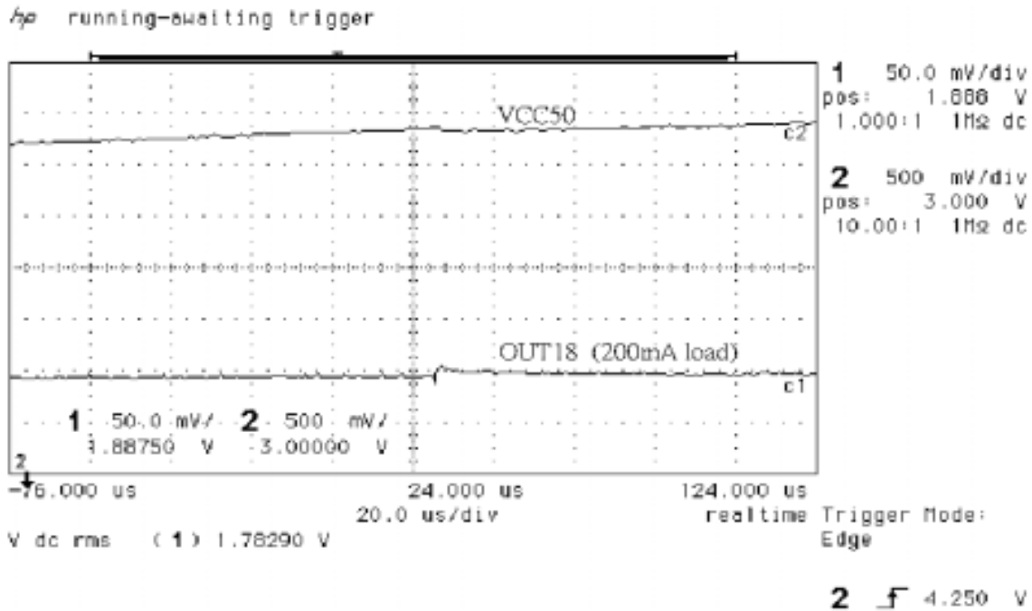
Figure 8. 1.8V VCC50 Power Up(AUX33=3.3V)
