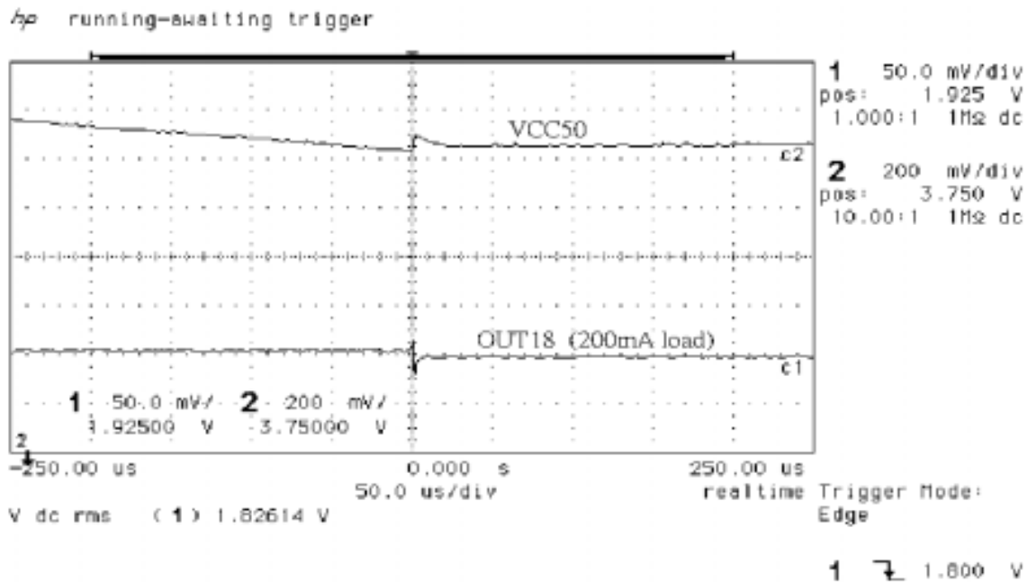
Figure 12. 1.8V VCC50 Power Down(VSB=5V)
