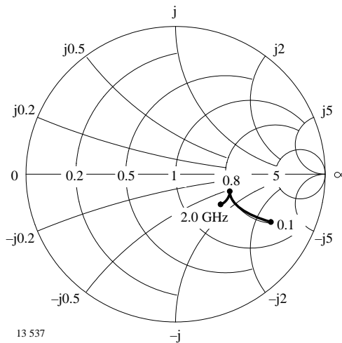
Figure 8. Output reflection coefficient
