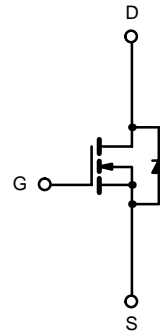
N-Channel MOSFET
