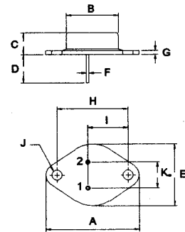
TO-66
