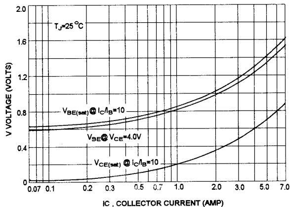
"ON" VOLTAGES
