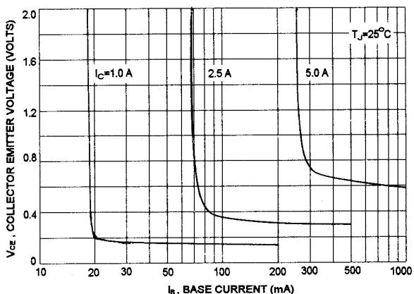
"ON" VOLTAGES
