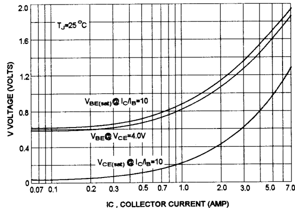
"ON" VOLTAGES
