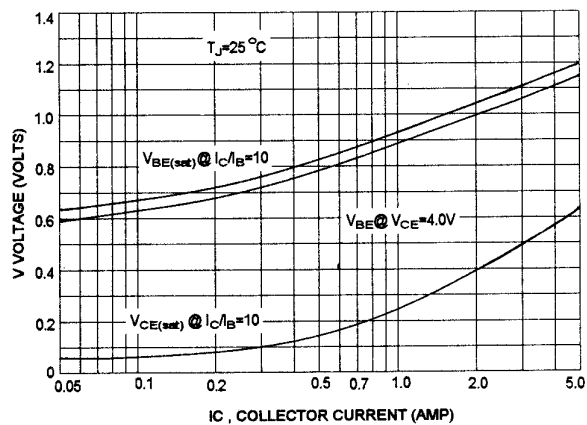
"ON" VOLTAGES
