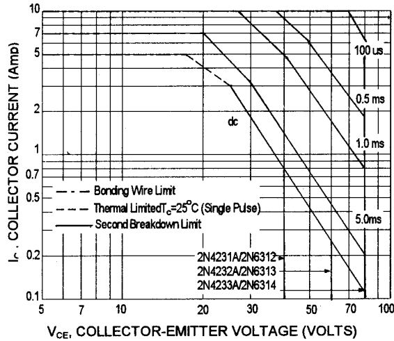
ACTIVE-REGION SAFE OPERATING AREA (SOA)
