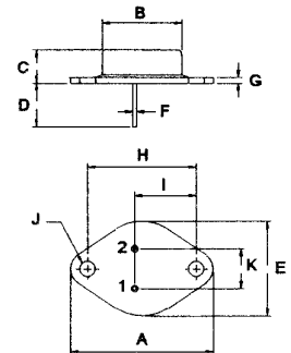
TO-66
