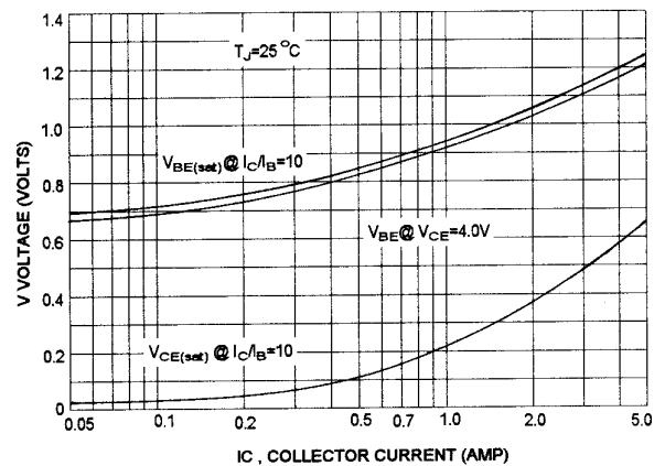
"ON" VOLTAGES
