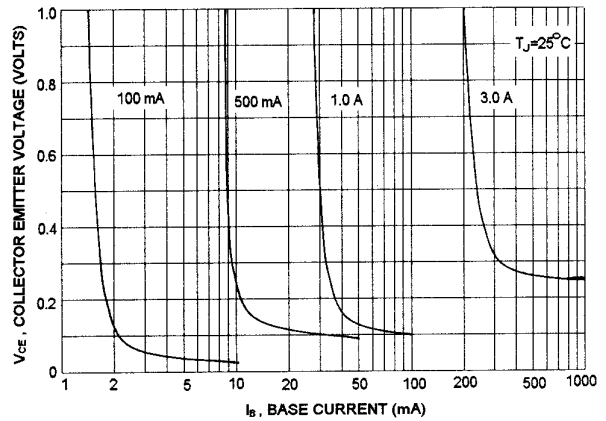
"ON" VOLTAGES
