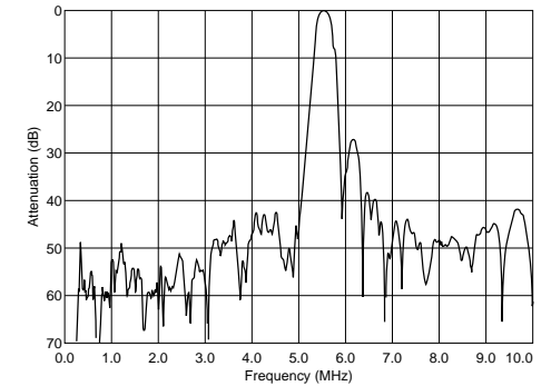
SFSRL5M50DF00-B0
