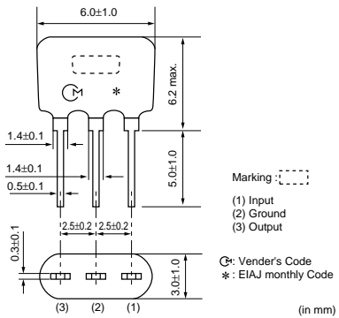
PFWLA Series
