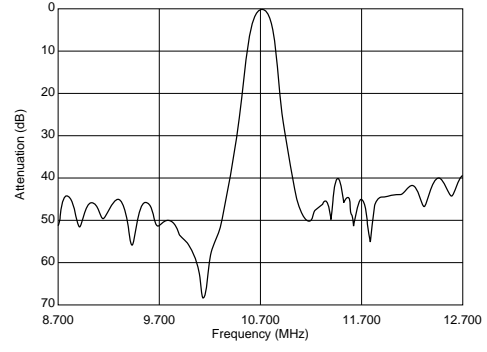
SFELA10M7HAA0-B0
