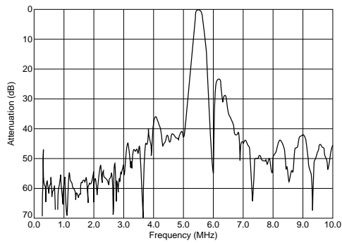
SFSRL5M50CF00-B0
