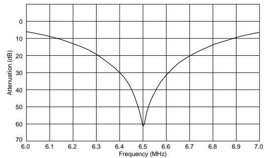
TPSRA6M50B00-B0
