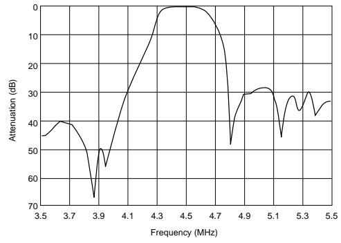
SFSRL4M50DF00-B0
