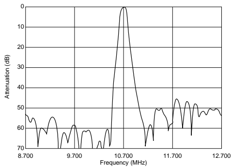
SFELB10M7KA00-B0
