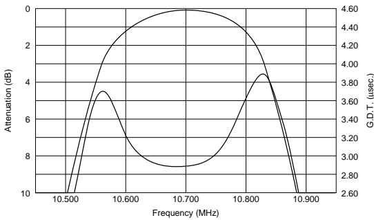
SFECS10M7FA00-R0
