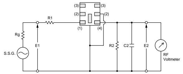
R1+Rg=R2=330\Omega\pm5\% , Rg=50\Omega C2=10pF (Including stray capacitance and input capacitance of RF Voltmeter) E1 : S.S.G. Output Voltage
