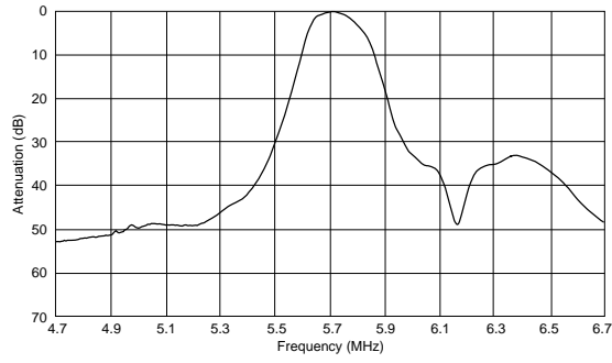
SFSRA5M74BF00-B0
