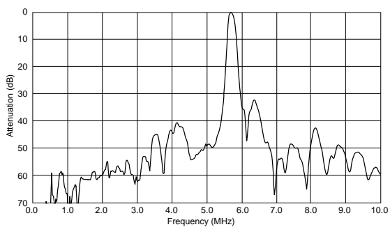
SFSRA5M74BF00-B0
