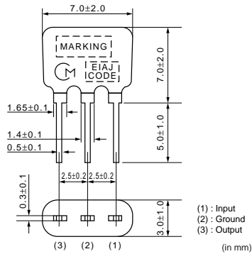
SFVLA10M7LF00-B0
