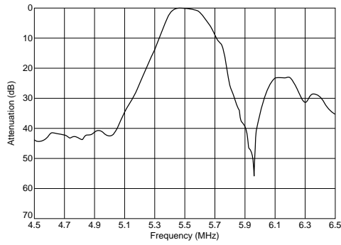
SFSRL5M50CF00-B0
