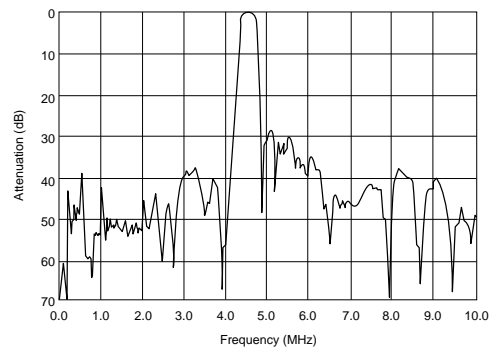
SFSRL4M50DF00-B0
