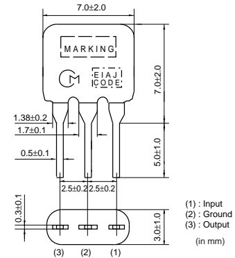
SFELA10M7EA00-B0
