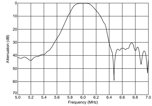
SFSRL6M00DF00-B0
