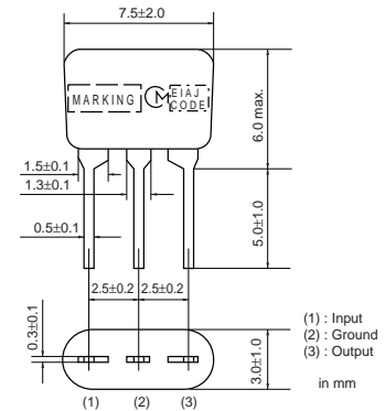
SFELB10M7HA00-B0
