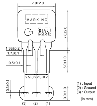
SFELA10M7DF00-B0
