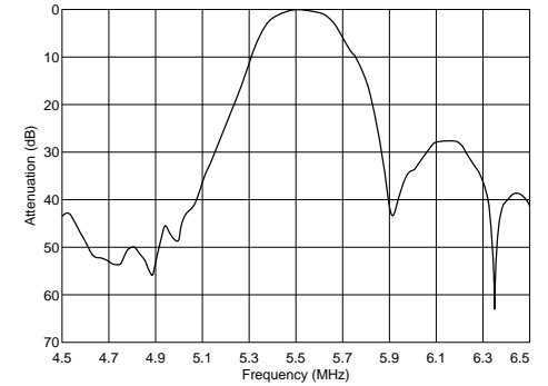
SFSRL5M50DF00-B0
