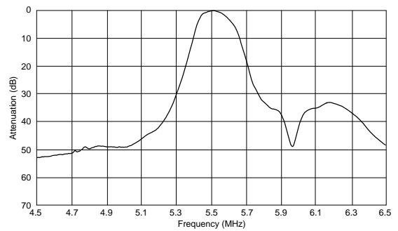
SFSRA5M50BF00-B0
