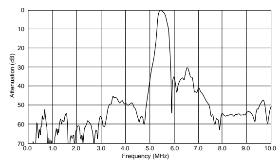
SFSRA5M50DF00-B0
