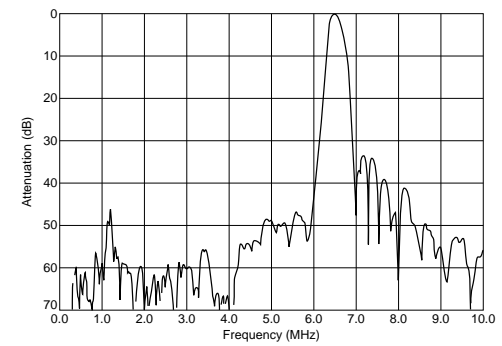
SFSRL6M50DF00-B0
