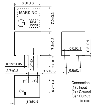
CFULA Series
