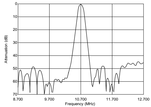
SFELB10M7JA00-B0
