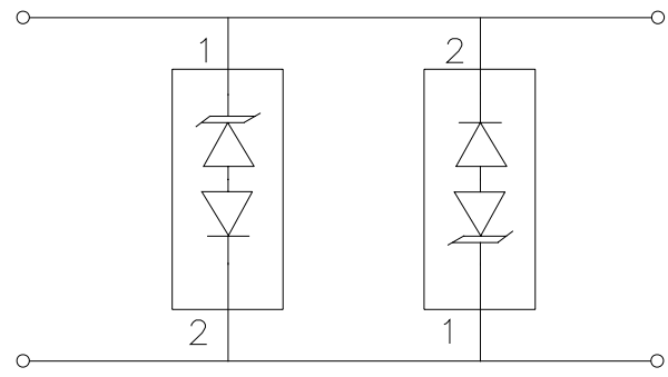
Two Devices : Bidirectional or Unidirectional Line
