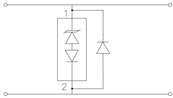
One Devices with Steering Diode : Unidirectional Line Only
