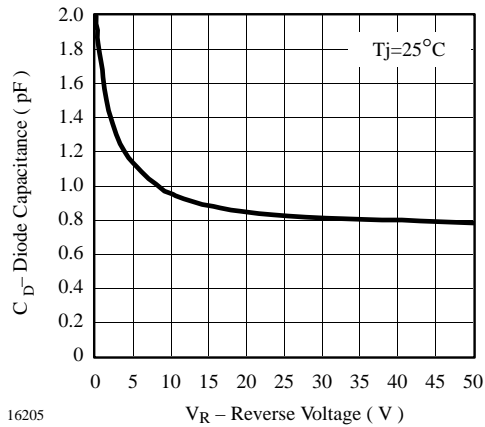
Figure 2. Diode Capacitance vs. Reverse Voltage
