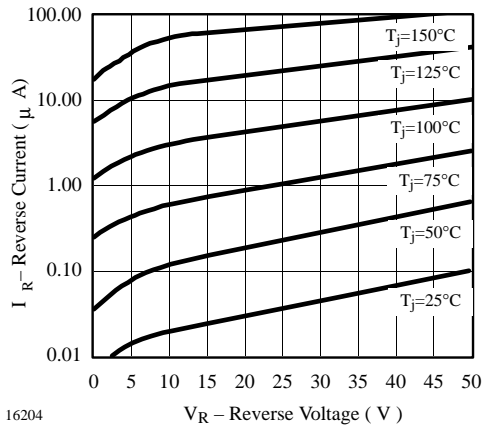
Figure 1. Reverse Current vs. Reverse Voltage
