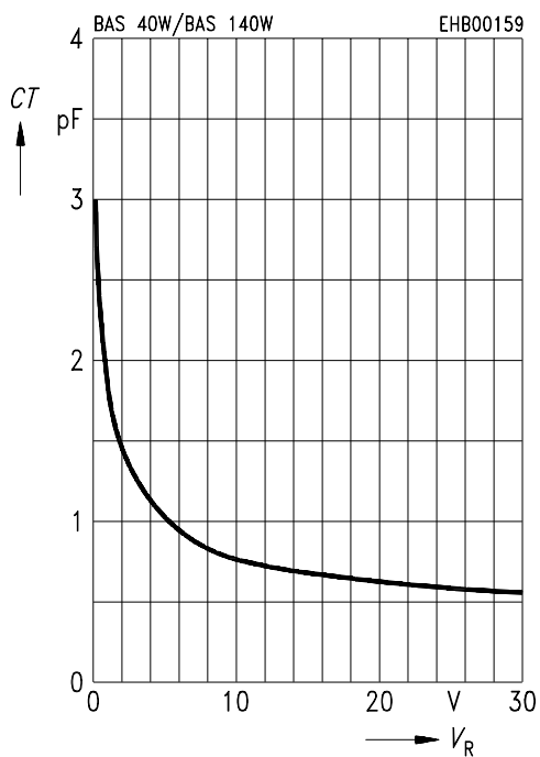
Diode capacitance C_T = f(V_R)
