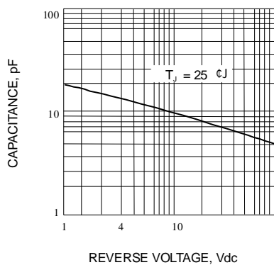
Fig. 4-TYPICAL JUNCTION CAPACITANCE
