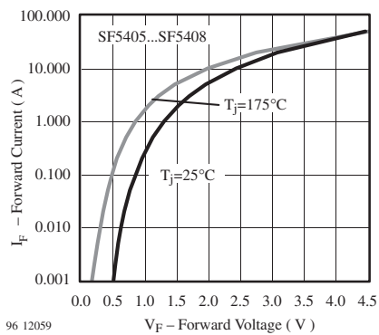
Figure 7. Max. Forward Current vs. Forward Voltage
