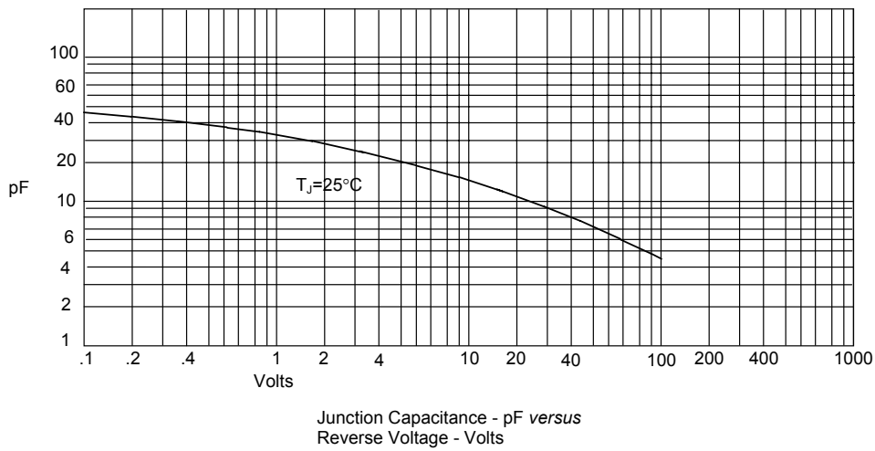
Figure 3 Junction Capacitance
