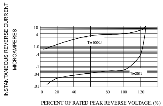
Fig. 5-TYPICAL REVERSE CHARACTERISTICS
