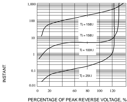
Fig. 4-TYPICAL REVERSE CHARACTERISTICS
