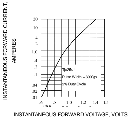
Fig. 2-TYPICAL FORWARD CHARACTERISTICS
