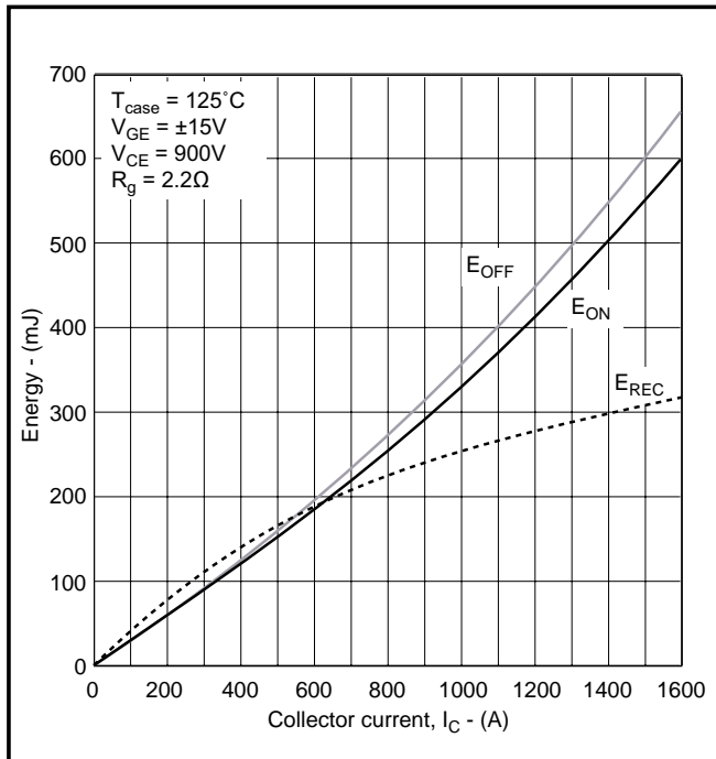
Fig. 5 Typical switching energy vs collector current
