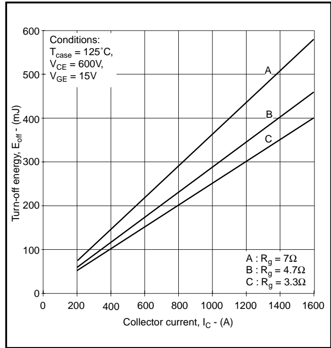
Fig.10 Typical turn-off energy vs collector current
