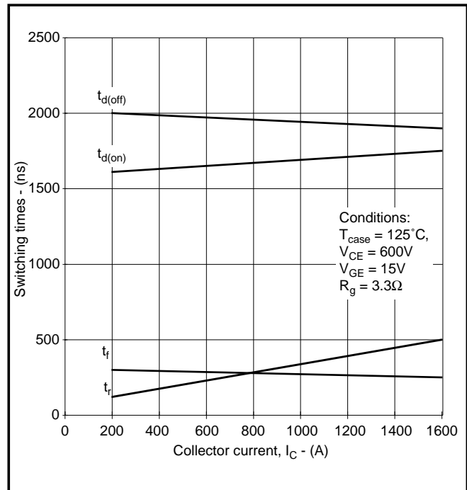
Fig.12 Typical switching times
