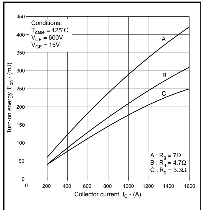
Fig.8 Typical turn-on energy vs collector current
