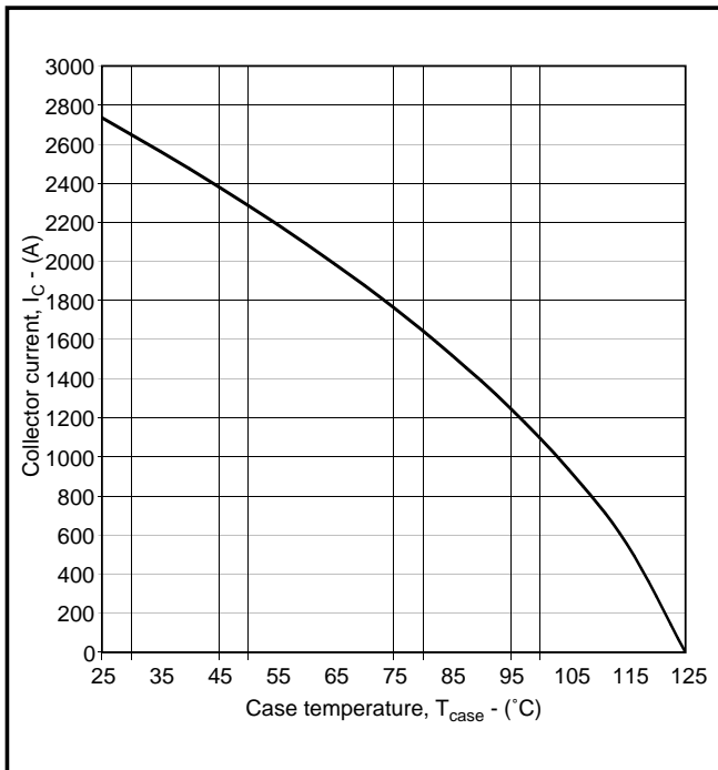
Fig.17 DC current rating vs case temperature
