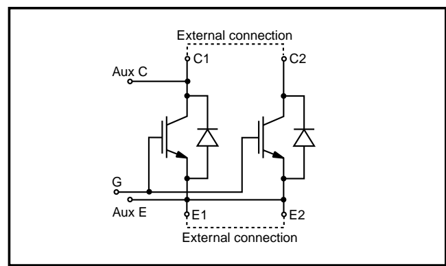
Fig.1 Single switch circuit diagram
