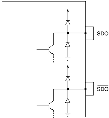
Fig. 6 Static Protection Diodes
