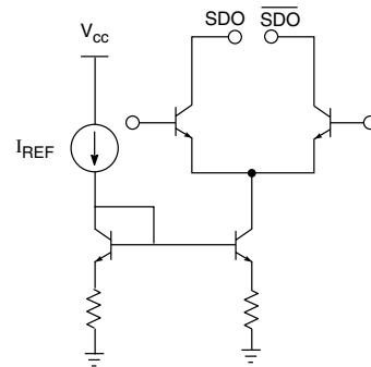
Fig. 2 Differential Output Stage (SDO/ \overline{\text{SDO}} ) I_{\text{REF}} derived using R_{\text{SET}}
