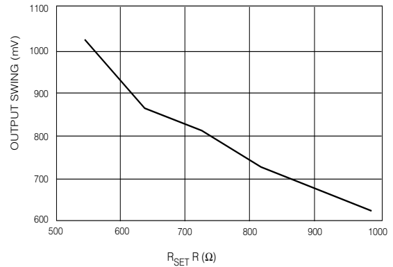
Fig. 7 Output Amplitude Adjustment
