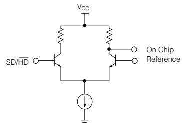
Fig. 3 Slew Rate Select Input Stage (SD/ \overline{\text{HD}} )
