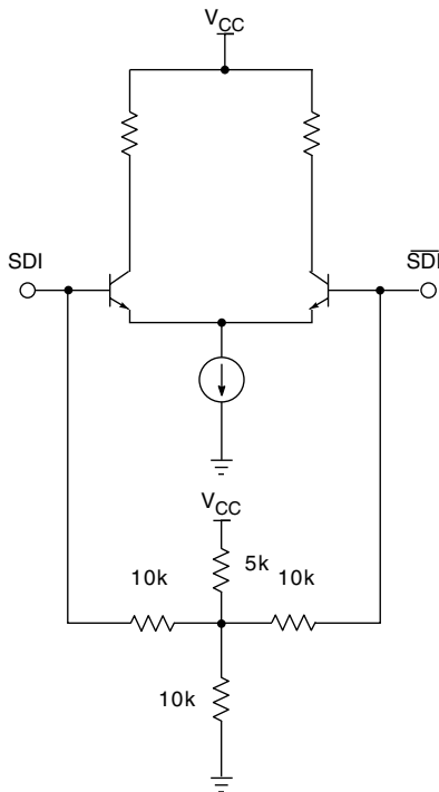
Fig. 1 Differential Input Stage (SDI/ \overline{\text{SDI}} )
