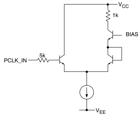
Fig. 11 PCLK_IN Circuit
