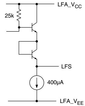
Fig. 5 LFS Output Circuit
