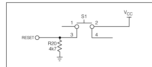
GS1522 RESET CIRCUIT
