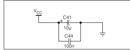
POWER CONNECT
