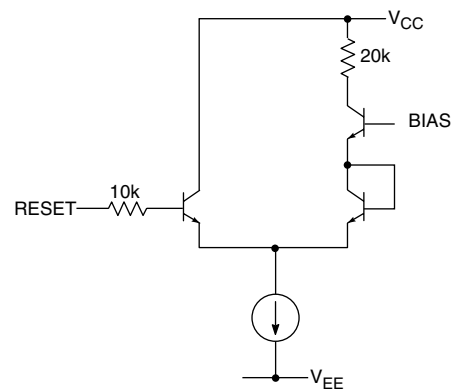
Fig. 12 RESET Circuit
