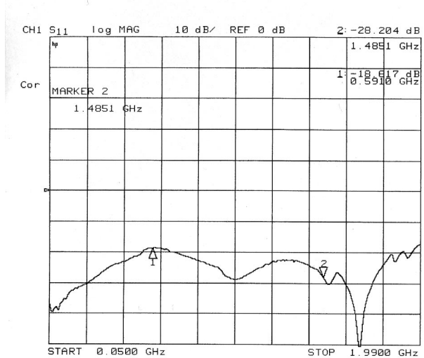
Fig. 26 Compensated Output Return Loss at Logic HIGH
