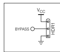
GS1522 SCRAMBLER BYPASS
