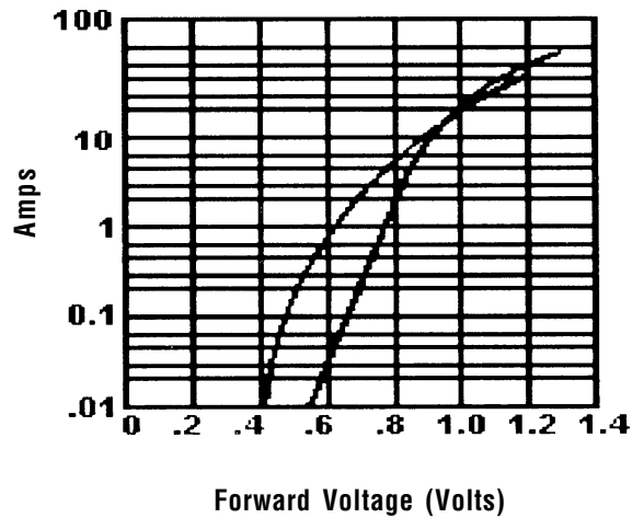
Instantaneous Forward Characteristics
