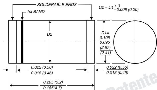
DO-213AB
